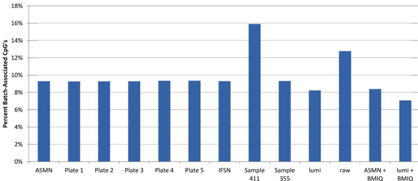
Figure 8. Percent of 450K array CpG sites associated with chip batch ( p < 0.01 ) shown by normalization method.
