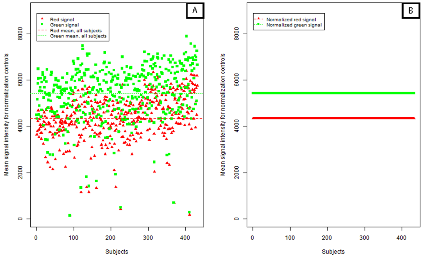
Figure 4. Mean control probe color signal intensity before and after normalization.
