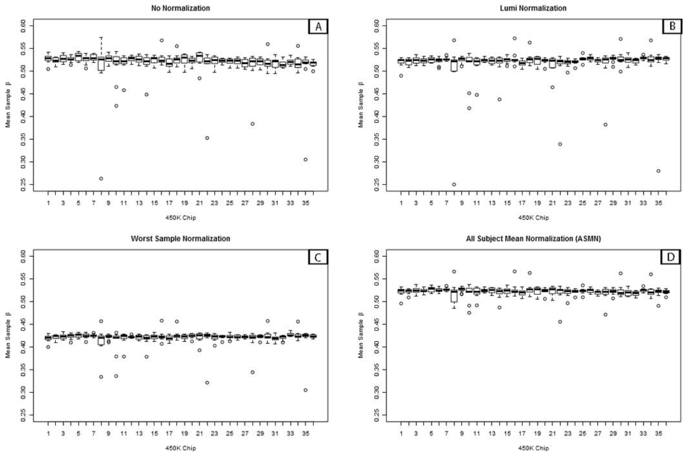
Figure 7. Box plots of sample mean methylation by normalization methods.
