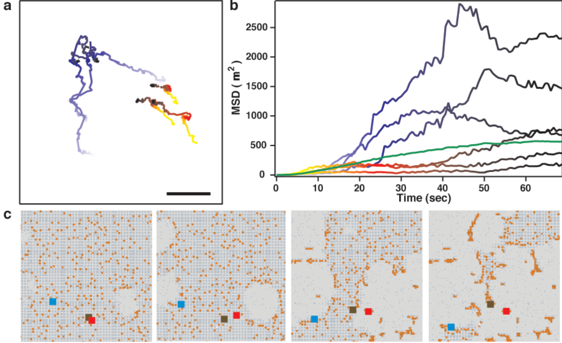
Figure 4: Individual NPs motion in liquid phase TEM observation and lattice gas modeling. (a) Trajectories of selected individual NPs from Fig. 1b for a time step of \delta t = \frac{1}{3} sec. The time variable is labeled with blue and orange color scale for different types of trajectories. Black color indicates final stage of movement. The scale bar is 20 nm. (b) MSD of individual NPs shown in panel (a) with the same color scale along with the average MSD of the selected 51 NPs (green line). (c) Trajectories from lattice gas simulations. Selected NPs are enlarged and colored with red, brown, and blue to signify their motion. Time increases from left to right, for times (in MC steps) 1000, 1200, 1400, and 1600, respectively. Parameters are identical to those in Fig. 1 for a coverage of \rho = 10\% , chemical potential \mu = -3\frac{1}{8}\varepsilon_\ell , and temperature T = 2\varepsilon_\ell . Image size corresponds to approximately 50 \times 50 \text{ nm}^2 .
