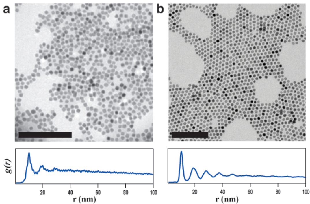
Figure S3: TEM images and radial-distribution functions of NPs assemblies formed under electron beam irradiation (panels (a)) and drop casting (panels (b)) on SiNx TEM grid. The scale bar is 100 nm.
