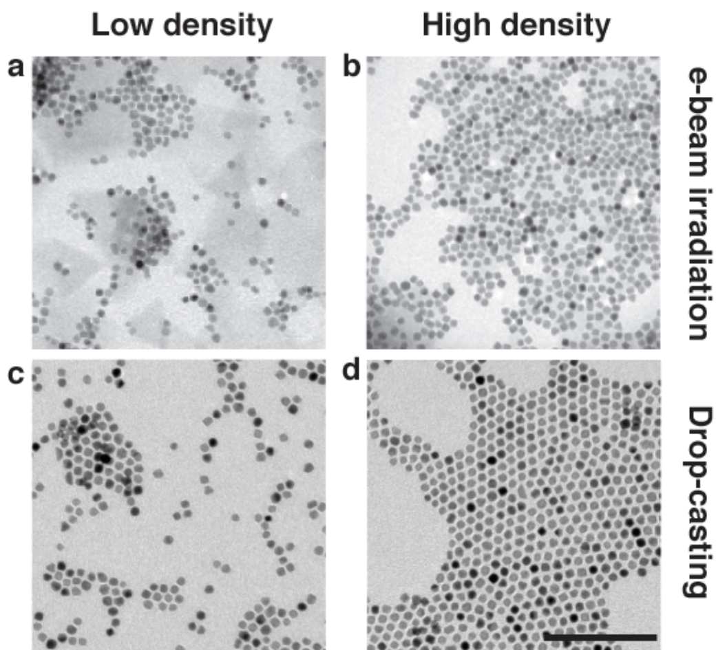
Figure 3: TEM images of NPs assembly formed under electron beam irradiation (panels (a) and (b)) and drop casting (panels (c) and (d)) on SiNx TEM grid. The scale bar is 100 nm.
