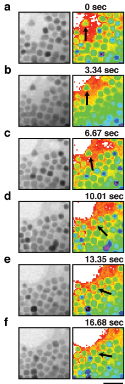
Figure 5: NP addition onto domain of superlattice. (a) – (f) Snapshots from Movie 3 at different times (left frames) and a corresponding color map with rainbow color scale (right frames). Contrast of rainbow color was calibrated such that white color corresponds to dried area. Arrow indicates a NP that moves laterally and rotates until it adequately fills in a vacancy in domain. The scale bar is 25 nm.
