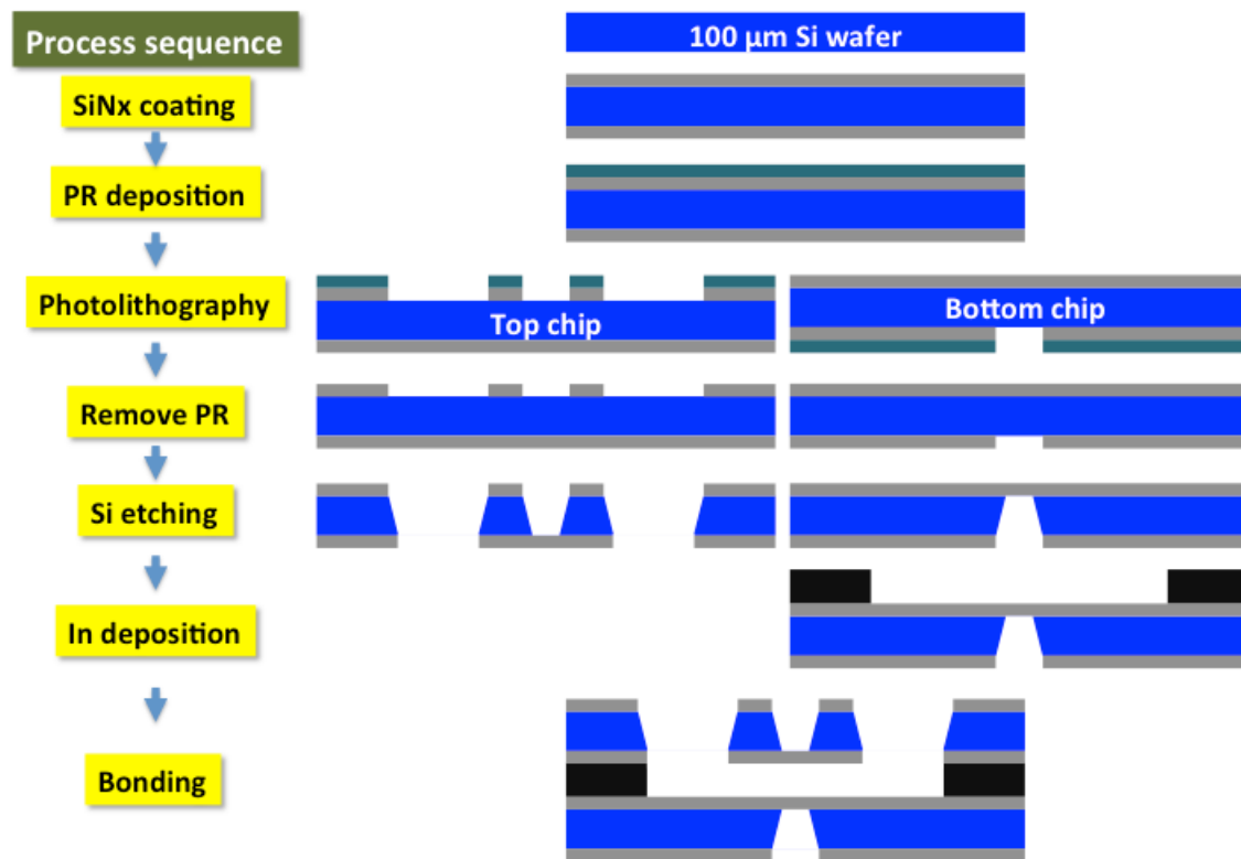
Figure S1: Fabrication process of liquid TEM cell.
