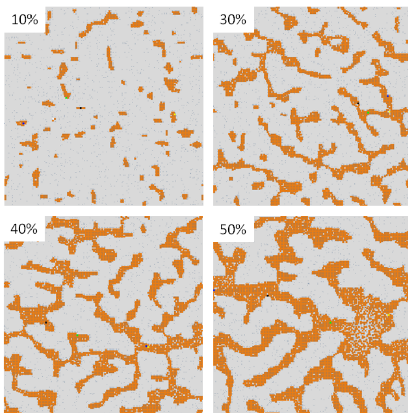
Figure S6: Simulated superlattice patterns with varying coverage of NPs under low NP diffusivity. Parameters are the same as in Fig. 4S.
