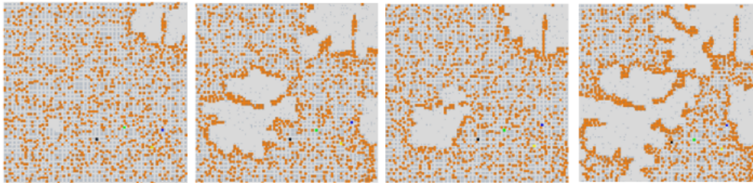
Figure S5: Simulated trajectories showing how NPs are dragged by the solvent front (upper right corner in each image). Time frame from left to right are 900, 1300, 1700, and 2100 in MC steps, respectively. Parameters are identical to those in Fig. 1 with \mu = -3\frac{1}{4}\varepsilon_\ell and T = 2\varepsilon_\ell .
