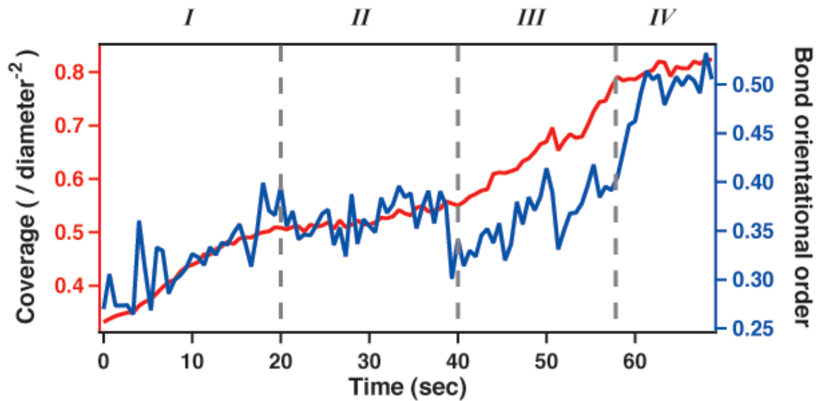
Figure 2: Surface coverage of NPs and the 2D bond orientational order parameter, a measure of crystalline ordering, as a function of time. Results are shown for the same trajectory of Fig. 1b.
