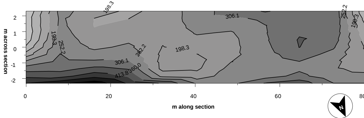
Figure 3.21: Distribution of aggregate base moduli along pavement section.
