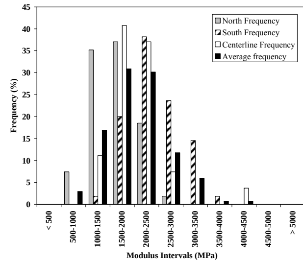
Figure 3.16: Relative frequency of asphalt concrete modulus.
