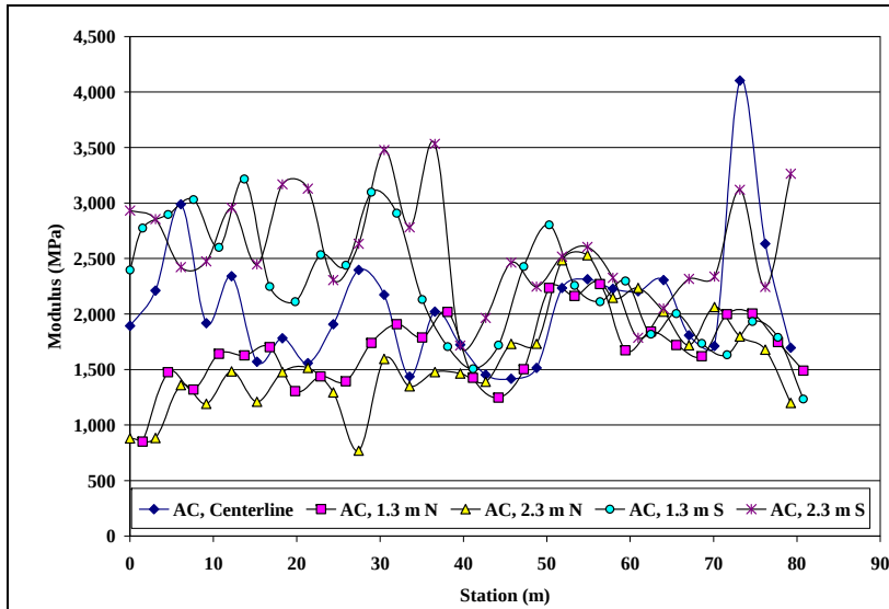
Figure 3.13: Back-calculated modulus of asphalt concrete (tested on AC).
