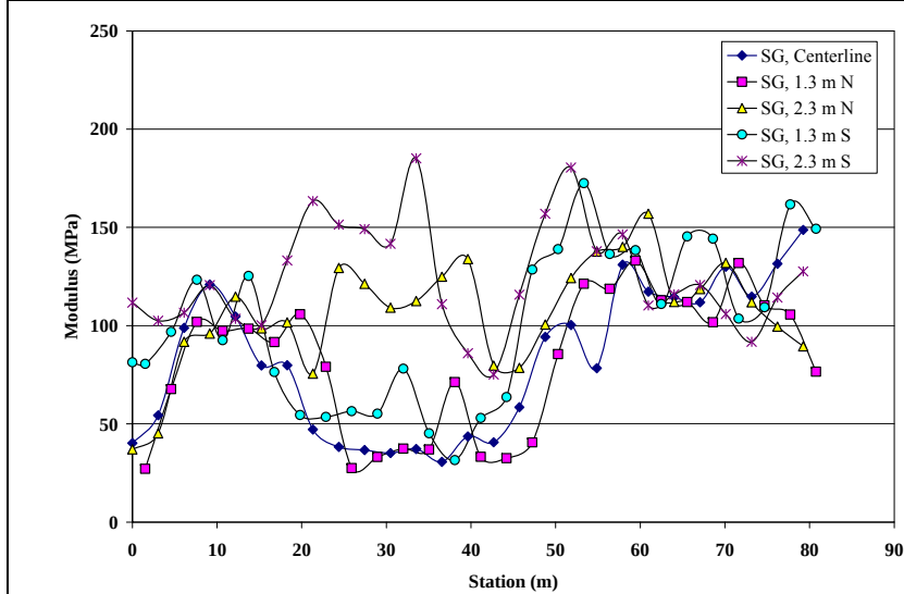
Figure 3.15: Back-calculated modulus of subgrade (tested on AC).
