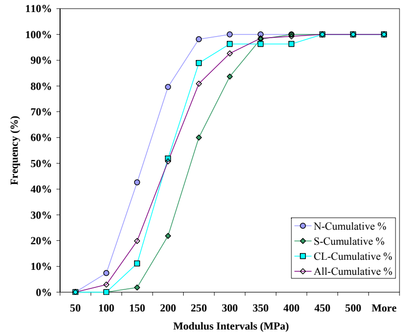
Figure 3.20: Cumulative histogram of base layer modulus.
