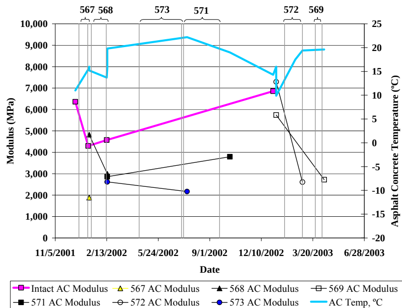
Figure 4.5: Backcalculated asphalt concrete moduli for HVS sections.
