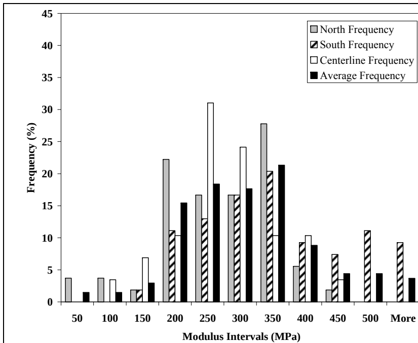
Figure 3.19: Relative frequency of base layer modulus.
