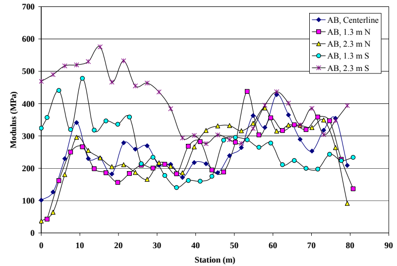
Figure 3.14: Back-calculated modulus of aggregate base (tested on AC).
