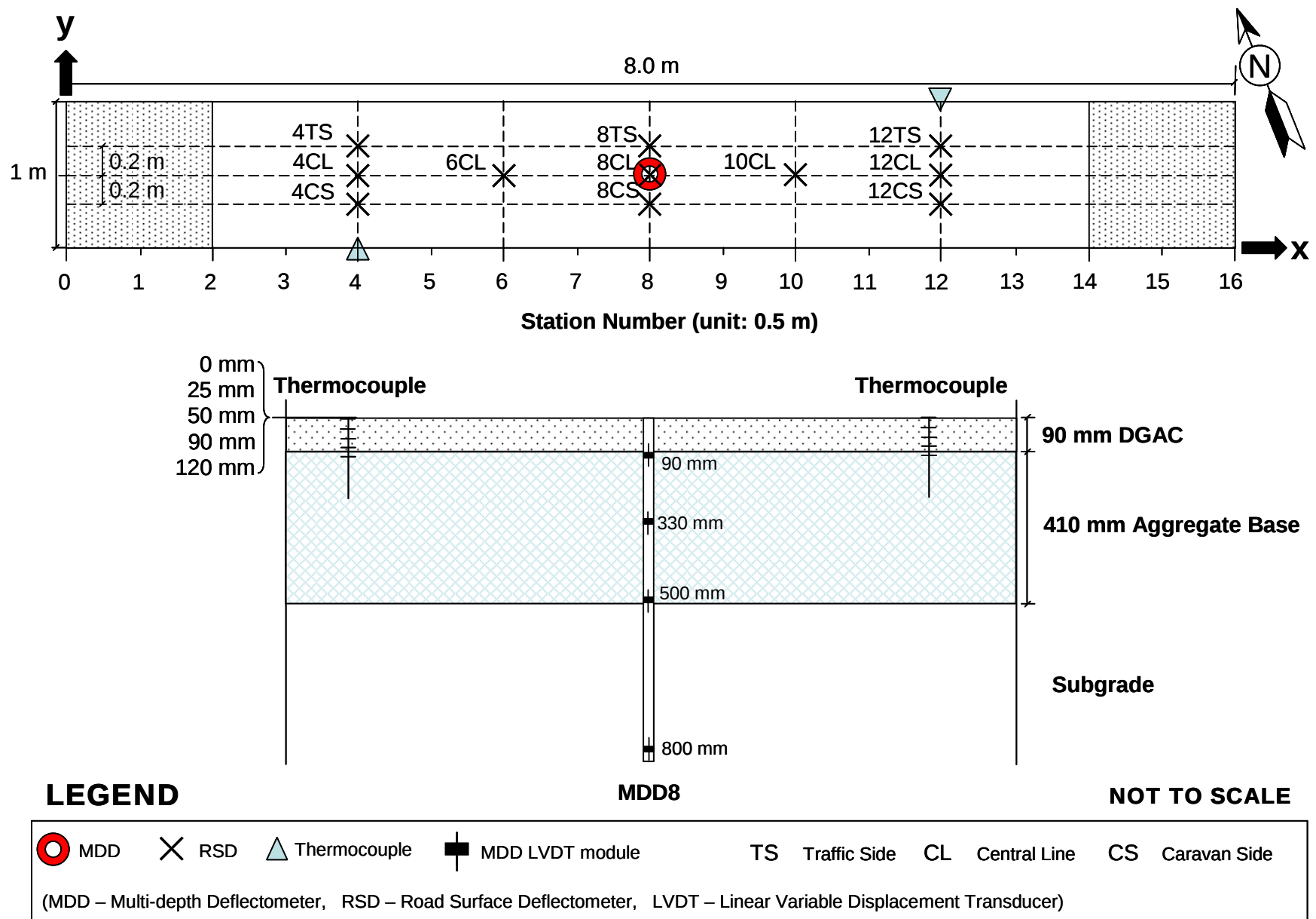
Figure 4.1: Test section layout and location of instruments.
