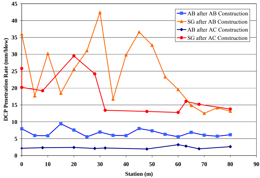
Figure 3.7: DCP data for unbound materials.
