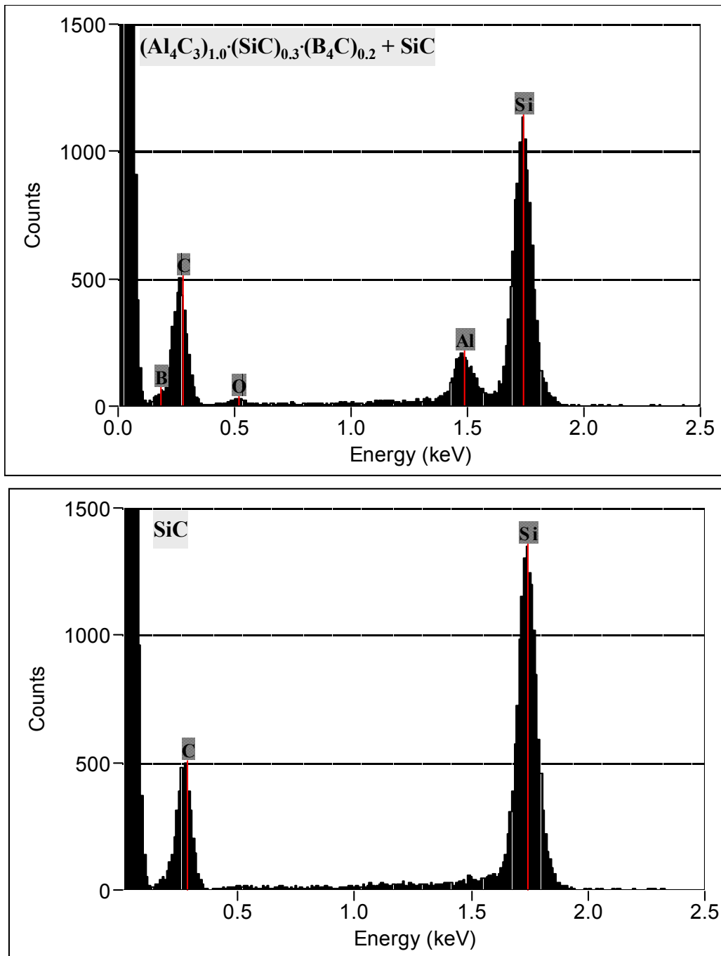
Fig. 7: Point EDS spectra obtained from (a), a large precipitate in 1600 °C-annealed SiC, and (b), an area in the SiC matrix 20 nm away from the precipitate under analyzing. The spectrum in (b) was subtracted from that in (a) to get net counts for the EDS peaks. An \text{Al}_4\text{C}_3 -based composition was therefore determined for the precipitate, which contained \text{B}_4\text{C} and SiC solid solutions as marked in (a).
