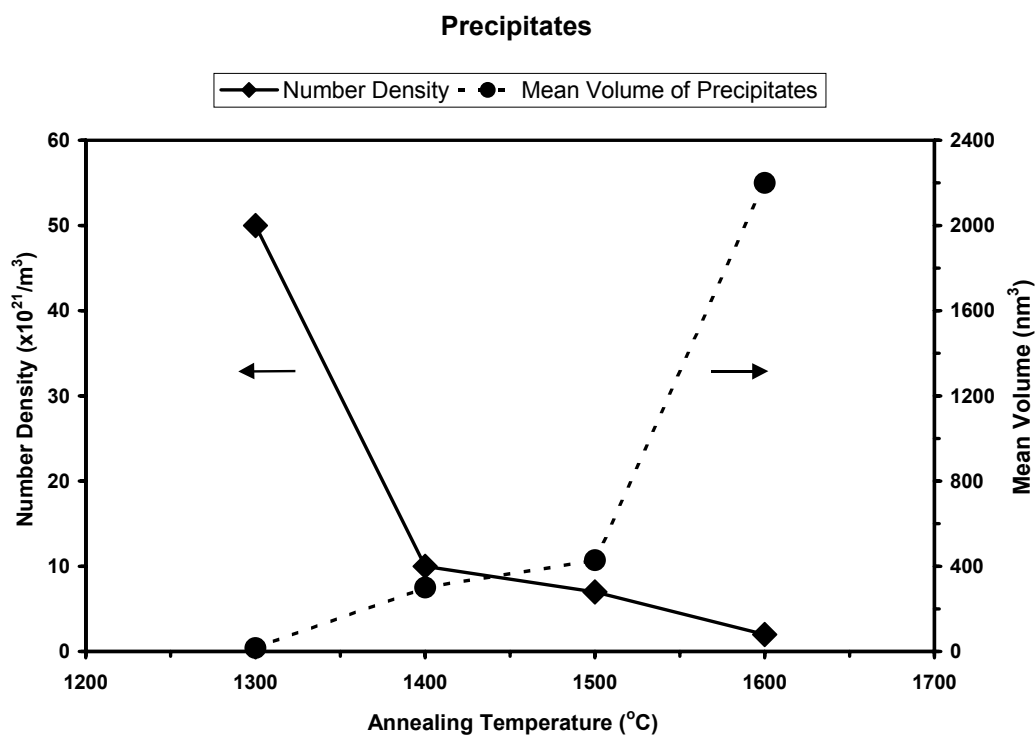
Fig. 4: A plot for change of number density and mean volume of the precipitates with increasing annealing temperature.
