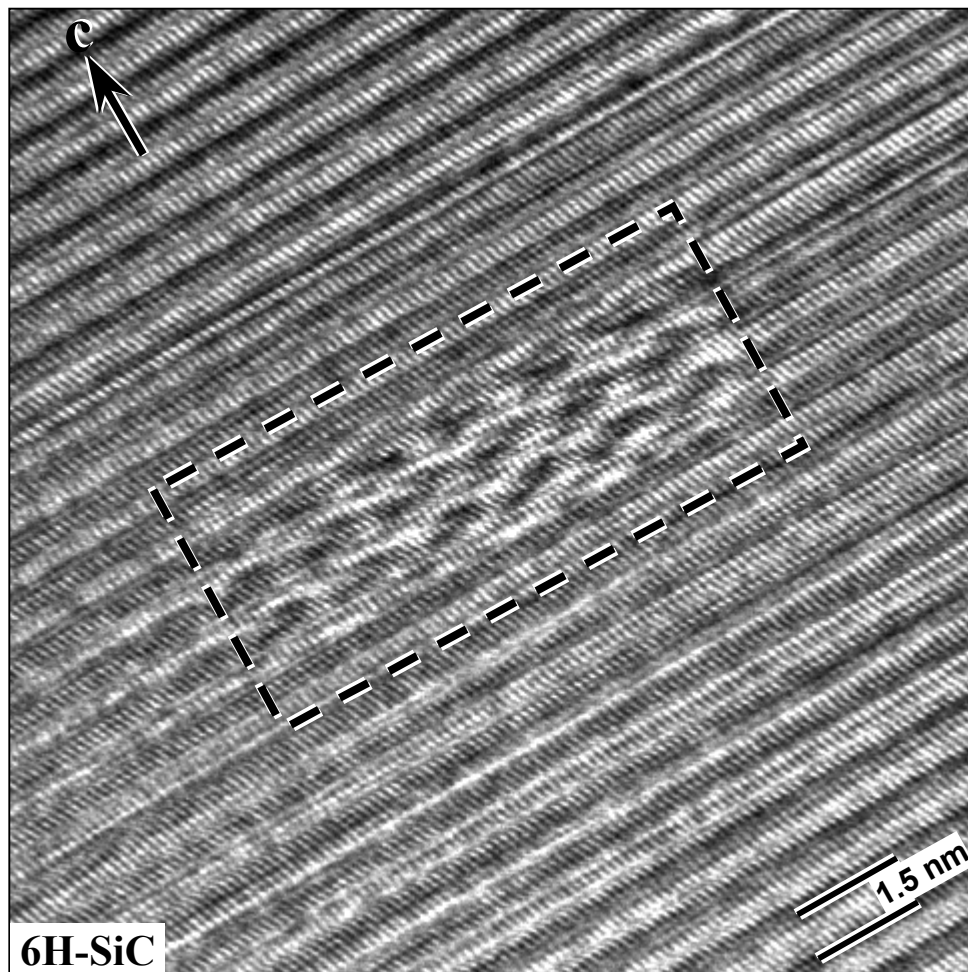
Fig. 10: High-resolution image taken along the [11\bar{2}0] zone-axis direction of a 6H-SiC grain. Inside the dashed-line frame is a nano-precipitate, which was not perfectly aligned with the SiC matrix. An about 7^\circ clockwise tilting of the \text{Al}_4\text{C}_3 (0001) plane about the incident beam direction results in moiré fringes in the framed region.
