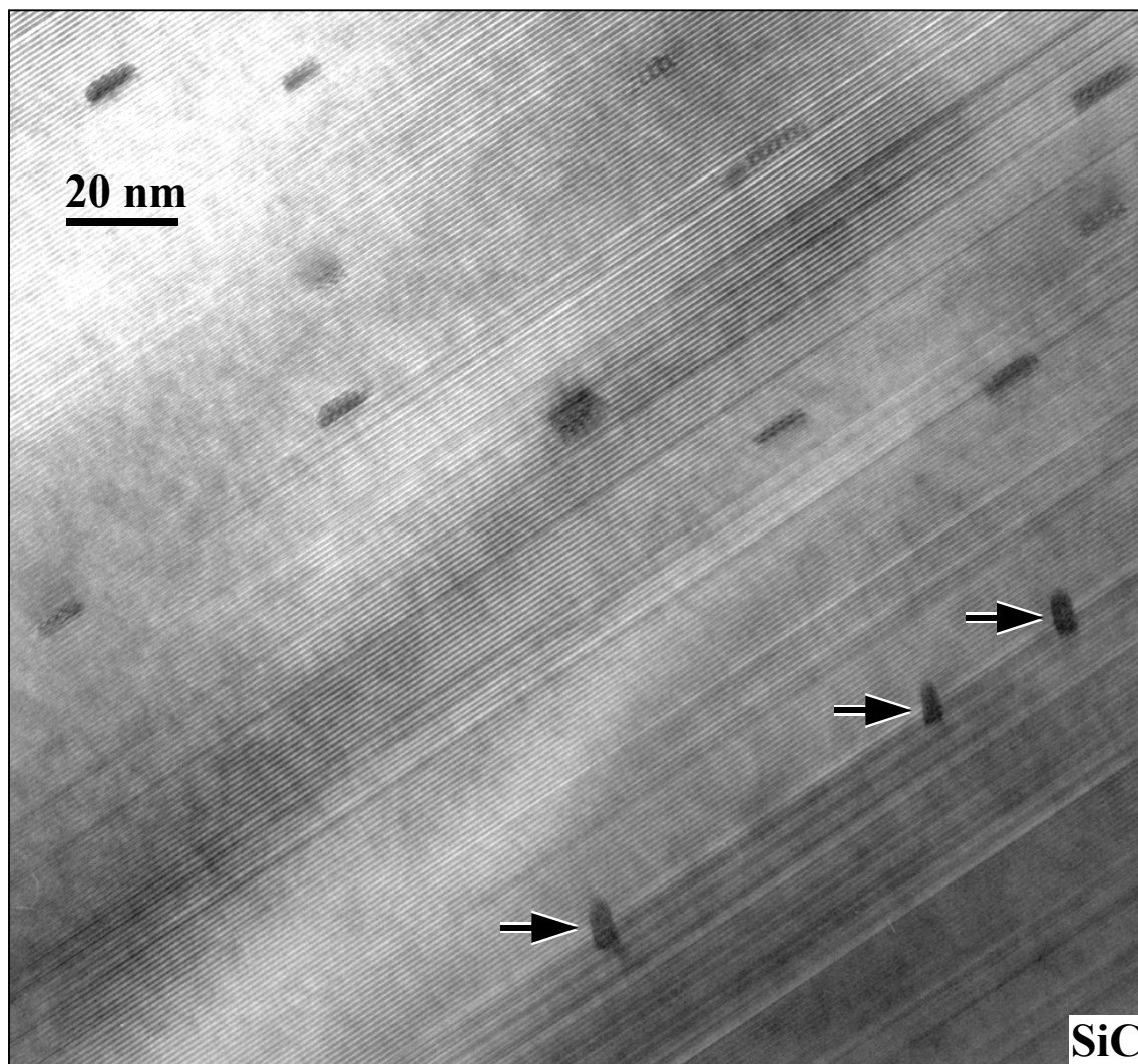
Fig. 3: Lattice-fringe image showing precipitates formed in ABC-SiC annealed at 1600 °C for 168 hrs. Note the bigger size but less amount density of the precipitates compared with those in Fig. 1, and Fig. 2. Three precipitates tilted away from the SiC (0001) habit plane are indicated by arrows.
