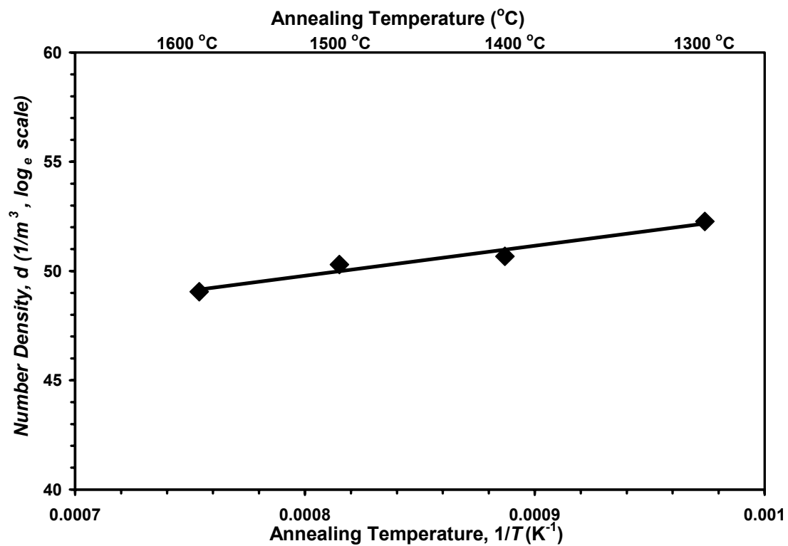
Fig. 11: Change of number density of precipitates ( d ) as a function of annealing temperature 1/T (note the unit for T is Kelvin). Linear relation is seen.
