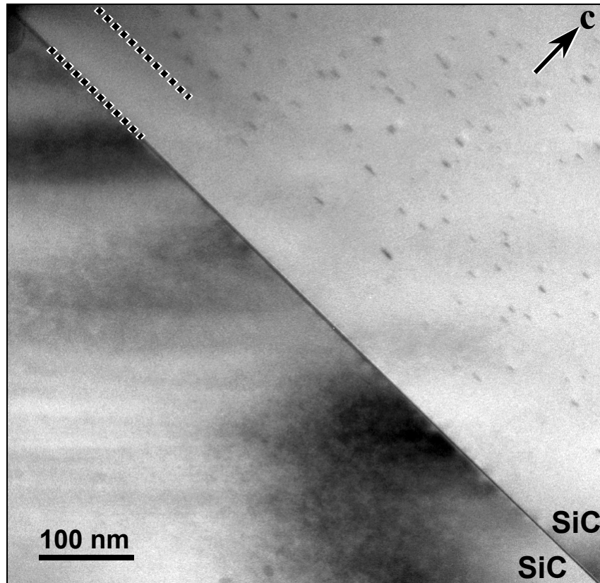
Fig. 5: A TEM micrograph showing a SiC grain boundary and the vicinity area in a sample annealed at 1400 °C. Nano-precipitates can be seen in the upper-right side SiC grain. Two dot lines mark an about 65 nm wide grain boundary zone, in which the number of the precipitates is much less than the grain interior. The precipitates in the lower-left side SiC grain cannot be distinguished because of the unfavorable imaging orientation.
