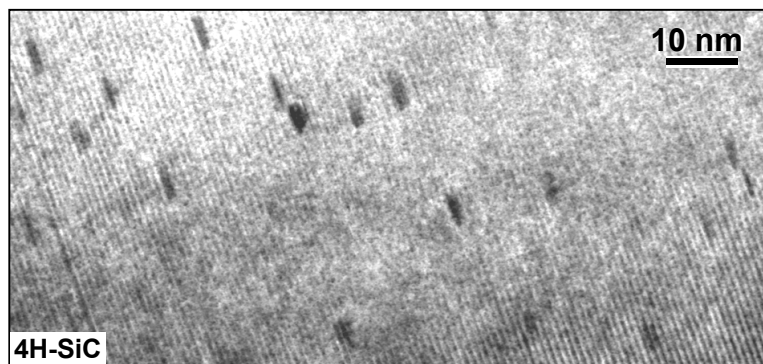
Fig. 1: Lattice-fringe image showing nanoscale precipitates in a 4H-SiC grain. The sample was annealed at 1300 °C for 85 hrs.
