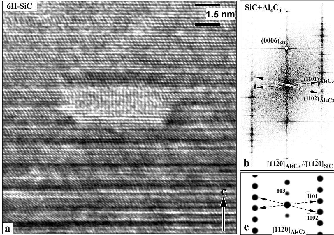
Fig. 8: (a). High-resolution image showing crystalline structure of a nano-precipitate in the 6H-SiC matrix. The image was taken along the [11\bar{2}0] zone-axis direction of the hexagonal SiC structure. Some buckled atomic planes can be seen in the precipitate, at a glance angle along the c -normal direction. (b). A Fourier transform from the high-resolution image in (a). The (0006) reflection from the \alpha -6H SiC is marked as (0006)_{6H} . Extra reflections, indicated by double-head arrows, can be indexed as (\bar{1}101) and (\bar{1}10\bar{2}) , respectively, based on the Al_4C_3 [11\bar{2}0] zone-axis diffraction pattern. (c). A computer simulated electron diffraction pattern for the Al_4C_3 structure along the [11\bar{2}0] zone-axis direction. Double-head arrows indicate reflections experimentally observed in (b).
