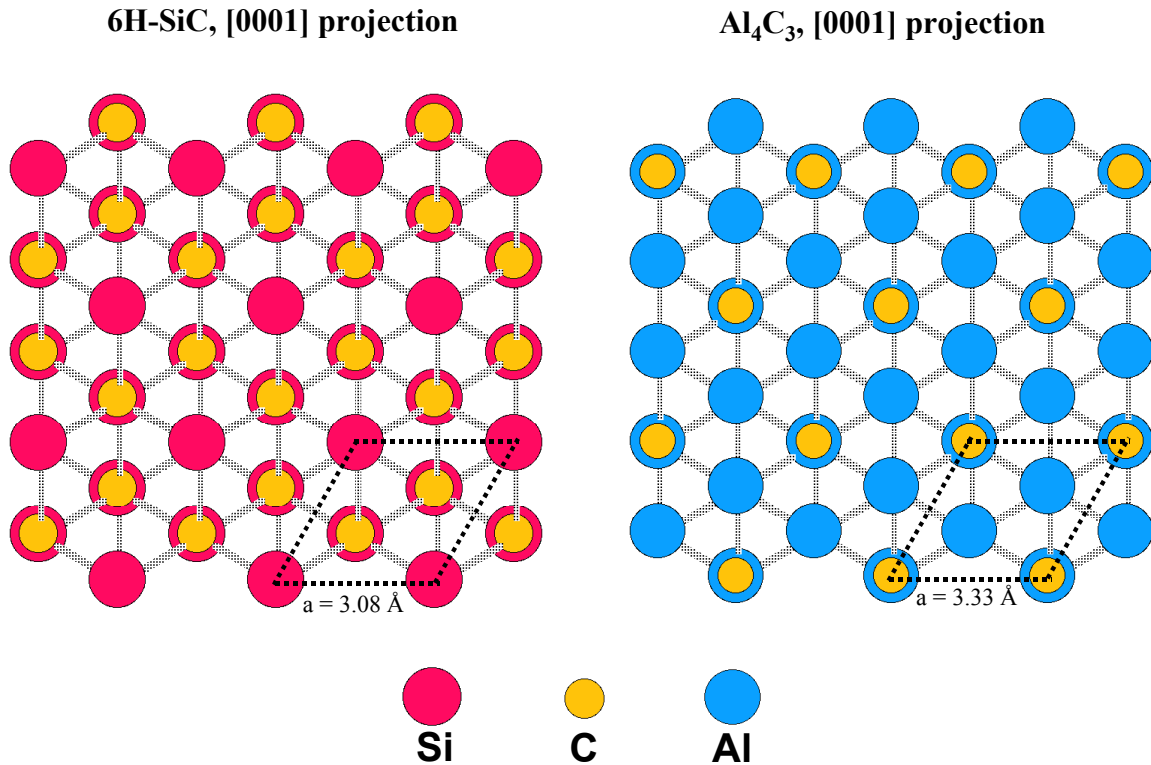
Fig. 9: [0001] projected structures for the 6H-SiC and the Al 4 C 3 , respectively. Grey color dashed lines represent the Si-C, or Al-C bonds. Atoms on different atomic layers along the projected direction cause the visual superposition in the projection. The dot lines marked the two-dimensional unit cells for the two structures, respectively.
