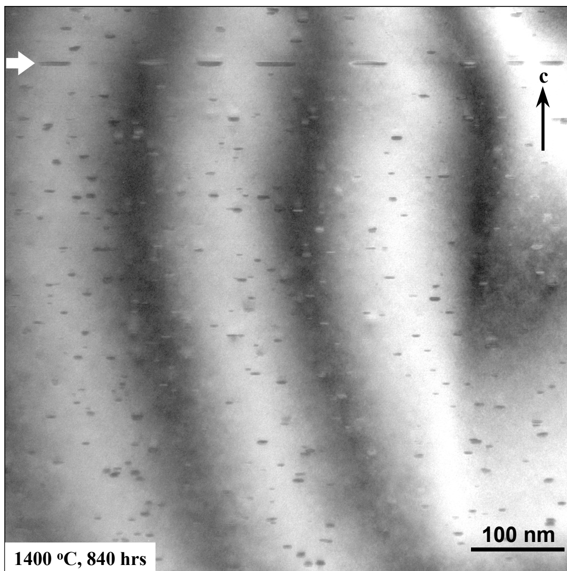
Fig. 2: A TEM micrograph showing highly dense nanoscale precipitates in the ABC-SiC annealed at 1400 °C for 840 hrs. A bold arrow indicates the unusually elongated precipitates.
