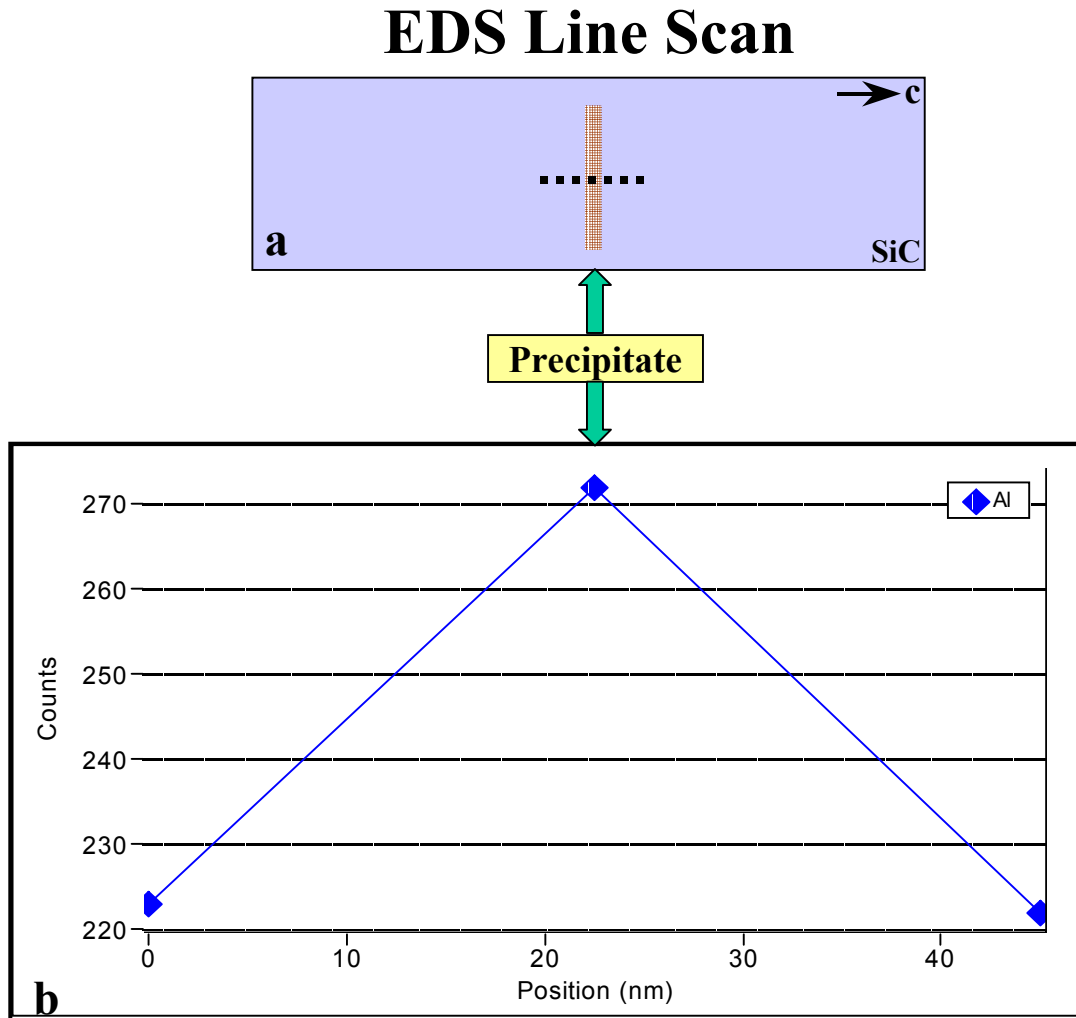
Fig. 6: (a). A schematic illustration for EDS line-scan across a nano-precipitate in a SiC grain. (b). Aluminum profile along a line, which was scanned by an 8 nm diameter electron beam probe, is presented. The EDS counts are proportional to the concentration. Note the increased Al concentration at the position of the precipitate.
