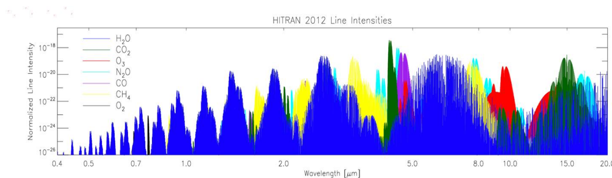
Figure 3.7: Combined spectral feature catalog for O_2 - O_2 , CO_2 , CO, H_2O and other molecules.
