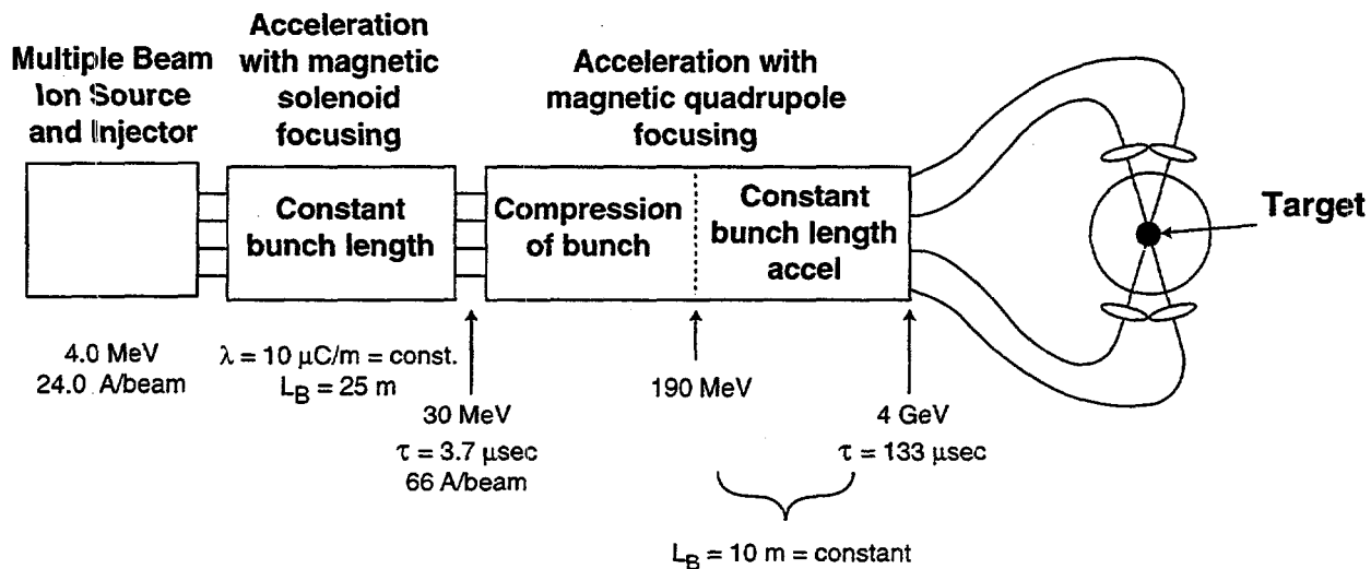
Figure 1. Solenoid-Based Four Beam Reference Design for Driver (Singly Charged Cesium)
