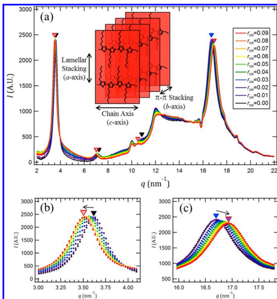
Figure 3. (a) Representative 1D WAXS profiles for one of the P3HT-PEO replicates for a range of doping levels. Peaks corresponding to P3HT (100, 200, 300, and 020) are indicated with triangle markers. The solid black and blue markers indicate the peak positions before doping, and the red highlighted markers indicate the peak positions at r_{ox} = 0.09 . The inset provides a schematic for the crystal structure of P3HT. (b) Expanded view of the (100) peaks. (c) Expanded view of the (020) peaks.
