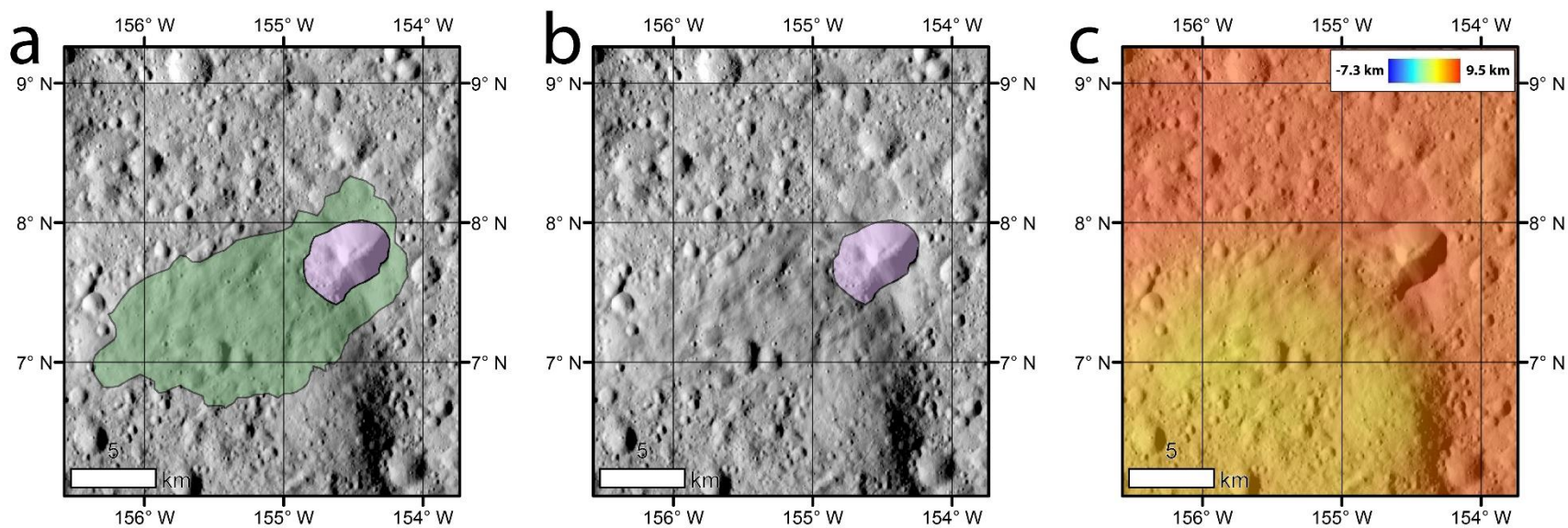
Figure A-17. (a) Unnamed crater ( -154.56^{\circ} E, 7.74^{\circ} N) with mapped cusate/lobate FAE deposit. (b) same image as (a) but with ejecta related map overlays removed. (c) same image as (a) but with all mapping overlays replaced by color coded HAMO derived topography.
