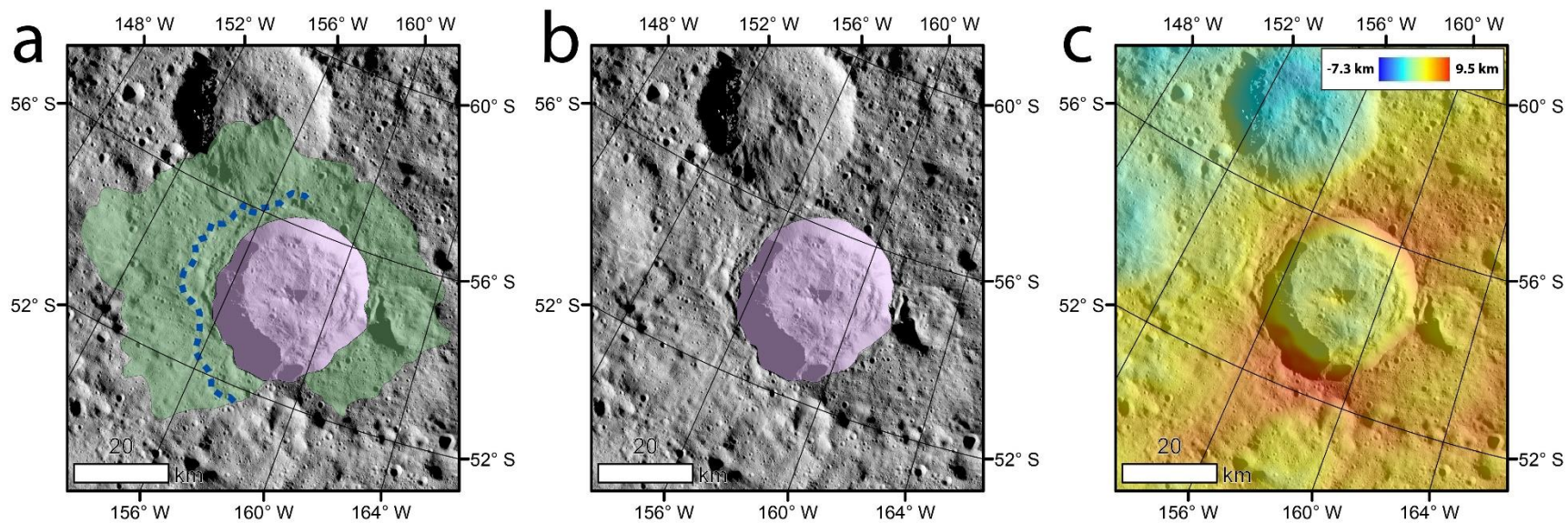
Figure A-12. (a) Unnamed crater ( -158.41^{\circ} E, -54.39^{\circ} N) with mapped cusate/lobate FAE deposit. (b) same image as (a) but with ejecta related map overlays removed. (c) same image as (a) but with all mapping overlays replaced by color coded HAMO derived topography.
