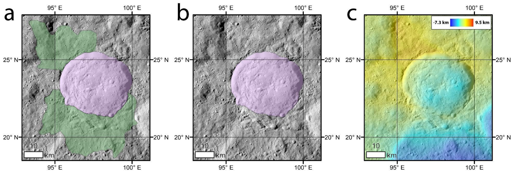
Figure A-5. (a) Aristaeus crater with mapped cusate/lobate FAE deposit. (b) same image as (a) but with ejecta related map overlays removed. (c) same image as (a) but with all mapping overlays replaced by color coded HAMO derived topography.
