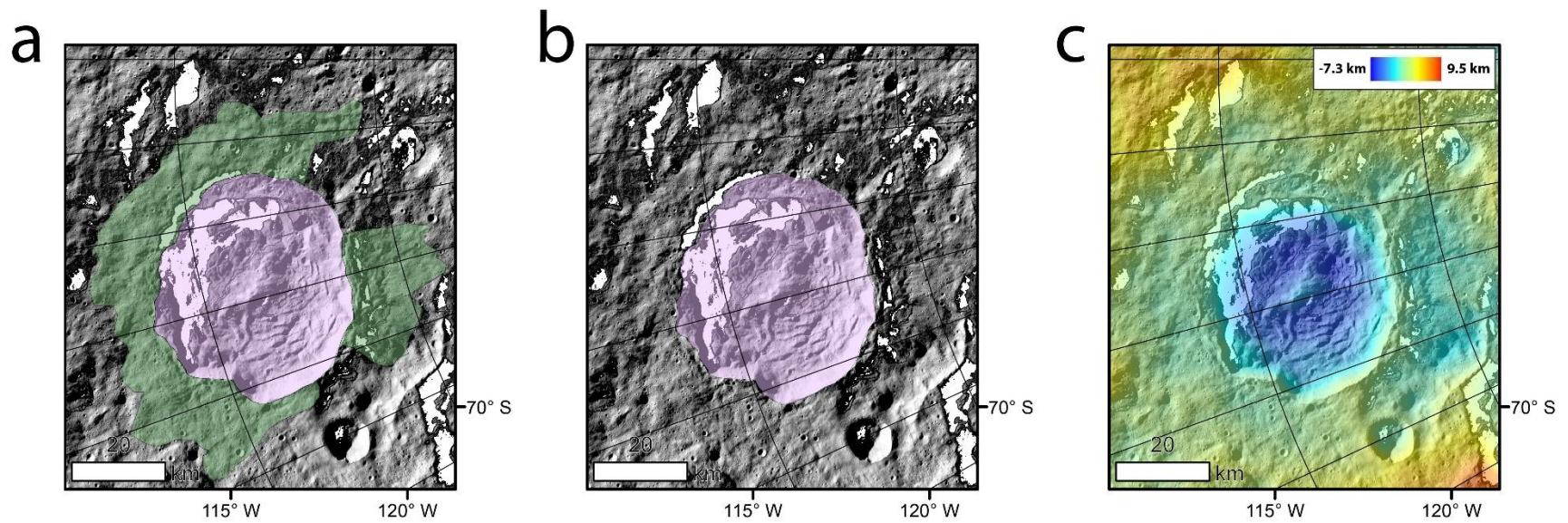
Figure A-13. (a) Sekhet crater with mapped cuscate/lobate FAE deposit. (b) same image as (a) but with ejecta related map overlays removed. (c) same image as (a) but with all mapping overlays replaced by color coded HAMO derived topography.
