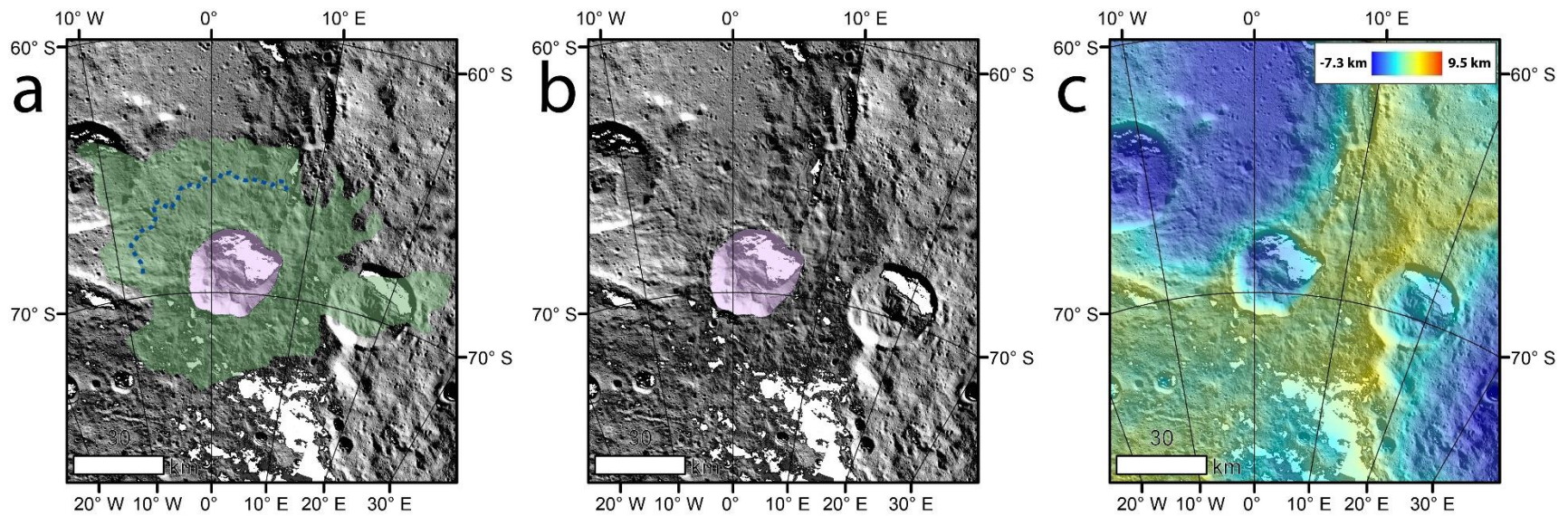
Figure A-14. (a) Jacheongbi crater with mapped cusped/lobate FAE deposit. (b) same image as (a) but with ejecta related map overlays removed. (c) same image as (a) but with all mapping overlays replaced by color coded HAMO derived topography.
