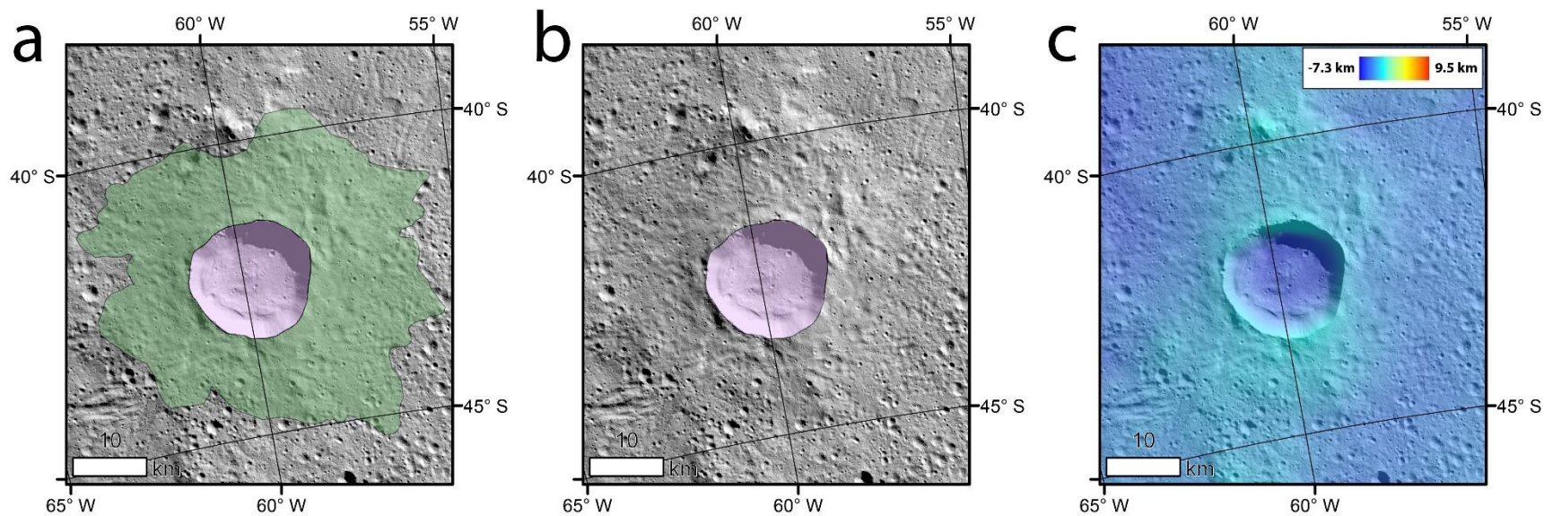
Figure A-9. (a) Besua crater with mapped cusate/lobate FAE deposit. (b) same image as (a) but with ejecta related map overlays removed. (c) same image as (a) but with all mapping overlays replaced by color coded HAMO derived topography.
