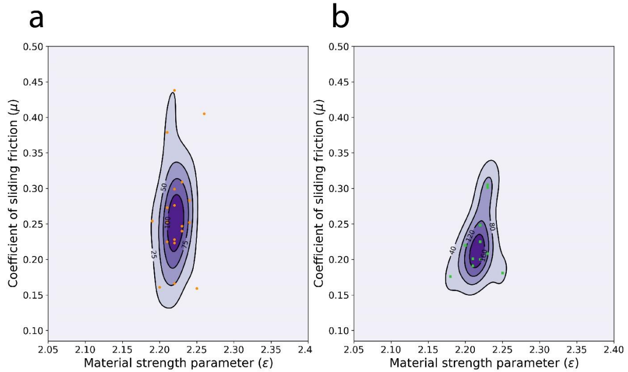
Figure 4-10. 2-Dimensional KDE analysis of the model derived \epsilon and \mu values for the cerean FAE. The labeled contour values are the probability density, with the color coding indicating increased probability with darkening color. Subplot (a) shows the cusate/lobate FAE (orange circle), while (b) displays the channelized FAE (green squares).
