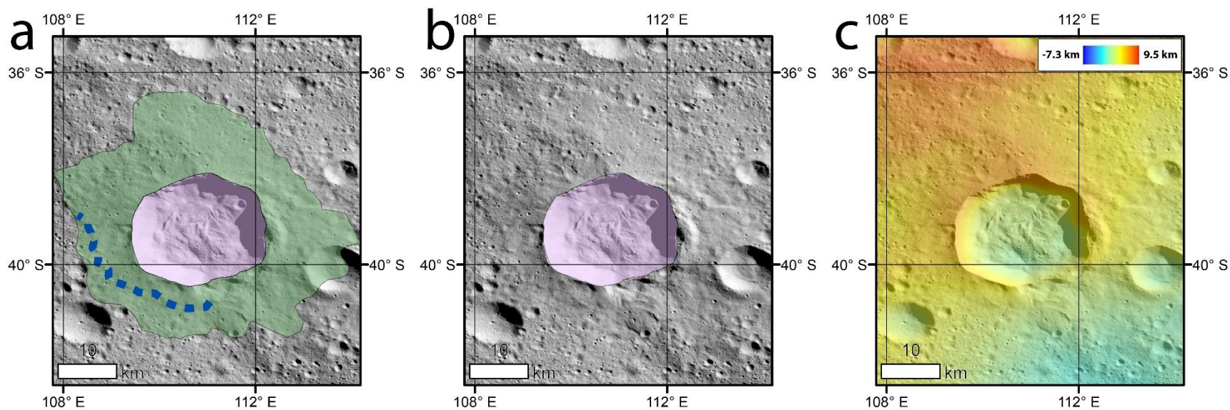
Figure A-11. (a) Unnamed crater (110.82° E, -39.29° N) with mapped cusate/lobate FAE deposit. (b) same image as (a) but with ejecta related map overlays removed. (c) same image as (a) but with all mapping overlays replaced by color coded HAMO derived topography.
