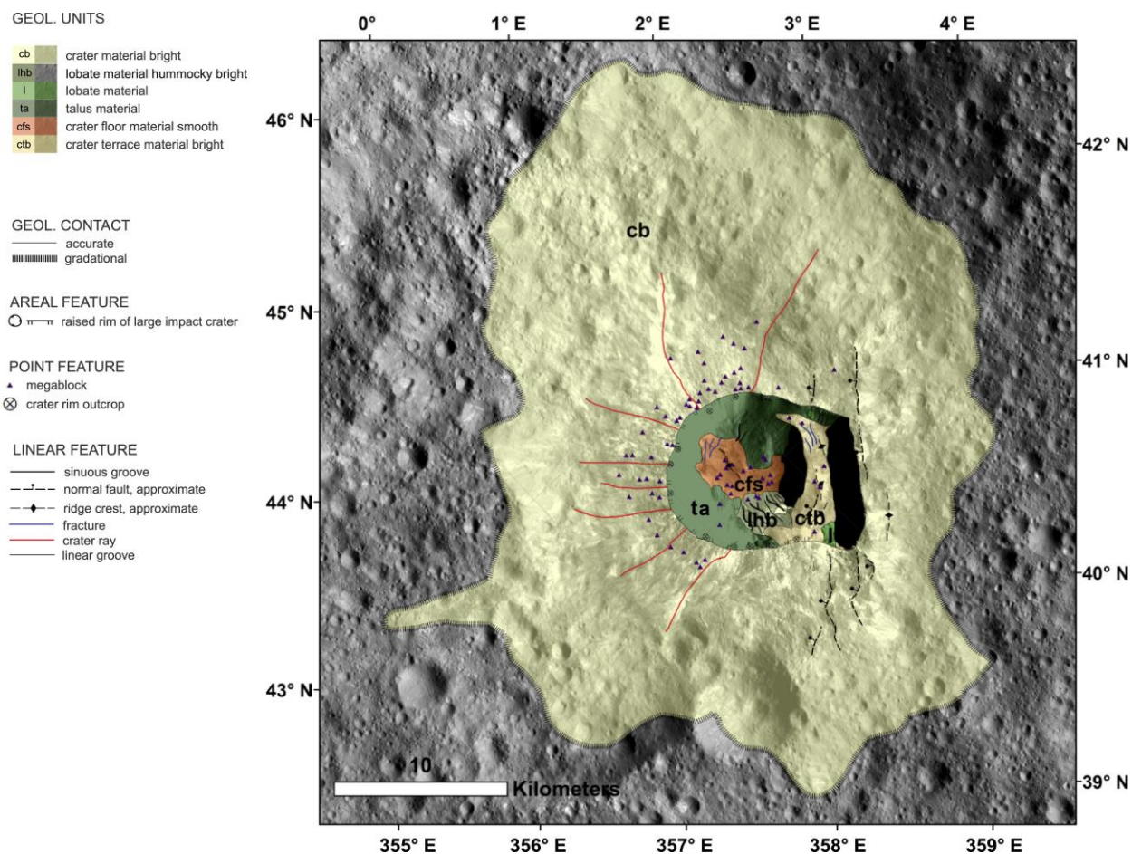
Figure 2-16. Geologic map of Oxo crater. The geologic map is shown is overlain onto a FC LAMO clear filter mosaic. The primary H 2 O detection is located at 41.8 °N, 359.8 °E, which is nearly coincident with the crater floor material bright enclave within the crater floor material hummocky unit in the lower central region of the crater. The secondary H 2 O detection is located at 41.4 °N, 359.9 °E, which is coincident with the lobate material unit in the lower right corner of Oxo’s slump terrace. Both of these detections are discussed in detail in Combe et al. (2016). Crater rim outcrops indicate major rocky protrusions around Oxo. These outcrops are commonly situated at the origins of bright and dark material streaks.
