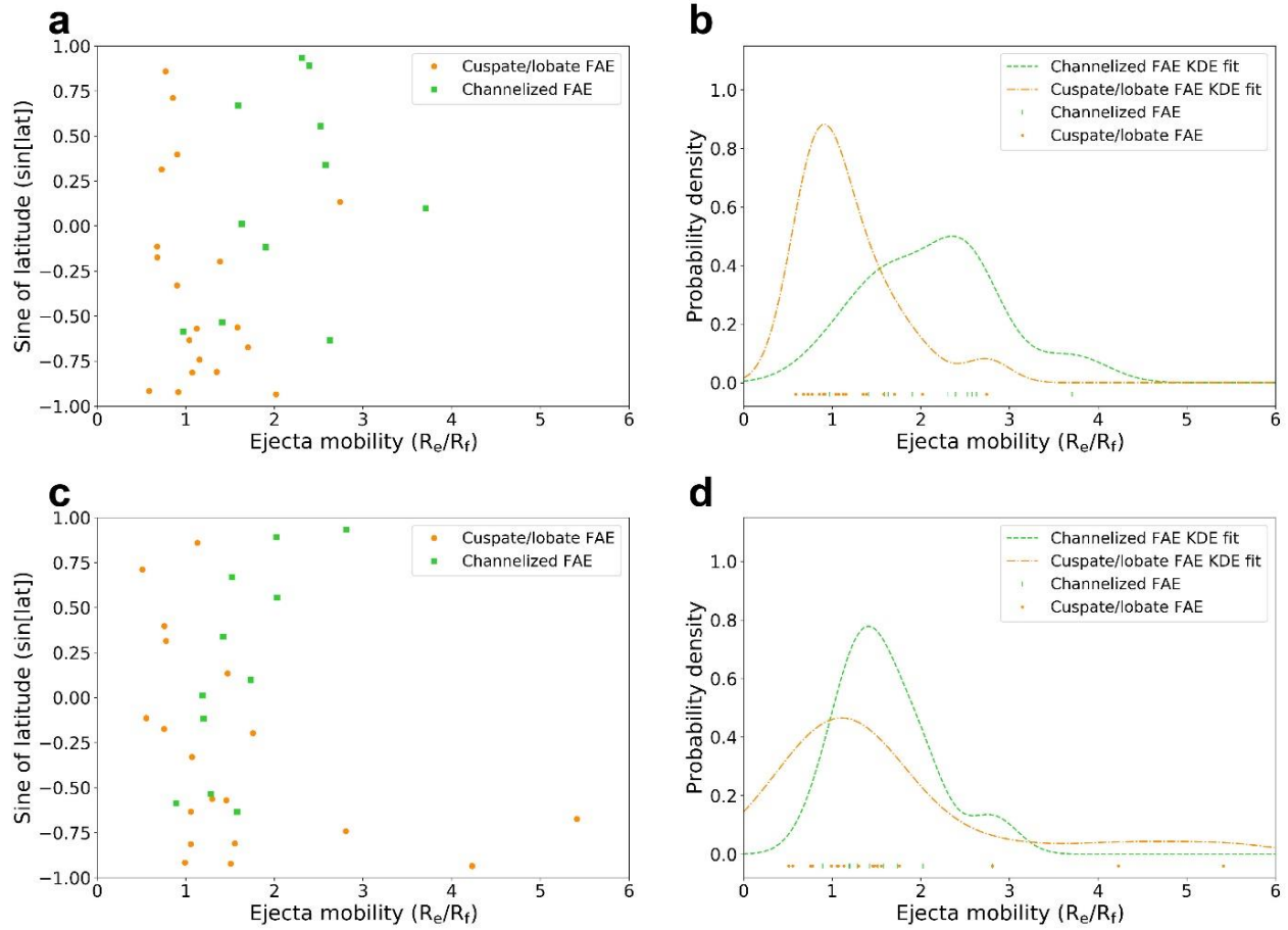
Figure 4-8. (a) Plot of the latitudinal distribution of the cusate/lobate (orange circles) and channelized (green squares) cerean FAE as a function of their observed (i.e. non-slope corrected) EM values. (b) Normalized KDE analysis of the observed EM distribution functions for the cusate/lobate and channelized FAE. (c) Plot of the latitudinal distribution of the cusate/lobate (orange circles) and channelized (green squares) cerean FAE as a function of their 7.5^\circ slope corrected EM values (i.e. the EM value for each FAE was adjusted using the model outlined in section 2.4 as if its mean regional radial slope was 7.5^\circ ). (d) Normalized KDE analysis of the slope corrected EM distribution functions for the cusate/lobate and channelized FAE. Note the slight increase in mobility of FAE at higher latitudes in the slope corrected subfigure (c). The point markers in (b) and (d) indicate the locations of each individual FAE on the EM axis. In
