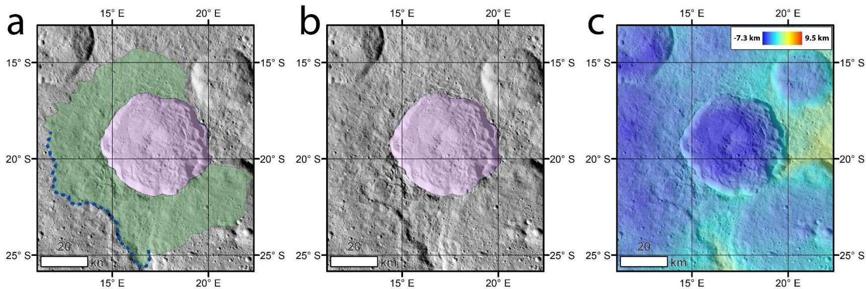
Figure A-8. (a) Kondos crater with mapped cuscate/lobate FAE deposit. (b) same image as (a) but with ejecta related map overlays removed. (c) same image as (a) but with all mapping overlays replaced by color coded HAMO derived topography.
