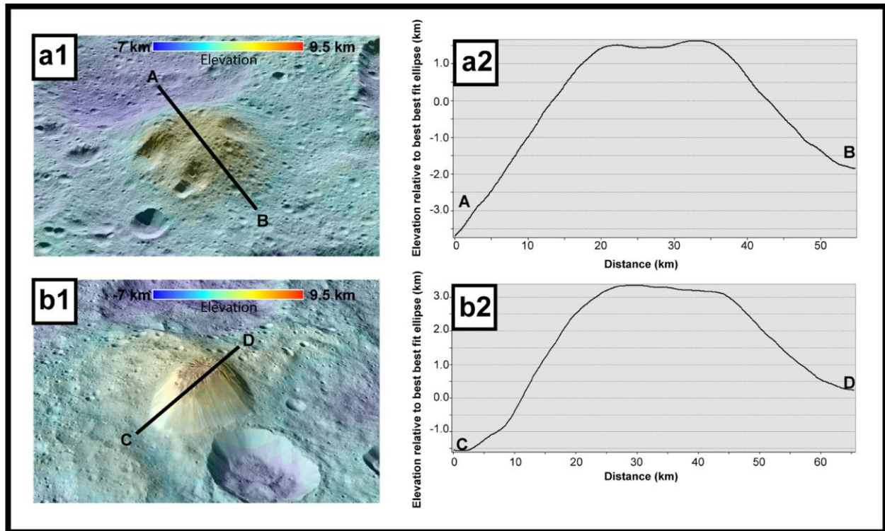
Figure 2-11. Perspective views and topographic profiles of Hosil tholus and Ahuna Mons (located in the Ac-10 Rongo Quadrangle). Hosil tholus, whose perspective view and profile are shown in panel (a1) and (a2), respectively, is the most morphologically similar example to Ahuna Mons found in the Fejokoo quadrangle. Ahuna Mons is depicted in panel (b1), and its profile is shown in panel (b2). The perspective views and profiles were created using the HAMO DTM. Vertical exaggeration in panels (a1) and (a2) is a factor of two. Panels (b1) and (b2) are vertically exaggerated by a factor of five.
