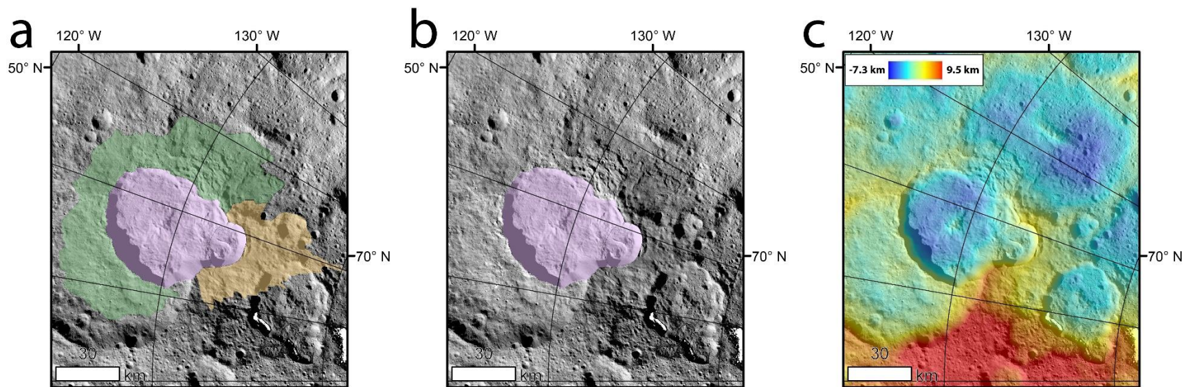
Figure A-2. (a) Datan and a small unnamed crater to its north ( -107.88^{\circ} E, 63.09^{\circ} N) with mapped cusate/lobate and channelized FAE deposits. (b) same image as (a) but with ejecta related map overlays removed. (c) same image as (a) but with all mapping overlays replaced by color coded HAMO derived topography.
