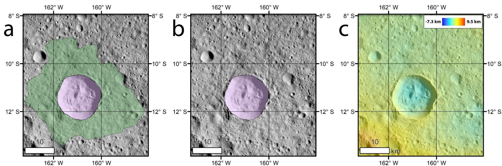
Figure A-28. (a) Unnamed crater (-160.93° E, -11.39° N) with mapped cusate/lobate FAE deposit. (b) same image as (a) but with ejecta related map overlays removed. (c) same image as (a) but with all mapping overlays replaced by color coded HAMO derived topography.
