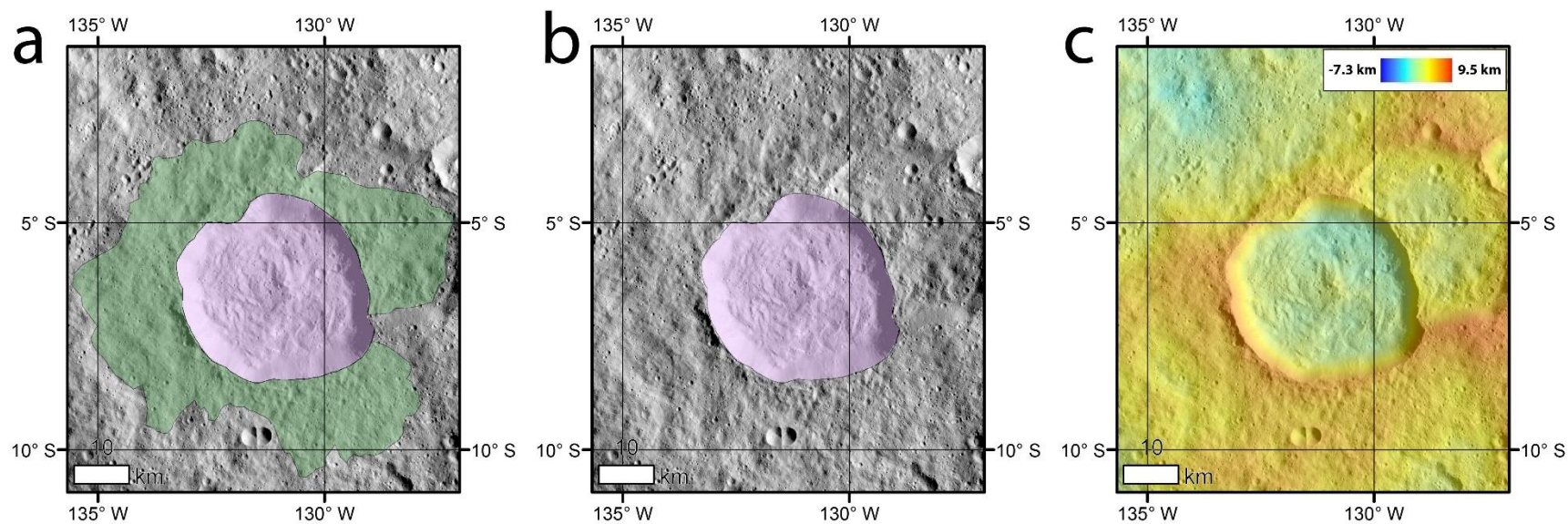
Figure A-7. (a) Lociyo crater with mapped cusate/lobate FAE deposit. (b) same image as (a) but with ejecta related map overlays removed. (c) same image as (a) but with all mapping overlays replaced by color coded HAMO derived topography.
