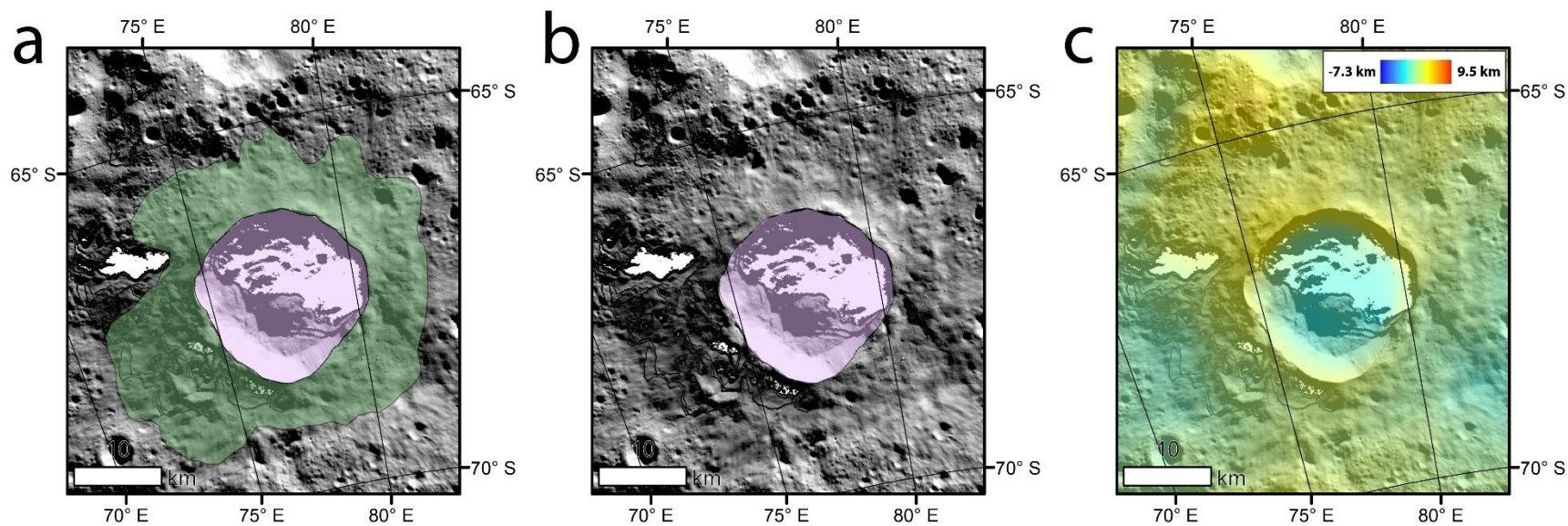
Figure A-20. (a) Ratumaibulu crater with mapped cusate/lobate FAE deposit. (b) same image as (a) but with ejecta related map overlays removed. (c) same image as (a) but with all mapping overlays replaced by color coded HAMO derived topography.
