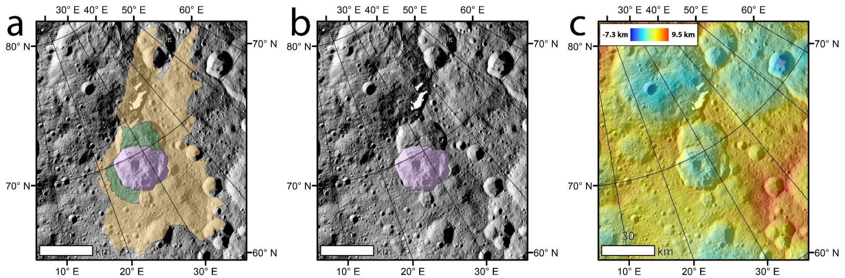
Figure A-1. (a) Shennong crater with mapped cusate/lobate and channelized FAE deposits. (b) same image as (a) but with ejecta related map overlays removed. (c) same image as (a) but with all mapping overlays replaced by color coded HAMO derived topography.
