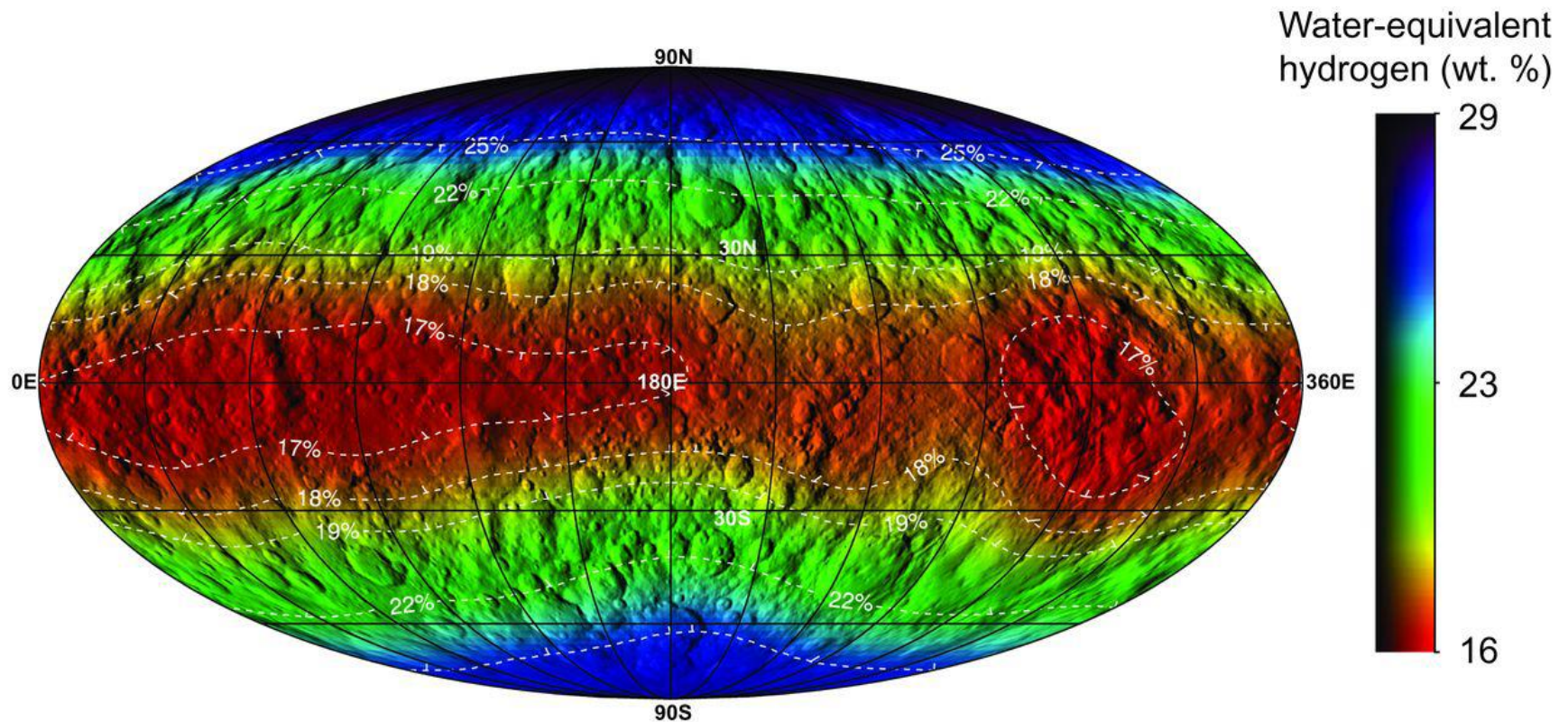
Figure 1-11. The lower bound distribution of water equivalent hydrogen within the top ~1 m of Ceres' regolith. This determination was made using thermal and epithermal neutron counting data taken by Dawn's GRaND instrument. To first order, the abundance of hydrogen in the upper regolith of Ceres correlates largely with latitude; the poles appear enriched in hydrogen relative to the seemingly depleted equatorial region. Note that while this latitudinal trend in poleward hydrogen enrichment is broadly symmetrical
