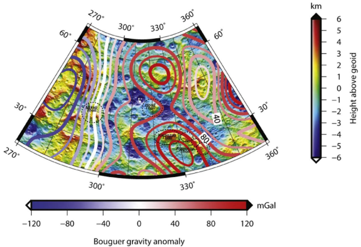
Figure 2-12. Bouguer gravity anomaly map of the Fejokoo quadrangle. The location and approximate size of the Fejokoo quadrangle tholi are indicated by dashed ellipses. The gravity model used is computed to degree n = 16 for a two-layer model. The specific parameters for the model are presented in Ermakov et al. (2017).
