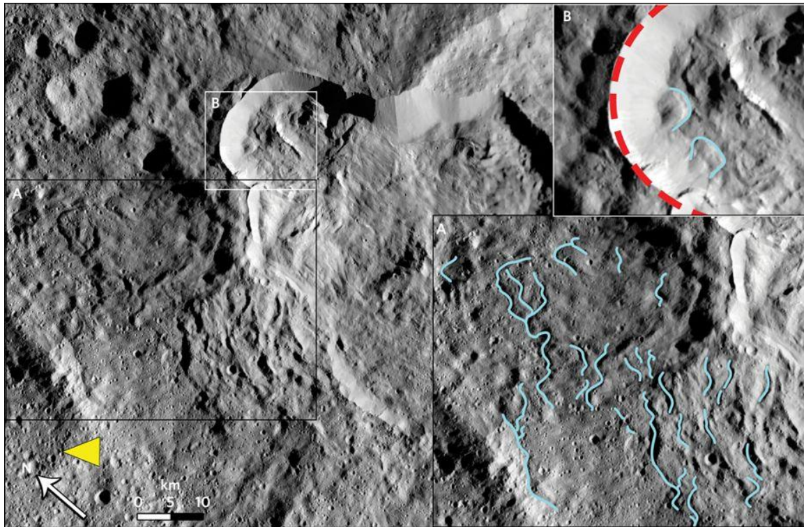
Figure 3-3. Example of a Type 3 lobate flow. These feature typically have a platy, smooth, lobate morphology with multiple superposed sheeted layers and numerous cusped terminal lobes. The archetypical cerean Type 3 flow shown in this image is located in Datan crater (60° N, 250° W). The black inset shows the flows in detail. Yellow arrows indicate the direction of incident sunlight, light blue solid lines show flow margins, and red dashed lines delineate crater rims. The frontal flow margins trace v-shaped cusped toes of the many flow sheets. The length of this flow ranges from ~17–32 km. The white inset shows terracing and two lobate flows on the interior of a presumably post-impact failed rim. These landslides could represent talus cones within the crater. Image adapted from Schmidt et al. (2017).
