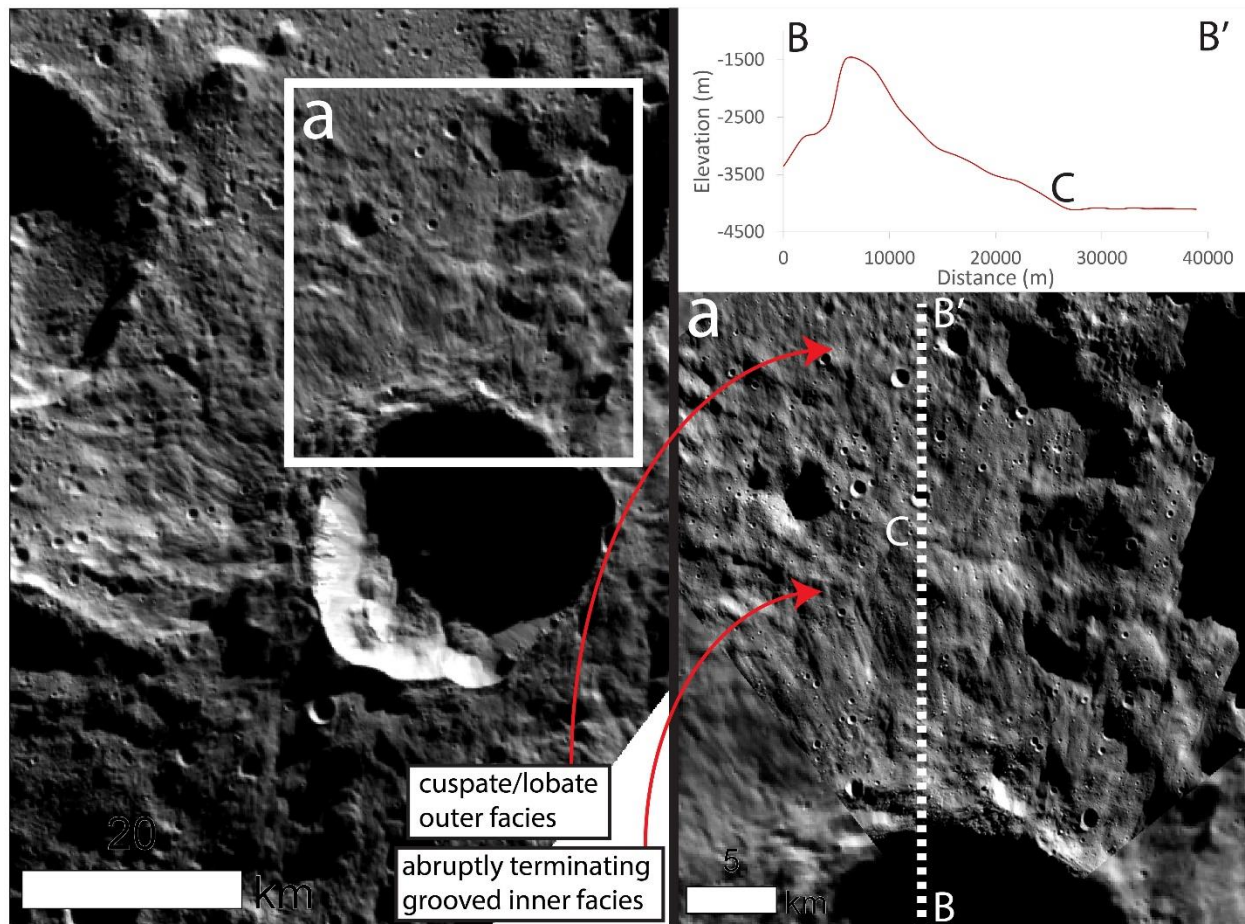
Figure 4-3. Expanded view of Jacheongbi crater and the northern portion of its cusate/lobate FAE deposit as seen in Figures 4-2d, 4-2e, and 4-2f. In inset (a) note the arcuate-to-cusate v-shaped lobes near the upper red arrow. This morphology is common among the outer facies of double- and multiple-layered ejecta on Mars as well as the other cusate/lobate cerean FAE, and were used, in part, to help determine the outer margins of cusate/lobate ejecta facies. The inner ejecta facies near the lower red arrow in inset (a) displays superimposed longitudinal grooves and an abruptly terminating margin, which is noticeable in the included topographic cross-section. These characteristic are often associated with the inner ejecta facies of martian double layer ejecta.
