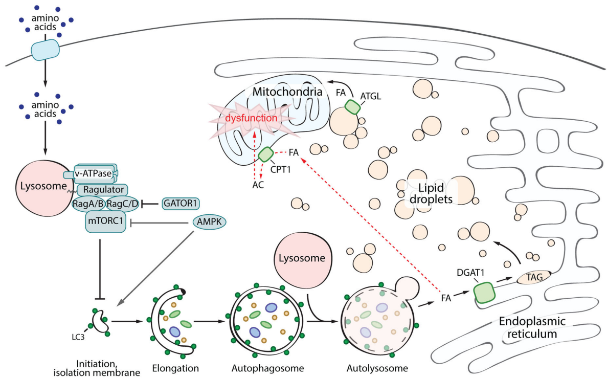
Figure 7. DGAT1-dependent lipid droplet biogenesis prevents lipotoxicity during starvation-induced autophagy
