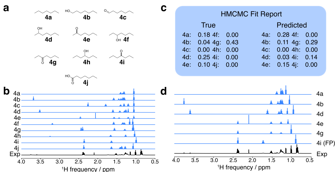
Figure 7. Results of HMMCM deconvolution of the spectrum from the heptane oxidation simulation. (a) Candidate library containing compounds 4a–4j, (b) initial DFT-generated spectra before HMMCM fitting, (c) final HMMCM fit report showing the predicted composition, and (d) final deconvoluted spectra showing the HMMCM-fit spectra of the molecules determined to be in the experimental mixture. The false positive prediction is denoted as (FP). The experimental spectrum was acquired at 700 MHz.
