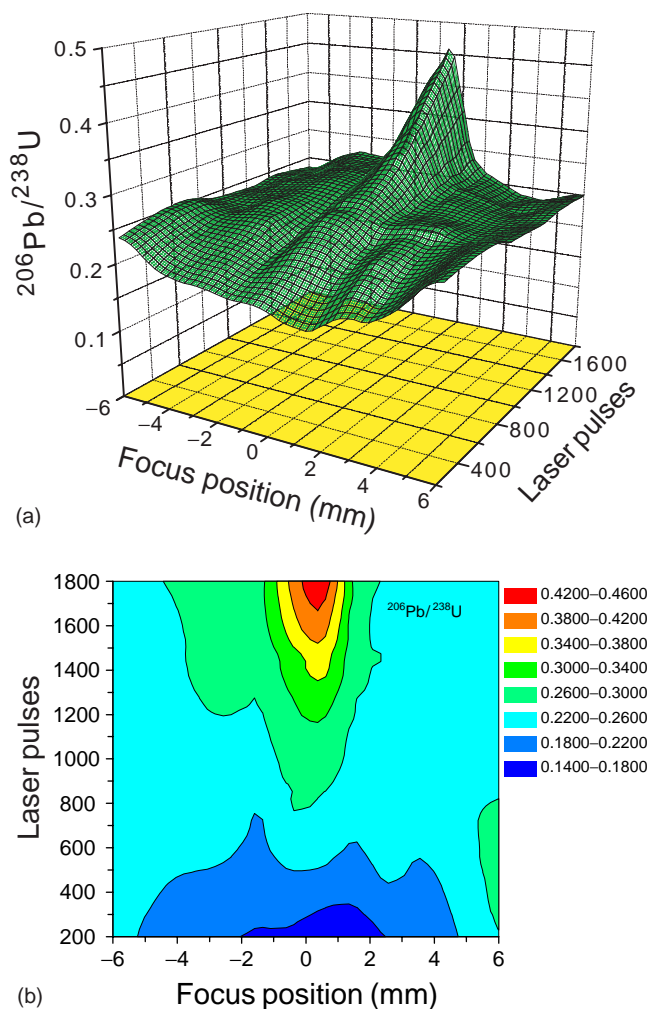
Figure 3 Pb–U fractionation versus number of laser pulses and lens-to-sample focal position (a) three-dimensional plot; (b) contour plot. Neodymium:yttrium aluminum garnet (Nd:YAG) laser, \lambda = 213 nm; pulse duration = 6 ns; energy = 1.15 mJ; sample: NIST SRM 610 glass in which the ^{206}\text{Pb}/^{238}\text{U} stoichiometric ratio is 0.2249. The positive and negative values represent the laser focus above and below the sample surface, respectively.
