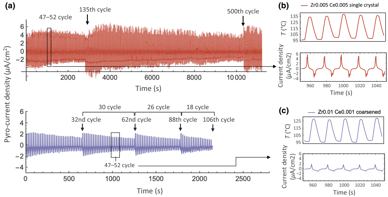
FIG. 7. Energy conversion by phase-transforming ferroelectric crystals. (a) Pyro-current density generated by the Zr0.005 Ce0.005 single-crystal capacitor (red) and the Zr0.01 Ce0.001 coarse-grained capacitor (blue) over hundreds of transformation cycles. (b),(c) Pyroelectric current density of 47 to 52 cycles corresponding to the applied temperature profiles.
