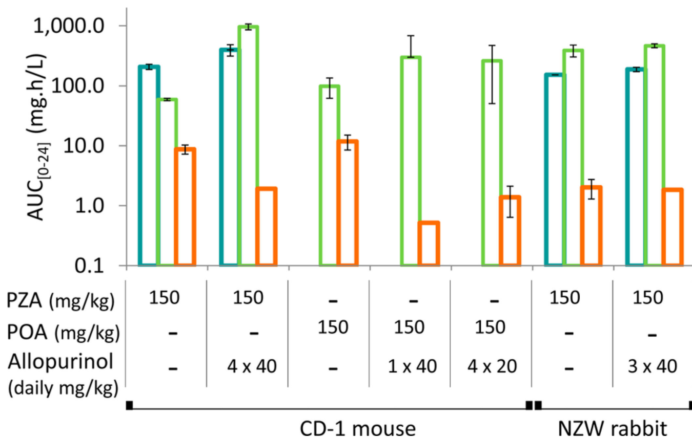
Figure 5. Effect of xanthine oxidase inhibition by varying allopurinol predosing schedules on the metabolism of PZA and POA in CD-1 mice and NZW rabbits. Blue bars, AUC_{[0-24]} of PZA; green bars, AUC_{[0-24]} of POA; orange bars, AUC_{[0-24]} of 5-hydroxy-POA.
