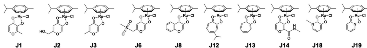
Fig. 1 Chemical structures of Ru-arene compounds that comprise the original class J metallofragments. Compounds J1 , J13 , and J19 were re-examined for their stability and inhibitory activity in this correction.
