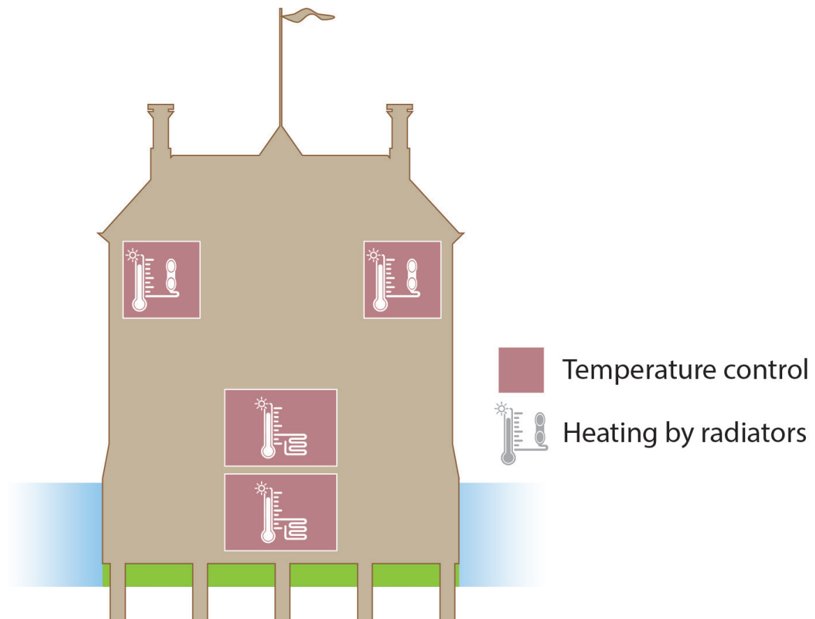
IMAGE 12 (top). Che Grand Salon on the belle etage (main floor). MARC STAPPERS IMAGE 13 (bottom). Amerongen Castle with the floor heating on two levels, the basement and the hallways on the ground floor. The former living apartments, now office spaces, are heated by radiators. The unheated historic rooms will be minimally heated by the adjacent heated spaces. BART ANKERSMIT
