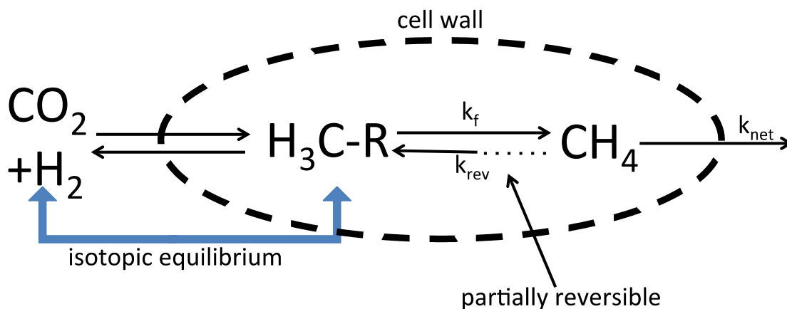
Figure A3: Cartoon of the isotopically enabled model of methane formation described in the main text and appendix. The dotted lines mark the boundary between the methanogen cell and extracellular water. In this model, \text{CO}_2 and \text{H}_2 are assumed to always be in isotopic equilibrium with a methyl group bound to coenzyme M (here symbolized with the 'R') following the differential reversibility hypothesis of Valentine et al., (2004). Additionally, the \text{H}_2 and hydrogen in the methyl group bound to coenzyme M are assumed to be in isotopic equilibrium with the intracellular \text{H}_2\text{O} . In the model, the reversibility of methyl-coenzyme M reductase (the relative rates of the steps symbolized by k_{\text{rev}} vs. k_f ) is varied as discussed in the appendix.
