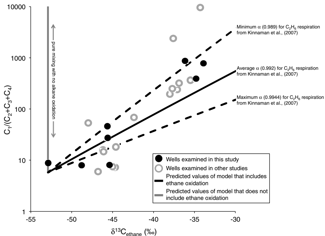
Figure 4: Mixing model's prediction of the \delta^{13}C of ethane as a function of the C_1/C_{2-4} ratio. \delta^{13}C values of ethane are from this study and from previous measurements from Martini et al. (2003) and Kirk et al. (2012). Fractionation factors ( \alpha ) for ethane oxidation are equal to (1000 + \delta^{13}C_{C_2H_6, \text{respired}})/(1000 + \delta^{13}C_{C_2H_6, \text{residual}}) , where 'respired' refers to the ethane that is respired by microbes and 'residual' refers to the remaining ethane. \alpha values for ethane oxidation are all from Kinnaman et al. (2007). The thermogenic end member is assumed to have a \delta^{13}C value of -52.9 ‰ and C_1/C_{2-4} of 5.8. See text for details.
