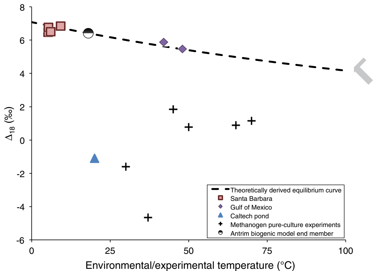
Figure 5: Measured or modeled \Delta_{18} values of biogenic gases from natural or experimental systems. The theoretically derived curve describes the expected \Delta_{18} value for methane isotopically equilibrated internally as a function of temperature and is from Stolper et al. (2014a). The Gulf of Mexico samples were reported in Stolper et al. (2014b). The Antrim biogenic model end member point is the value used in the mixing model of the Antrim Shale samples to describe the biogenic end member and is thus required to be on the equilibrium curve.
