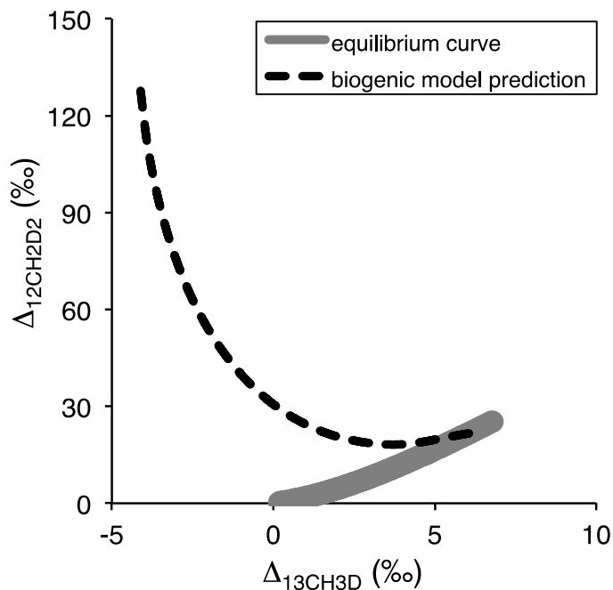
Figure 7: Comparison of the biogenic model (described in the text) vs. the expected values for internal isotopic equilibrium for \Delta_{12\text{CH}_2\text{D}_2} and \Delta_{13\text{CH}_3\text{D}} values. \Delta_{12\text{CH}_2\text{D}_2} = [([^{12}\text{CH}_2\text{D}_2]/[^{12}\text{CH}_4])/([^{12}\text{CH}_2\text{D}_2]^*/[^{12}\text{CH}_4]^*) - 1] \times 1000 . \Delta_{13\text{CH}_3\text{D}} = [([^{13}\text{CH}_3\text{D}]/[^{12}\text{CH}_4])/([^{13}\text{CH}_3\text{D}]^*/[^{12}\text{CH}_4]^*) - 1] . * refers to the random isotopic distribution. If both \Delta_{12\text{CH}_2\text{D}_2} and \Delta_{13\text{CH}_3\text{D}} can be measured, the model can be tested.
