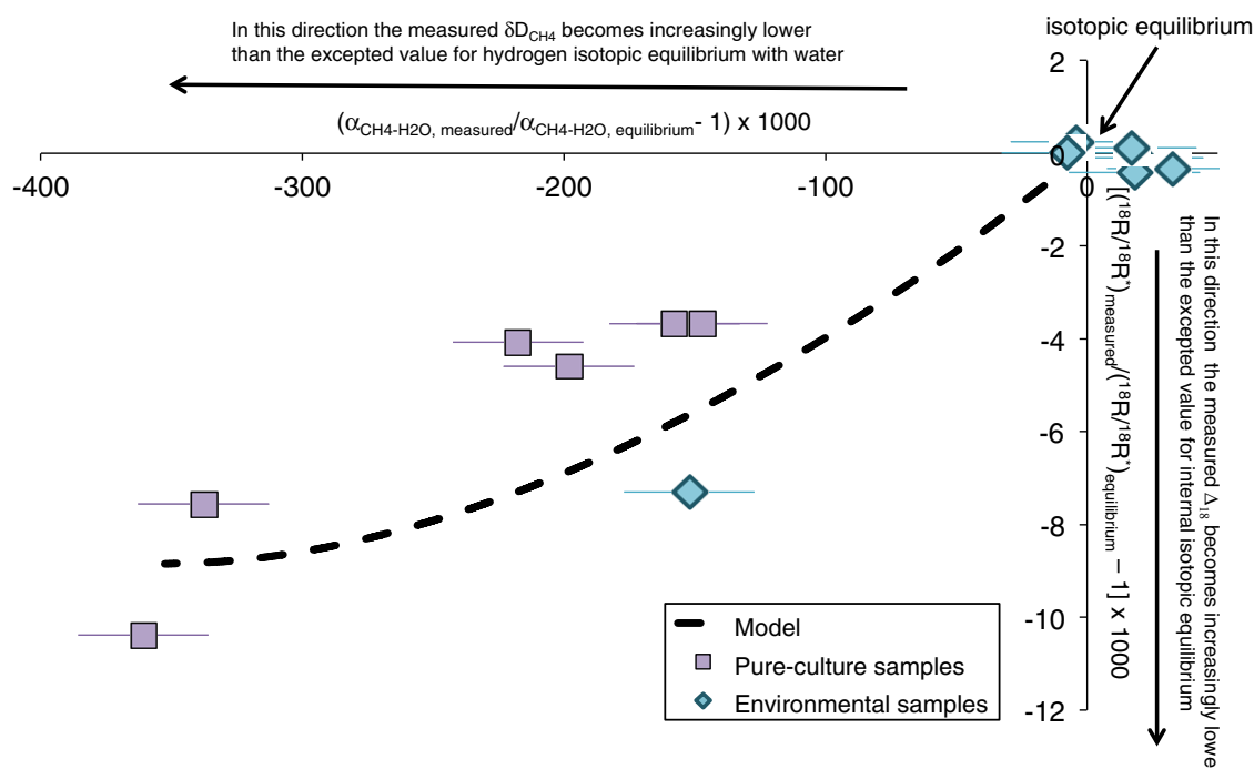
Figure 6: Comparison of measured \Delta_8 values to those expected if the methane formed in internal isotopic equilibrium vs. the difference in measured \mathfrak{D}_{\text{CH}_4} and \mathfrak{D}_{\text{H}_2\text{O,liquid}} values (expressed as a difference in ratios, \alpha_{\text{CH}_4\text{-H}_2\text{O,liquid}} ) compared to that expected for heterogeneous-phase isotopic equilibrium. Deviations in measured \Delta_8 values vs. those expected for equilibrium are represented in this figure through the comparison of ^{18}\text{R}/^{16}\text{R}^* values. As given in equation 1, ^{18}\text{R}/^{16}\text{R}^* = (\Delta_8/1000 + 1) . All samples near the origin, which is the point at which methane is both internally isotopically equilibrated amongst all isotopologues and isotopically equilibrated for hydrogen isotopes with \text{H}_2\text{O} are from marine samples and assumed to have a \mathfrak{D}_{\text{H}_2\text{O,liquid}} = 0\text{‰} . The Caltech pond sample, the only environmental sample not located near the origin, was measured to have a \mathfrak{D}_{\text{H}_2\text{O,liquid}} of -16\text{‰} . One pure-culture sample (the 65\text{ °C} experiment) was measured to have a \mathfrak{D}_{\text{H}_2\text{O,liquid}} = -37.8\text{‰} for the culture media. We assume that this value is the same for all pure-culture experiments. We assume a conservative error for assignment of \mathfrak{D}_{\text{H}_2\text{O,liquid}} of 25\text{‰} to account for our estimations and potential for differences in the \mathfrak{D}_{\text{H}_2\text{O,liquid}} of the environmental waters vs. the intracellular waters of the methanogens. The model describes the isotopic composition of methane formed by methanogens as a function of the reversibility of methyl-coenzyme M reductase. It is described in the text and appendix.
