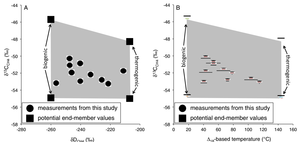
Figure A2: Comparison of potential \delta^{13}\text{C}_{\text{CH}_4} values for the biogenic and thermogenic end members for the mixing model discussed in the main text for A) \delta^{13}\text{C}_{\text{CH}_4} vs. \delta\text{D}_{\text{CH}_4} and B) \delta^{13}\text{C}_{\text{CH}_4} vs. \Delta_{18} -based temperature. The range of biogenic end members were taken from the maximum and minimum \delta^{13}\text{C}_{\text{CH}_4} values for gases from the northern margin of the Antrim shale with \text{C}_1/\text{C}_{2-4} > 500 . The maximum and minimum values are found in Martini et al. (1998). The thermogenic values were found by taking the maximum and minimum range of \delta^{13}\text{C}_{\text{CH}_4} values for gases from the Antrim Shale with \text{C}_1/\text{C}_{2-4} < 100 , including those outside of the northern margin (Martini et al., 1998; Martini et al., 2003). Because the overall potential range of \delta^{13}\text{C}_{\text{CH}_4} values is far larger than total range of \delta^{13}\text{C}_{\text{CH}_4} values observed in this study (3‰), the leverage that the \delta^{13}\text{C}_{\text{CH}_4} values provide for validating the model is low.
