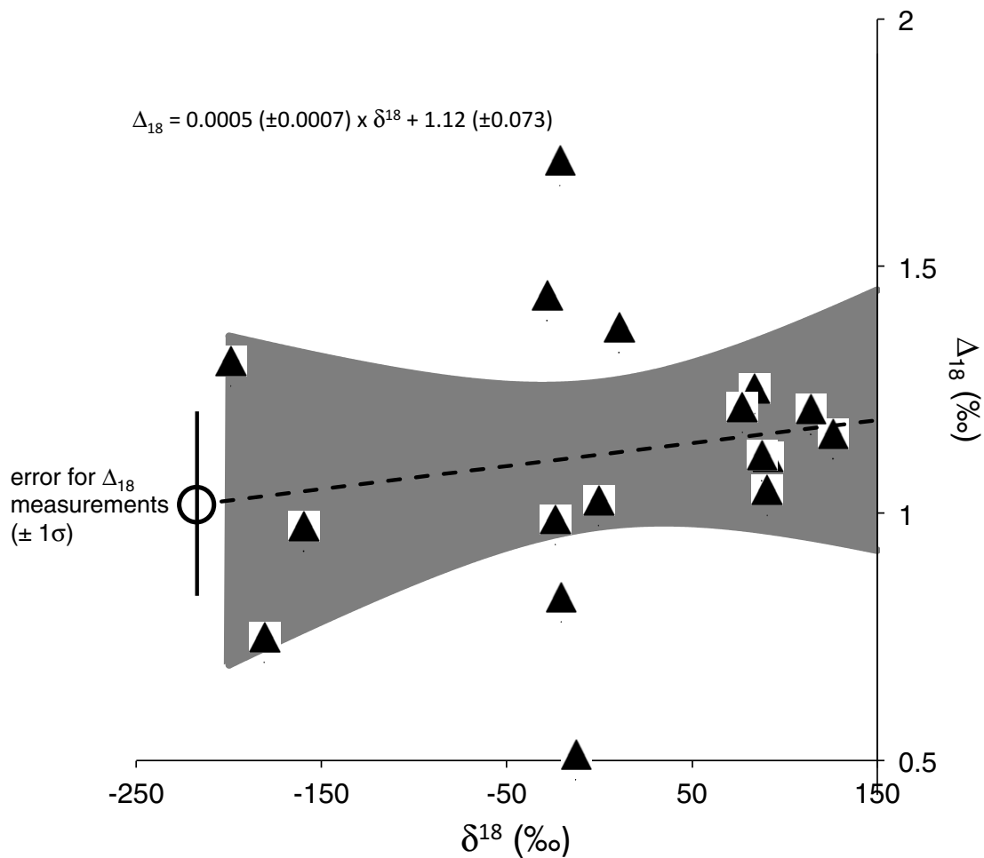
Figure A1: Comparison of measured \Delta_{18} values vs. the average isotopic composition (tracked via \delta^{18} values) for gases equilibrated at 500 °C in the lab using nickel catalysts as described in Stolper et al. (2014c). The \delta^{18} values are dominantly controlled by variations in the \delta D value of the gas. No statistically significant dependence for \Delta_{18} on \delta^{18} is observed: the slope is 0.0005‰ and the 1 \sigma error of the slope is 0.0007‰. Additionally the intercept of the line, 1.12‰ ( \pm 0.073 , 1 \sigma ), is within 1 \sigma of the long-term average value for 500 °C heated gases, 1.06‰. The overall standard deviation of the measured points is 0.28‰, similar to the internal precision of each individual measurement ( \sim 0.25 ‰).
