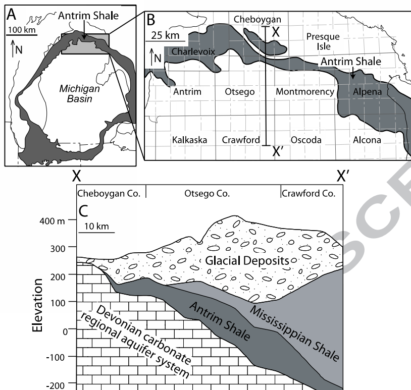
Figure 1: Geological map and cross section of the Antrim Shale. Modified after Martini et al. (1998) and Martini et al. (2008).
