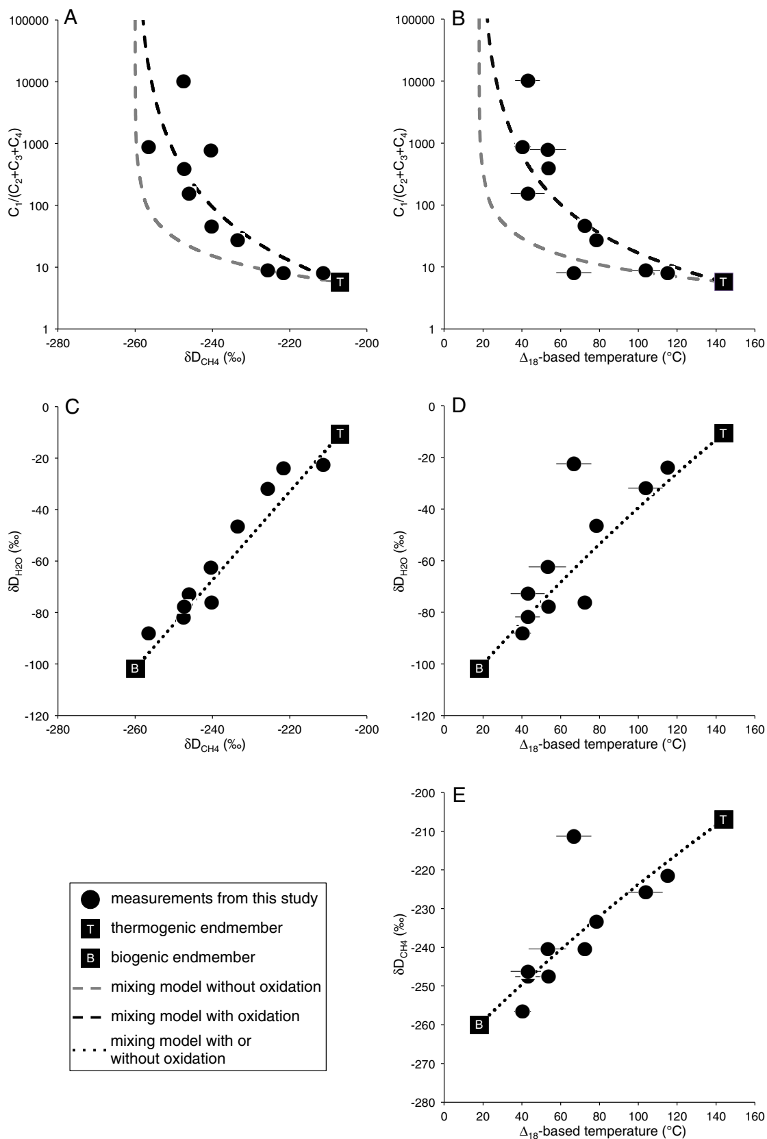
Figure 3: Comparison of the end member mixing models with or without oxidation of C_{2-4} hydrocarbons. Error bars are all 1σ and are not displayed if they are smaller than the symbol. For C, D, and E, both mixing models yields identical results as the
