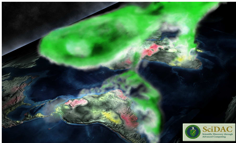
Figure 4. A snapshot from a visualization showing the CO 2 tracer from the land, the product of NEE, being advected in the atmosphere. The colors on the land surface depict NEE (green and yellow for a source, red for a sink). Visualization produced by Jamison Daniel, NCCS/ORNL.
