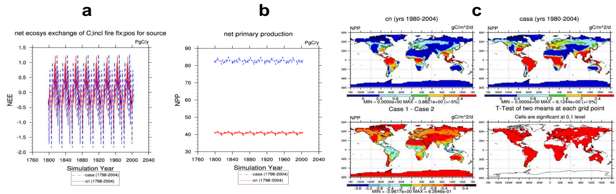
Figure 1. Example model-to-model comparison diagnostics for (a) net ecosystem exchange (NEE), (b) net primary production (NPP), and (c) distribution of annual average NPP (1980–2004) from CLM3-CN and CLM3-CASA' for the control run (Experiment 1.1).
