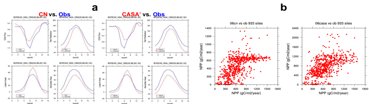
Figure 2. Example model-to-observation comparison diagnostics for (a) surface CO 2 and energy balance at the BOREAS Fluxnet site and (b) NPP at Ecosystem Model-Data Intercomparison (EMDI) sites from CLM3-CN and CLM3-CASA' for the control run (Experiment 1.1).
