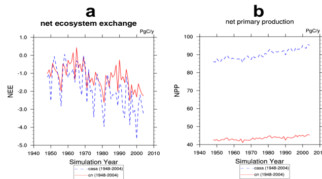
Figure 3. Example model-to-model comparison diagnostics for (a) NEE and (b) NPP for CLM3-CN and CLM3-CASA' from the varying climate, CO 2 , and N deposition run (Experiment 1.4).
