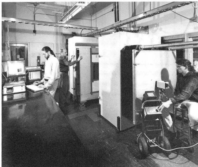
Brent Griffith, left, and Radim Jasek prepare a sample window for testing in the infrared thermography facility. Paul Donohoe, far right, adjusts the infrared camera. The structure attached to the bellows is the newly built room temperature chamber that maintains environmental conditions as constant as those in the refrigerated chamber to its left.
