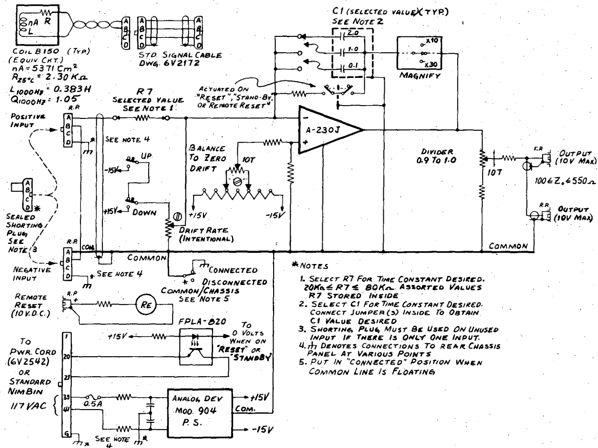
Fig. A III - 1, Electronic Integrator Block Diagram
