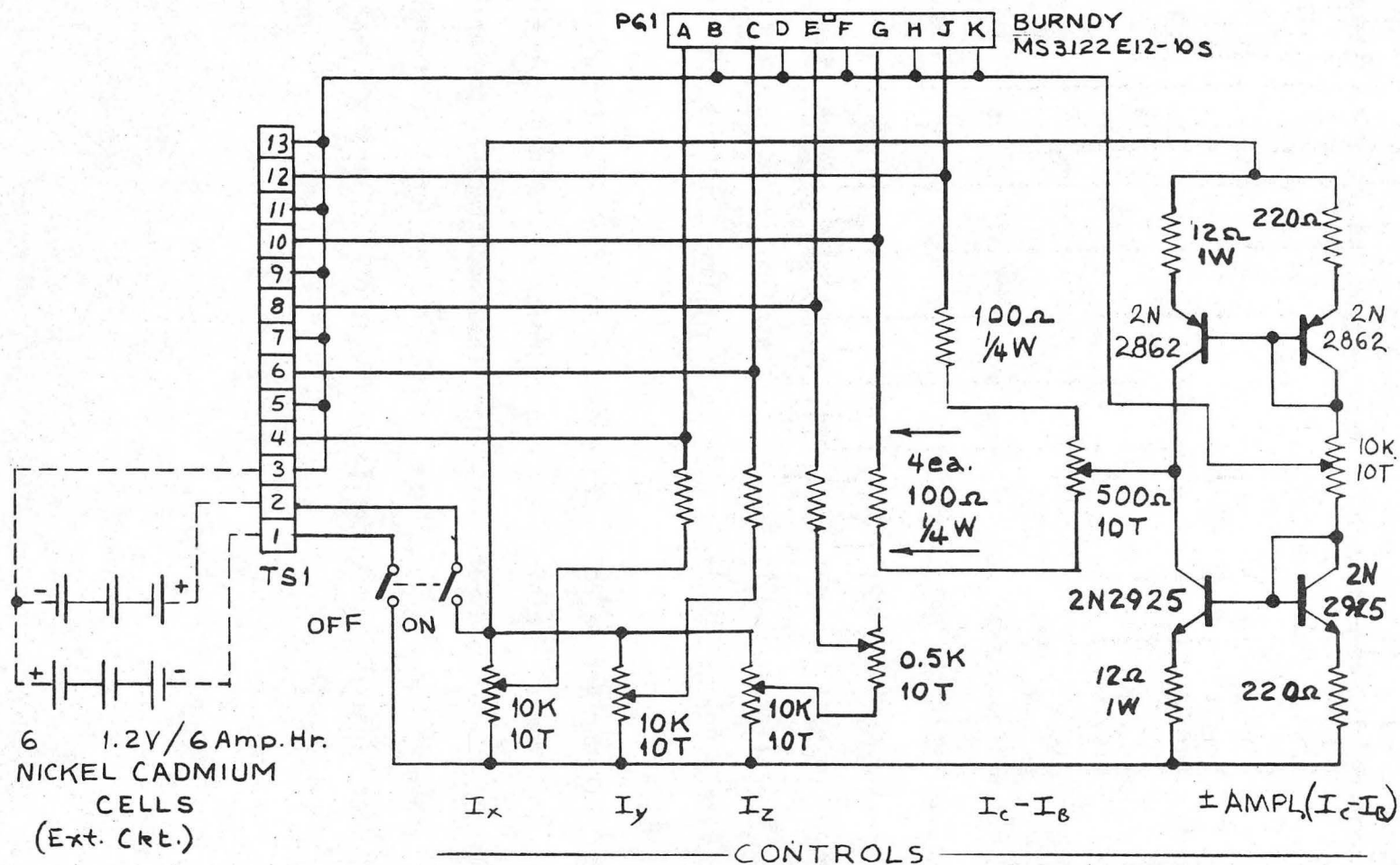
Fig. 11 Current-Controller Schematic
