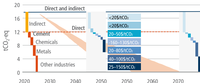
Figure 11.13 | Potentials and costs for zero-carbon mitigation options for industry and basic materials: CIEI – carbon intensity of electricity for indirect emissions; EE – energy efficiency; ME – material efficiency; Circularity – material flows (clinker substituted by coal fly ash, blast furnace slag or other by-products and waste, steel scrap, plastic recycling, etc.); FeedCI – feedstock carbon intensity (hydrogen, biomass, novel cement, natural clinker substitutes); FSW+EI – fuel switch and processes electrification with low-carbon electricity. Ranges for mitigation options are shown based on bottom-up studies for grouped technologies packages, not for single technologies. In circles, contribution to mitigation from technologies based on their readiness are shown for 2050 (2040) and 2070. Direct emissions include fuel combustion and process emissions. Indirect emissions include emissions attributed to consumed electricity and purchased heat. For basic chemicals only methanol, ammonia and high-value chemicals are considered. The total for industry doesn't include emissions from waste. Base values for 2020 for direct and indirect emissions were calculated using 2019 GHG emission data (Crippa et al. 2021) and data for materials production from World Steel Association (2020a) and IEA (2021d). Negative mitigation costs for some options like Circularity are not reflected. Data from sources: Pauliuk et al. (2013a); Fawkes et al. (2016); WBCSD (2016); Bazzanella and Ausfelder (2017); IEA (2018a, 2019b,g,h, 2020a,c, 2021a); Lehne and Preston (2018); Scrivener et al. (2018); EUROFER (2019); Friedmann et al. (2019); Material Economics (2019); Sandalow et al. (2019); CAT (2020); CEMBUREAU (2020); Gielen et al. (2020); Habert et al. (2020); World Steel Association (2020b); Bataille (2020a); GCCA (2021a); and Saygin and Gielen (2021).
