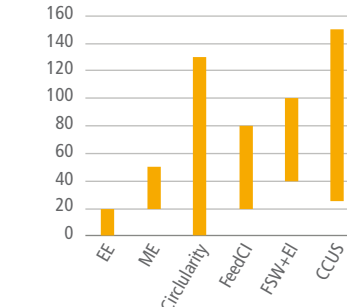
Figure 11.13 | Potentials and costs for zero-carbon mitigation options for industry and basic materials: CIEI – carbon intensity of electricity for indirect emissions; EE – energy efficiency; ME – material efficiency; Circularity – material flows (clinker substituted by coal fly ash, blast furnace slag or other by-products and waste, steel scrap, plastic recycling, etc.); FeedCI – feedstock carbon intensity (hydrogen, biomass, novel cement, natural clinker substitutes); FSW+EI – fuel switch and processes electrification with low-carbon electricity. Ranges for mitigation options are shown based on bottom-up studies for grouped technologies packages, not for single technologies. In circles, contribution to mitigation from technologies based on their readiness are shown for 2050 (2040) and 2070. Direct emissions include fuel combustion and process emissions. Indirect emissions include emissions attributed to consumed electricity and purchased heat. For basic chemicals only methanol, ammonia and high-value chemicals are considered. The total for industry doesn't include emissions from waste. Base values for 2020 for direct and indirect emissions were calculated using 2019 GHG emission data (Crippa et al. 2021) and data for materials production from World Steel Association (2020a) and IEA (2021d). Negative mitigation costs for some options like Circularity are not reflected. Data from sources: Pauliuk et al. (2013a); Fawkes et al. (2016); WBCSD (2016); Bazzanella and Ausfelder (2017); IEA (2018a, 2019b,g,h, 2020a,c, 2021a); Lehne and Preston (2018); Scrivener et al. (2018); EUROFER (2019); Friedmann et al. (2019); Material Economics (2019); Sandalow et al. (2019); CAT (2020); CEMBUREAU (2020); Gielen et al. (2020); Habert et al. (2020); World Steel Association (2020b); Bataille (2020a); GCCA (2021a); and Saygin and Gielen (2021).
