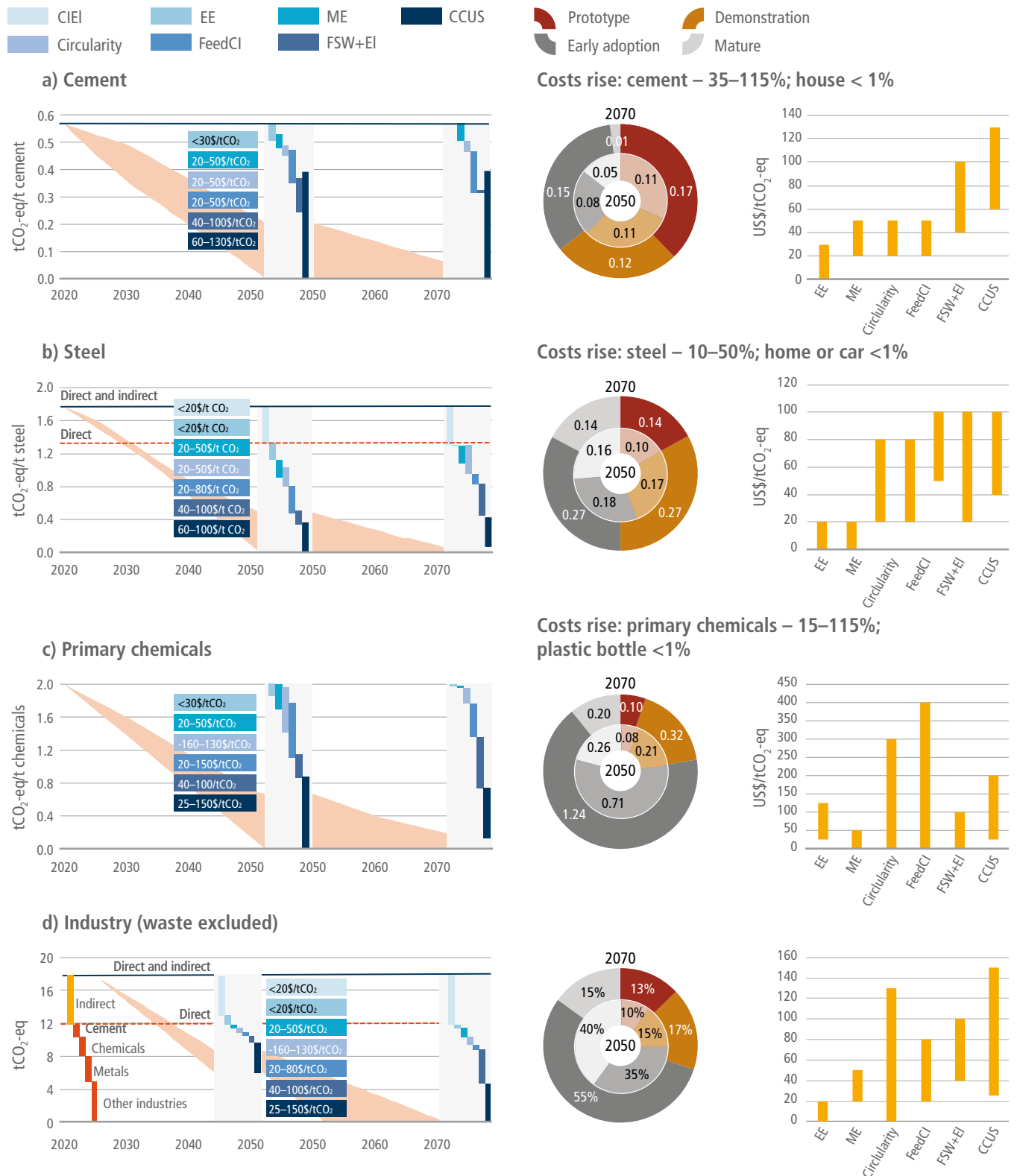
Figure 11.13 | Potentials and costs for zero-carbon mitigation options for industry and basic materials: CIEL – carbon intensity of electricity for indirect emissions; EE – energy efficiency; ME – material efficiency; Circularity – material flows (clinker substituted by coal fly ash, blast furnace slag or other by-products and waste, steel scrap, plastic recycling, etc.); FeedCI – feedstock carbon intensity (hydrogen, biomass, novel cement, natural clinker substitutes); FSW+EI – fuel switch and processes electrification with low-carbon electricity. Ranges for mitigation options are shown based on bottom-up studies for grouped technologies packages, not for single technologies. In circles, contribution to mitigation from technologies based on their readiness are shown for 2050 (2040) and 2070. Direct emissions include fuel combustion and process emissions. Indirect emissions include emissions attributed to consumed electricity and purchased heat. For basic chemicals only methanol, ammonia and high-value chemicals are considered. The total for industry doesn't include emissions from waste. Base values for 2020 for direct and indirect emissions were calculated using 2019 GHG emission data (Crippa et al. 2021) and data for materials production from World Steel Association (2020a) and IEA (2021d). Negative mitigation costs for some options like Circularity are not reflected. Data from sources: Pauliuk et al. (2013a); Fawkes et al. (2016); WBCSD (2016); Bazzanella and Ausfelder (2017); IEA (2018a, 2019b,g,h, 2020a,c, 2021a); Lehne and Preston (2018); Scrivener et al. (2018); EUROFER (2019); Friedmann et al. (2019); Material Economics (2019); Sandalow et al. (2019); CAT (2020); CEMBUREAU (2020); Gielen et al. (2020); Habert et al. (2020); World Steel Association (2020b); Bataille (2020a); GCCA (2021a); and Saygin and Gielen (2021).
