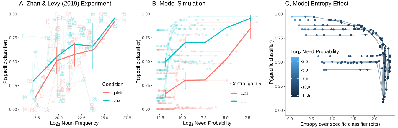
Figure 3: Experimental data and model simulations for Mandarin classifier choice. A. Empirical proportions of specific classifier use in a picture naming task, by noun frequency and timing condition. Solid lines show empirical means for 5 bins of noun frequency and error bars are 95% confidence intervals. Transparent lines link datapoints for individual classifiers. B. Model probability to use a specific classifier as a function of need probability and control gain, in a toy language with 200 Zipf-distributed nouns and 10 specific classifiers distributed randomly among them. C. Model probability to use the specific classifier as a function of the entropy over specific classifiers given the communicative goal, for control gain \alpha = 1.1 .
