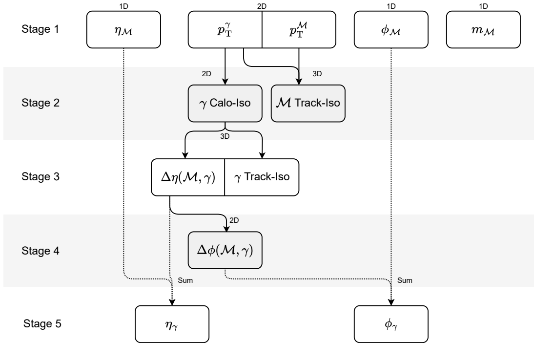
Figure 2: A schematic diagram showing the stages of the background model used for the analyses presented. Variables are drawn using a combination of 1D, 2D and 3D histograms in order to retain the correlations between them. Solid arrows correspond to where variables have been sampled from the previous stage. Dashed arrows correspond to where previous variables have been summed to produce a new variable. Joined cells indicate variables that have been simultaneously sampled from the previous stage.
