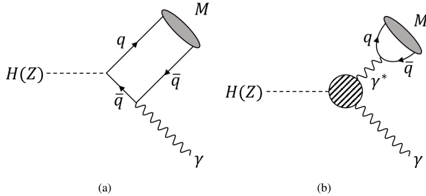
Figure 1: Feynman diagrams for the (a) direct and (b) indirect contributions to the H/Z \rightarrow M\gamma decays.
