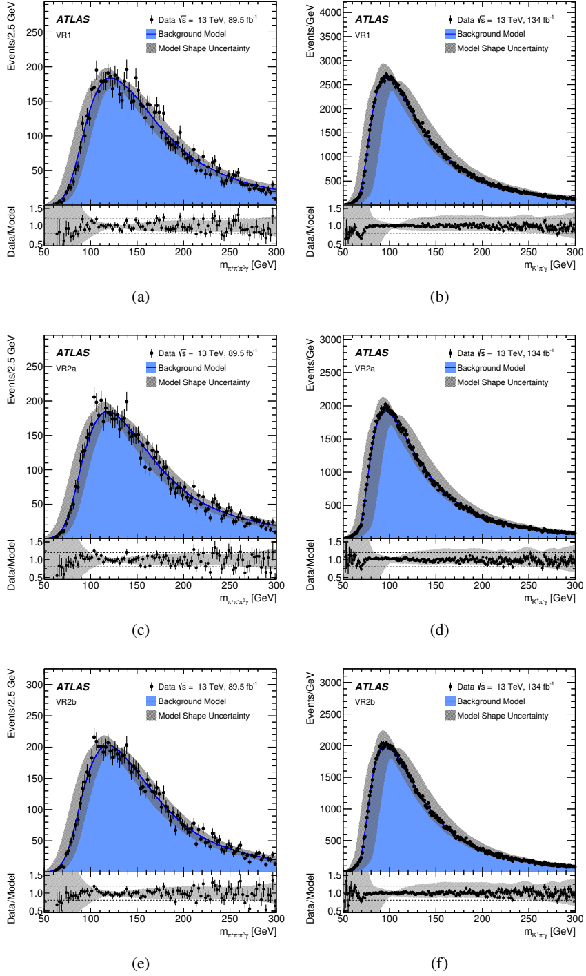
Figure 3: Distributions of ((a), (c), (e)) m_{\pi\pi\pi\gamma} and ((b), (d), (f)) m_{K\pi\gamma} in data compared with the prediction of the background model for the VR1, VR2a and VR2b validation regions. The background model is normalised to the observed number of events within the region shown. The uncertainty band corresponds to the uncertainty envelope derived from variations in the background modelling procedure, described in Section 5. The ratio of the data to the background model is shown below the distributions.
