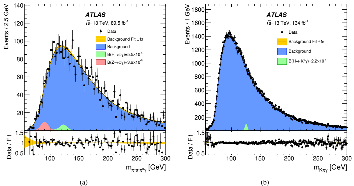
Figure 4: Background-only fits performed in the signal region for the (a) \omega\gamma and (b) K^*\gamma final states. The branching fraction of each of the signals is set to the observed 95% CL upper limit. The yellow band represents the uncertainty in the fit arising from the constrained background shape systematic uncertainties.
