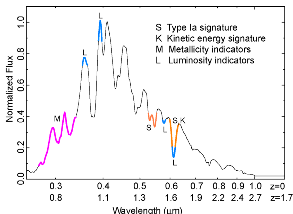
Figure 2. Type Ia spectrum at maximum brightness showing critical features. The horizontal axis shows wavelengths for z=0 and z=1.7 .
