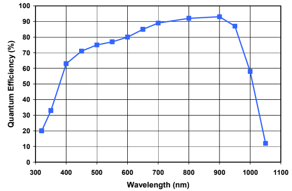
Figure 7. Quantum efficiency for a 300 \mu\text{m} thick LBNL CCD with a simple InTiO/SiO 2 AR coating.
