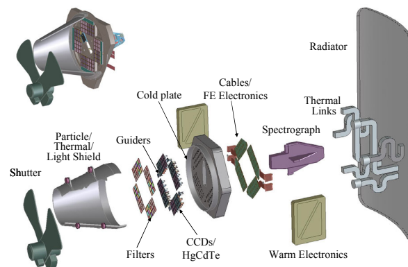
Figure 4. Exploded view of the focal plane region. Shown is an imager using CCDs and HgCdTe sensors and discrete filters.
