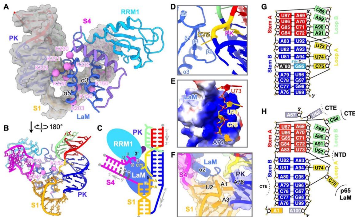
Figure 5: p65 \alpha N-LaM binds the TER 5'-end, UUUU-3'-OH, and PK.
