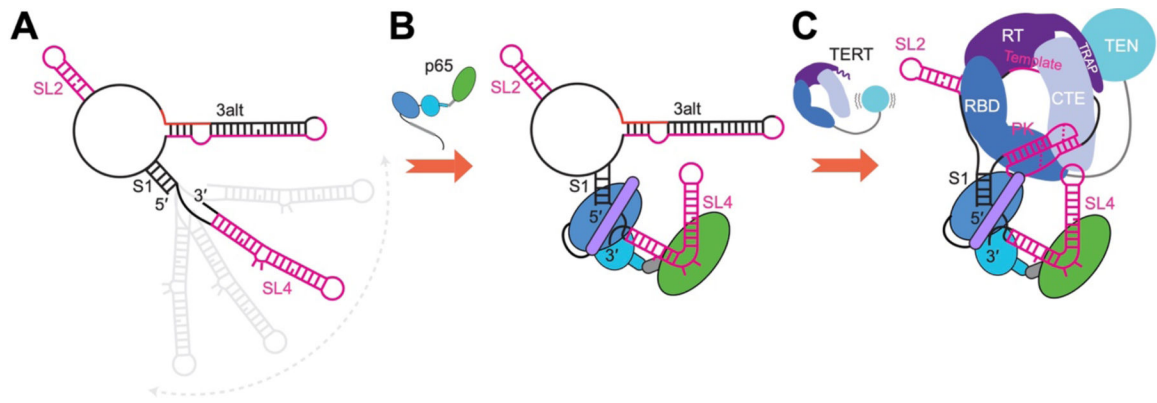
Figure 7: Steps in p65–TER–TERT assembly.
