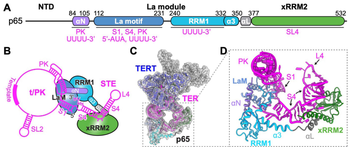
Figure 1: Structure of p65-TER complex in Tetrahymena telomerase.
