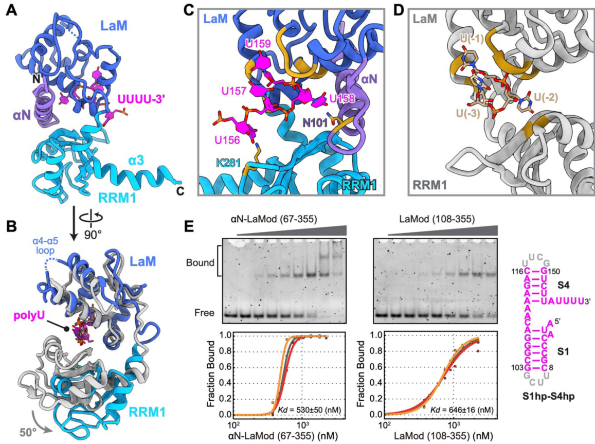
Figure 4: Interactions between p65 and the polyU tail of TER.
