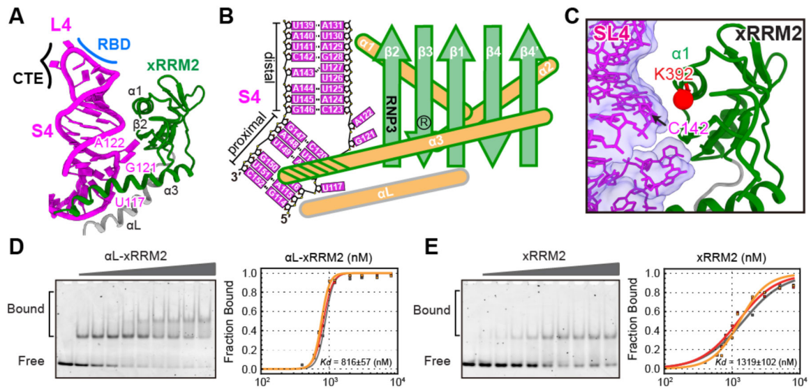
Figure 6: Interactions between p65 \alpha L-xRRM2 and SL4.
