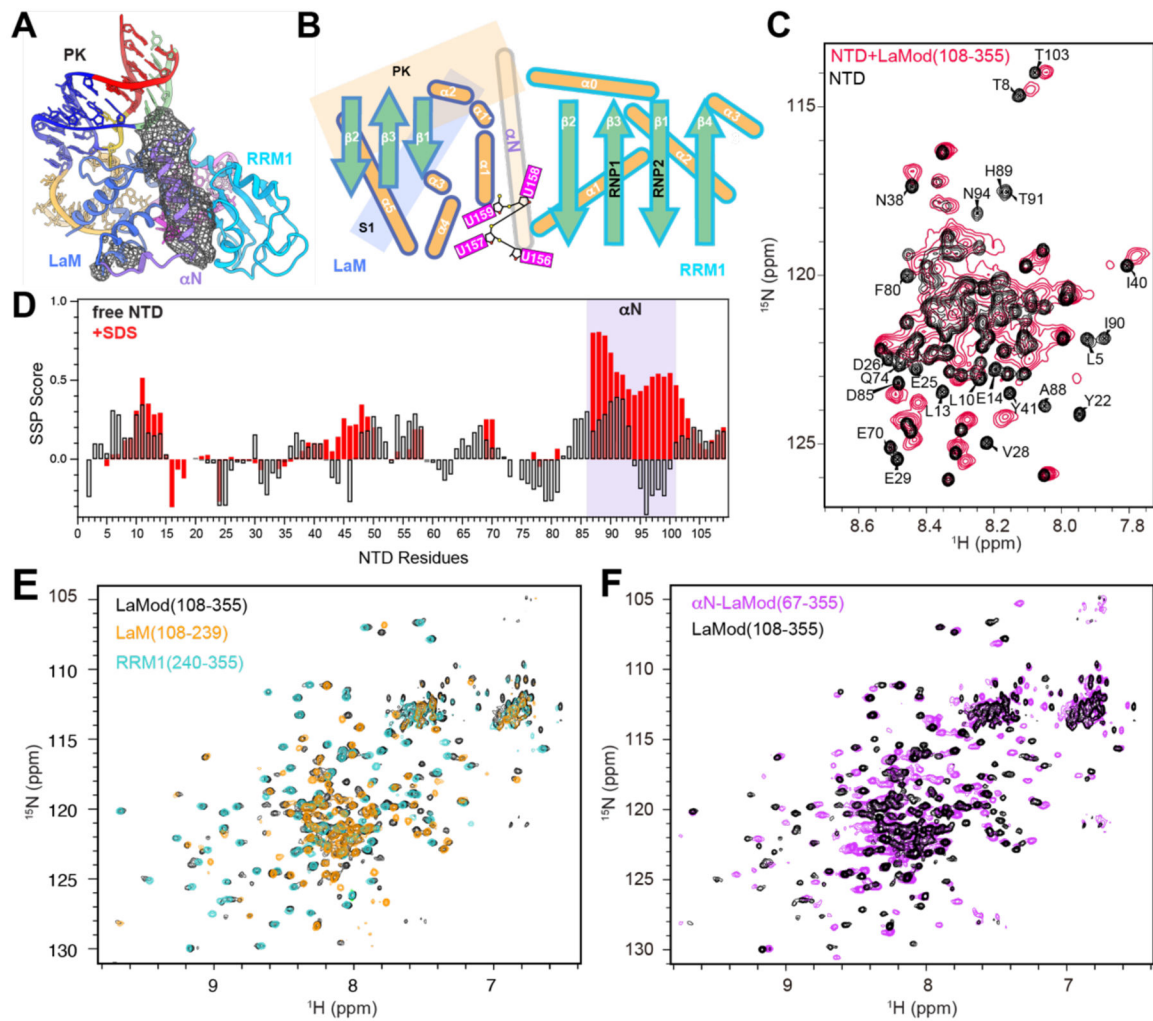
Figure 3: p65 NTD \alpha N binds the La module
