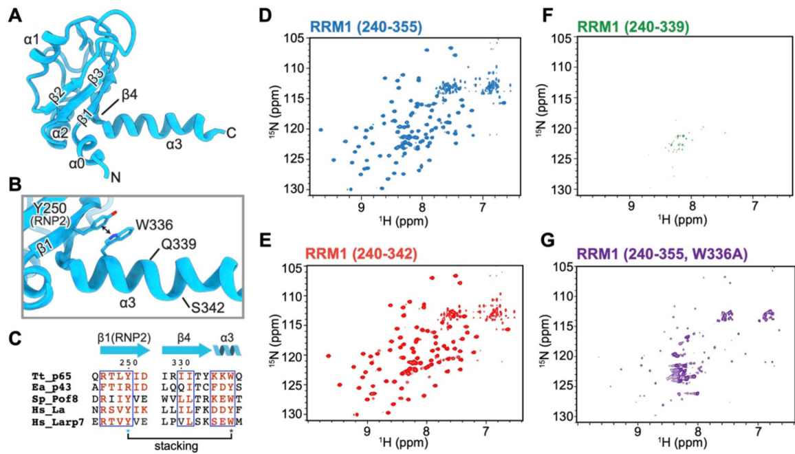
Figure 2: Structure and stability of La Module RRM1.
