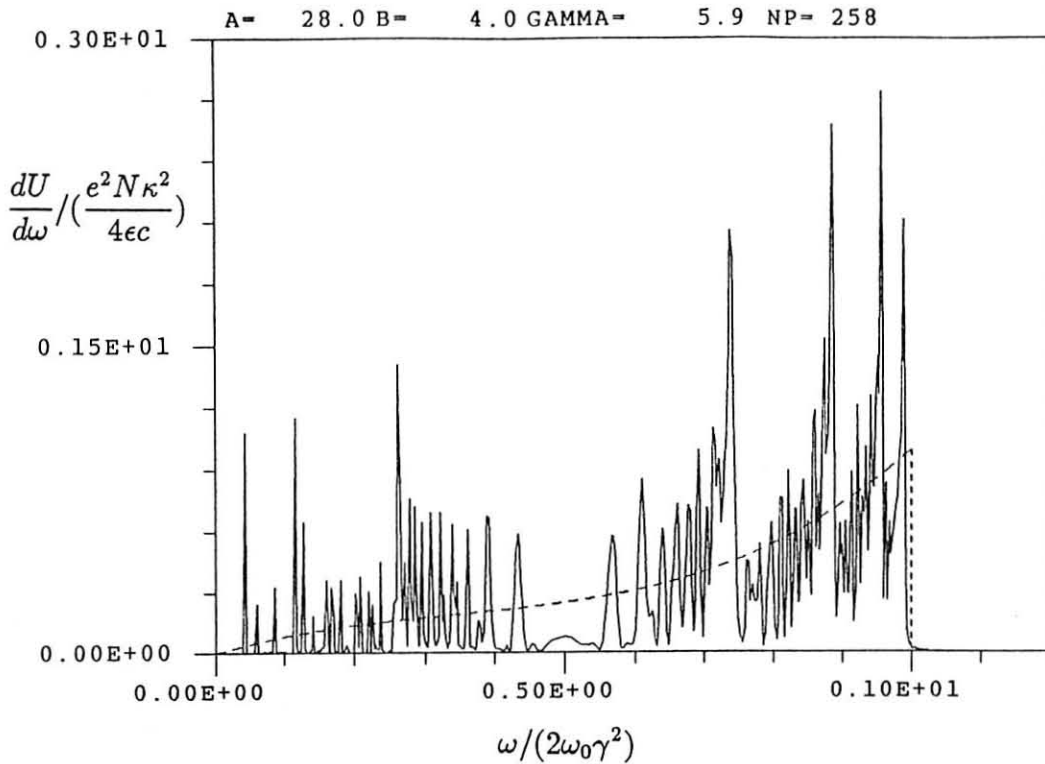
Figure 1: Radiated energy spectrum of UCSB FEL. The free space result is denoted by the broken line.
