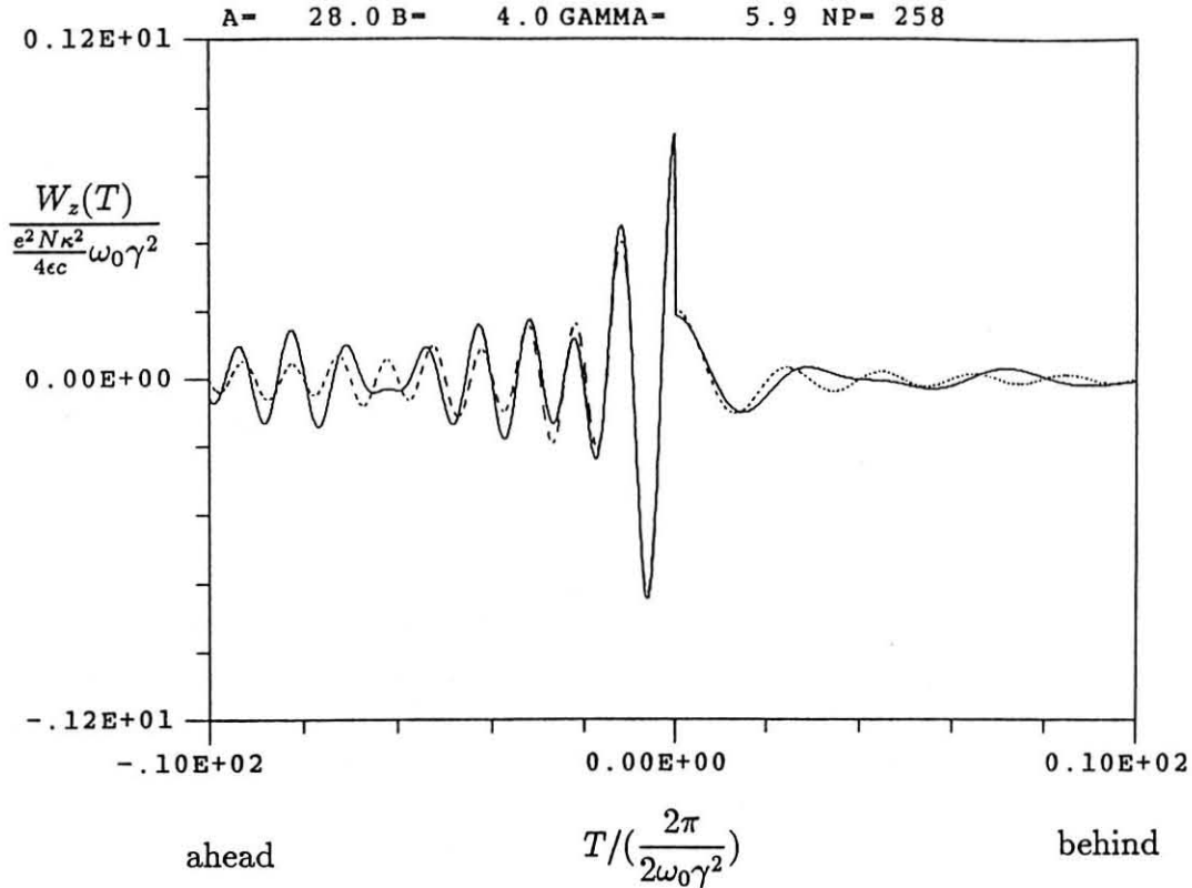
Figure 2: Longitudinal wake function of the UCSB FEL.
