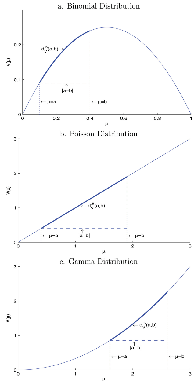
Figure 1. The variance functions of binomial, Poisson and gamma distributions. The length of the thick line is \sqrt{d_V^5(a, b)} , and the length of the dashed line is |a - b| . These two lengths may differ dramatically in binomial and gamma distributions.
