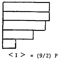
Figure 5. Poisson Distributed Interarrival Times
