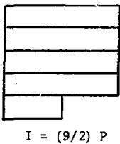
Figure 4. Uniformly Distributed Interarrival Times
