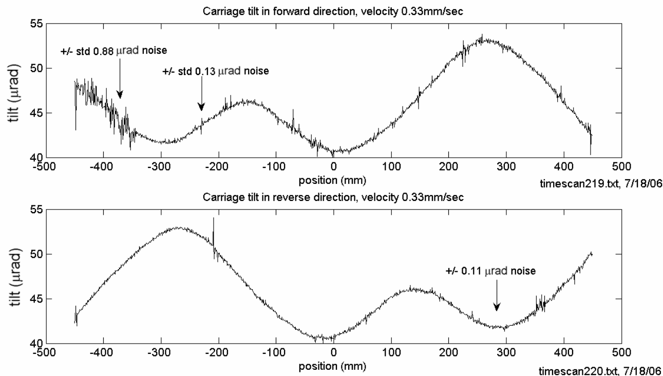
Figure 5: Tiltmeter output for DLTP setup in forward (top) and reverse (bottom) movement direction. The areas of fluctuation are related to small changes in acceleration likely due to the balance of the beam, loads on the picomotors, and motor tuning parameters.
