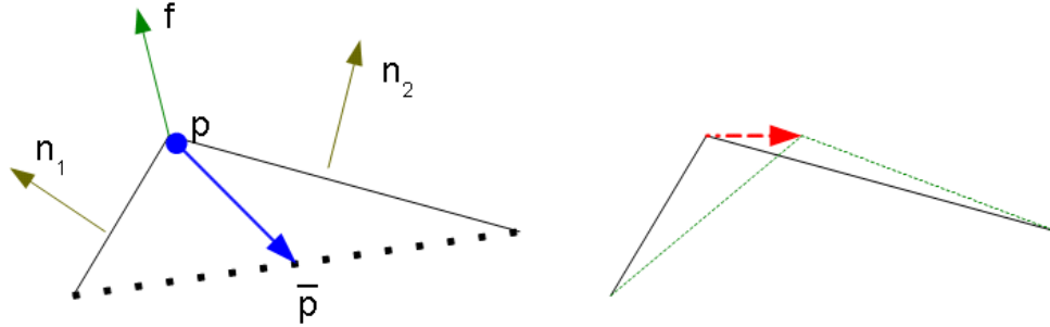
Figure 1.3: An illustration of the force vectors involved in the Active Interface Reconstruction algorithm from 1.4. On the left, the blue arrow is the smoothing vector, while the green is the volume correction vector. On the right, the red is the resultant, and the new interface is drawn in green.
