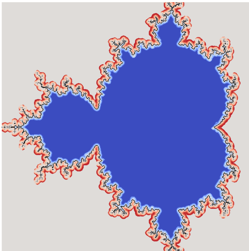
Figure 5.7: Mandelbrot. Reconstruction of the Mandelbrot set truncated at 20 iterations, i.e. the set of points z_0 \in \mathbb{C} such that |f \circ f \circ \cdots f(z_0)| < 2 , the number of compositions being twenty, and f(z) = z^2 + z_0 . The reconstruction was allowed to form islands due to pinch-off.
