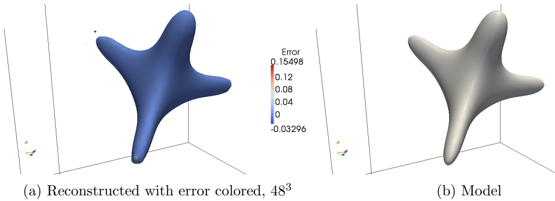
Figure 5.19: Deltoid-like. Reconstruction of a deltoid-like object, defined as 0 = r^4 + 18a^2r^2 - 27a^4 - 8a(x^3 + y^3 - 3xz^2) - 1, a = \frac{1}{2} . Reconstruction is very accurate away from the tips. The tips, though smooth, have curvature quite high and end up truncated.
