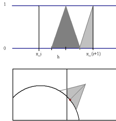
Figure 4.7: Illustration of the the computation of gradient functionals. On top, in the 1D function graph case; on bottom, the extension to the level set case.
