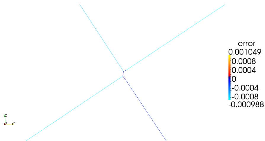
Figure 5.10: Quadruple point. Close up of quadruple point. The reconstructed topology is that of two nearby triple points.
