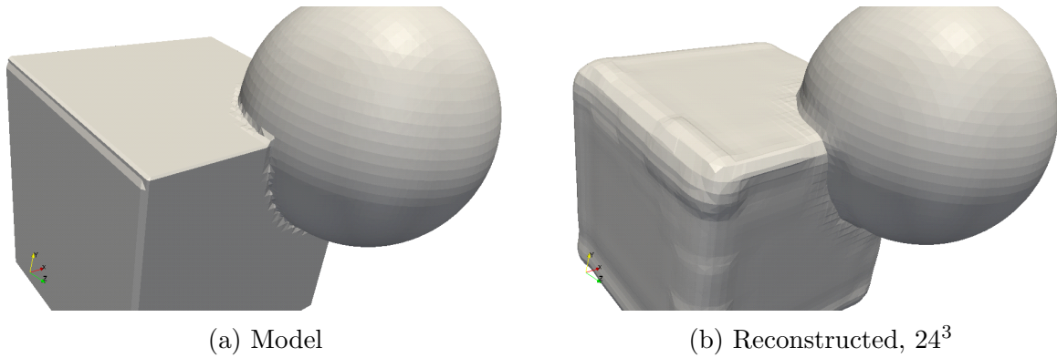
Figure 5.25: Sphere/Box. See [3]. Within [0, 1]^3 , the sphere is centered at (0.6, 0.6, 0.6) , with radius 0.2; the cube is from (0.2, 0.2, 0.2) to (0.6, 0.6, 0.6) , and is only defined where the sphere is not. The third material is empty space. The average error reported is over 1%, however, as we can see, most of the error is in the reconstruction of the cube itself. The sphere is reconstructed as a sphere, and the junction between the cube and sphere is a smooth curve.
