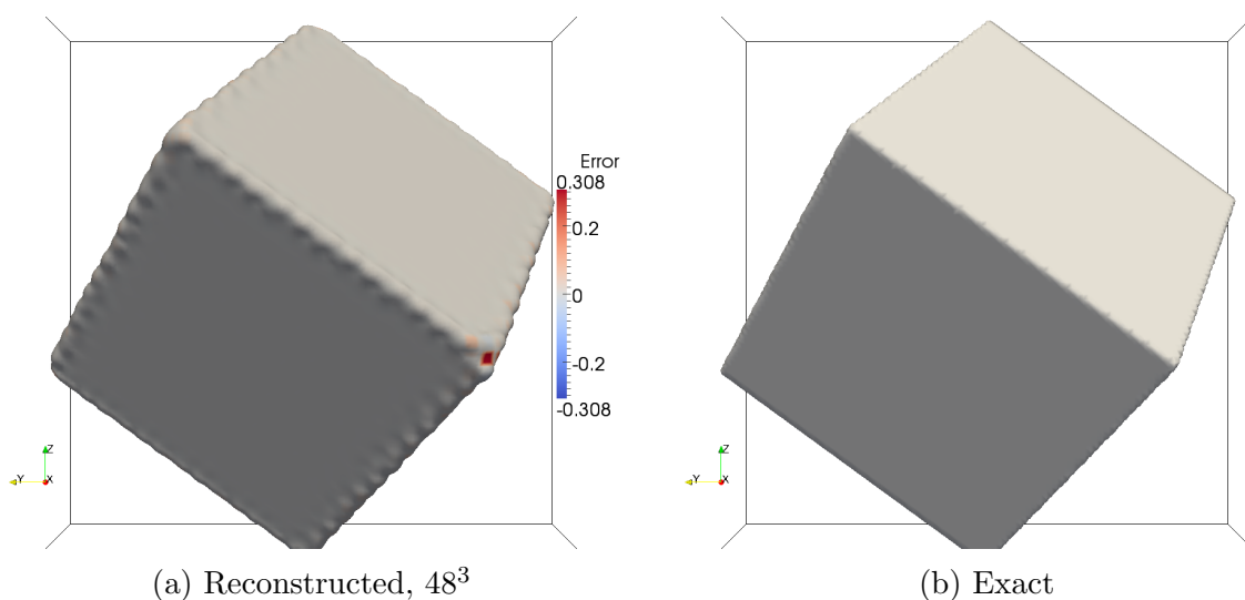
Figure 5.22: Cube. A cube, with side length 3, on the interval [-3, 3] . The cube is rotated about the origin by the angles (\pi/5, \pi/5, 0) , as done previously. The edges have the same aliasing effect as seen in Chapter 3.
