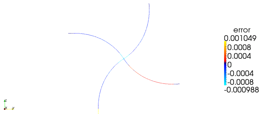
Figure 5.9: Quadruple point. First defined on the interval [-1, 1] , as rays at angles 0, \pi/2, \pi, 3\pi/2 from the origin. The swirl is done by the tranform (r, \theta) \mapsto (r, \theta - r\frac{\pi}{6}) .
