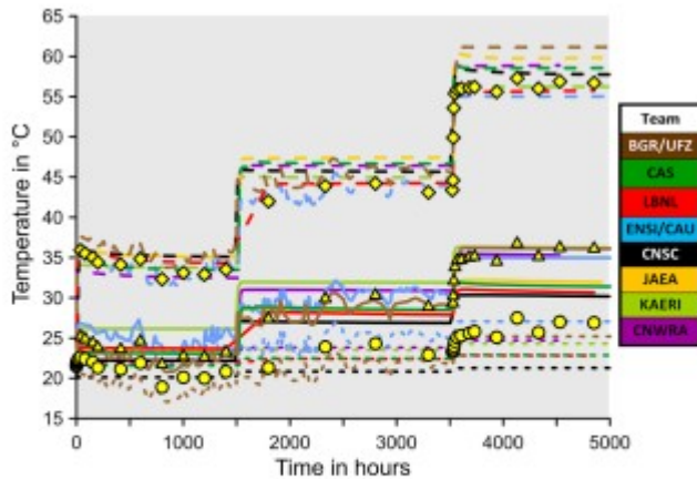
Fig. 9 Measured and modelled temperature at Sensor 1 (circles and dotted lines), at Sensor 2 (triangles and full lines) and at Sensor 3 (diamonds and dashed lines) during the heating phase (light grey area)
