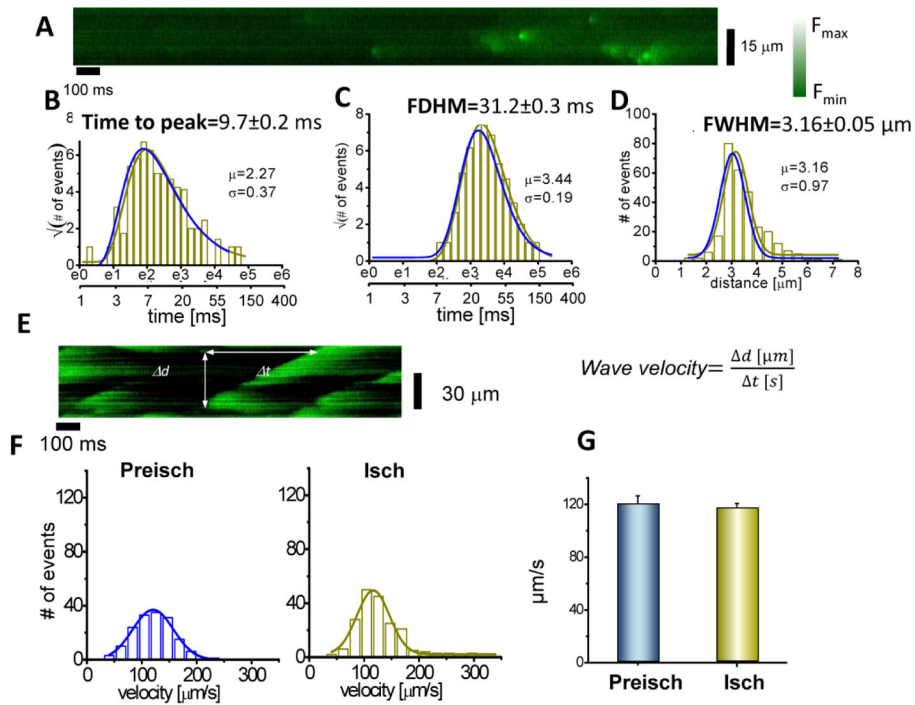
Figure 4. Ca 2+ spark and waves are similar in ischemia and in preischemia
