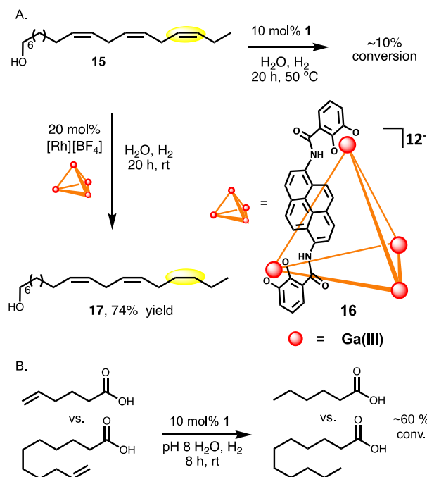
Figure 5. (a) Minor conversion of 15 was observed using catalyst 1 . Catalyst 16 provides good conversion of 15 to the singly hydrogenated product 17 . (b) Competition between two acids with different alkane lengths show similar conversion, indicating remote group does not affect reactivity.
