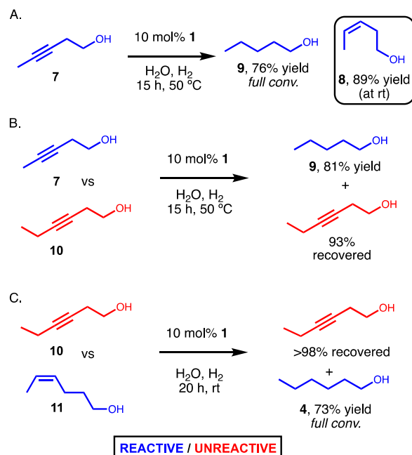
Figure 3. Supramolecular supported catalyst selectively hydrogenates alkynes based on size-exclusion. (a) Hydrogenation of methyl-alkyne 7 provide cis -alkene 8 at room temperature and heating provides fully hydrogenated 9 . (b) Competition between methyl- and ethyl-alkyne ( 7 and 10 respectively) provide size-selective hydrogenation of 7 and full recovery of 10 . (c) Methyl-alkene 11 was selectively hydrogenated with full recovery of ethyl-alkyne 10 .
