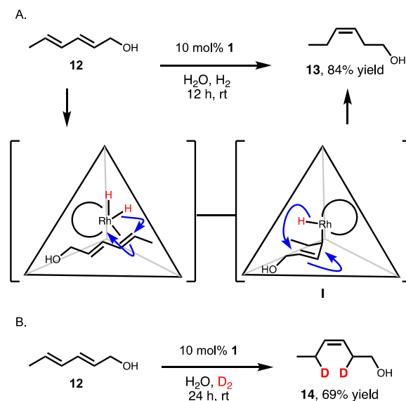
Figure 4. (a) Supramolecular host supported hydrogenation of trans,trans -2,4-hexadiene-1-ol ( 12 ) to cis -3-hexen-1-ol ( 13 ). (b) Under di-deuterium conditions, selective 1,4-addition was observed to yield a single major isomer 14 .
