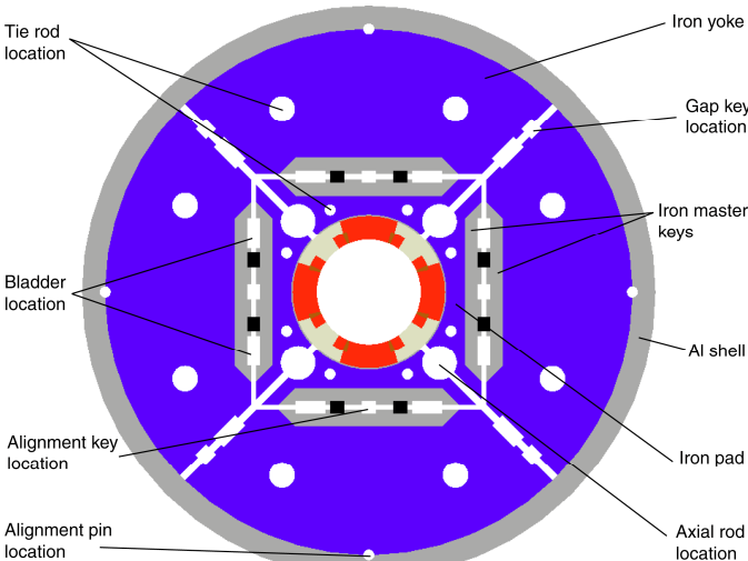
Fig. 2. LQS01 cross-section.
