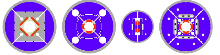
Fig. 1. LARP shell-based (S) magnets (from left to right in chronological order and in scale): Subscale Quadrupole SQ (2004), Technology Quadrupole TQS (2005), Long Racetrack LRS (2006), and Long Quadrupole LQS (under development).
