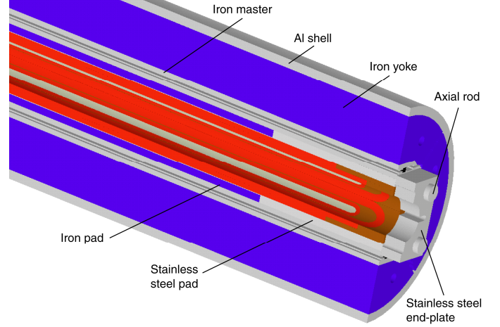
Fig. 3. LQS01 end design.
