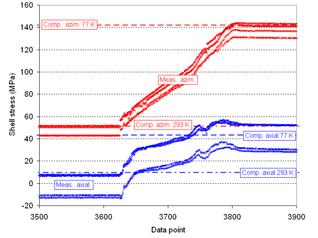
Fig. 12. Gauge measurements of azimuthal and axial stress (MPa) in the shell (markers) and comparison with computed values (dashed lines).
