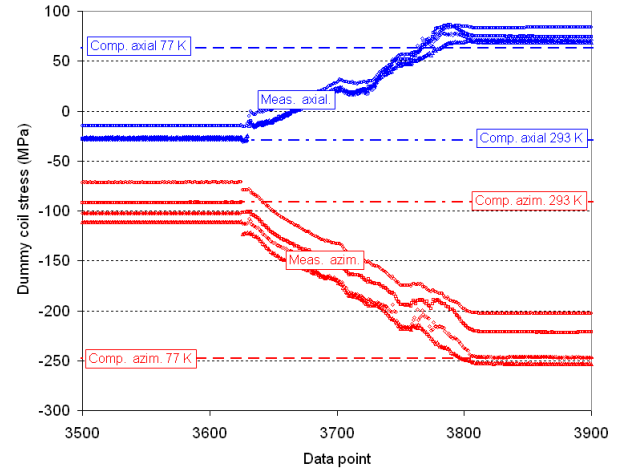
Fig. 13. Gauge measurements of azimuthal and axial stress (MPa) in the dummy coils (markers) and comparison with computed values (dashed lines).
