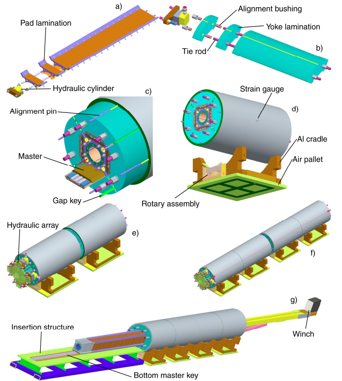
Fig. 10. Assembly steps: pad lamination stacking (a); yoke lamination stacking (b); assembly of first segment (c); segment support system (d); connection of two segments (e); connection of four segments (f); insertion of full-length coil-pack.
