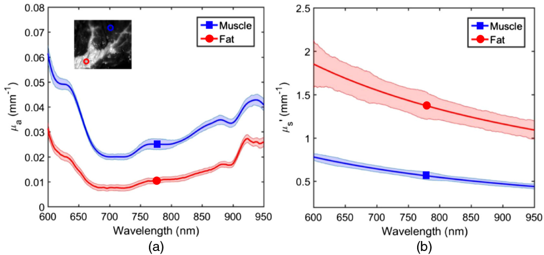
Fig. 6 Plot of (a) bulk \mu_a spectra and (b) \mu_s' spectra at two ROIs (3 mm × 3 mm): fat (red) and muscle (blue).
