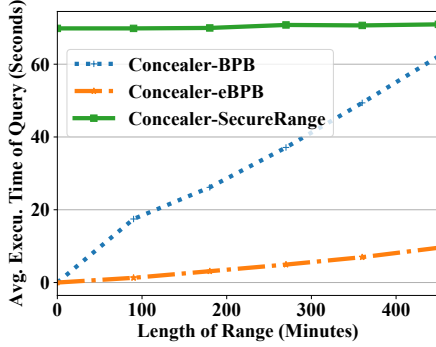
Figure 5: Exp 3: Range length impact.
