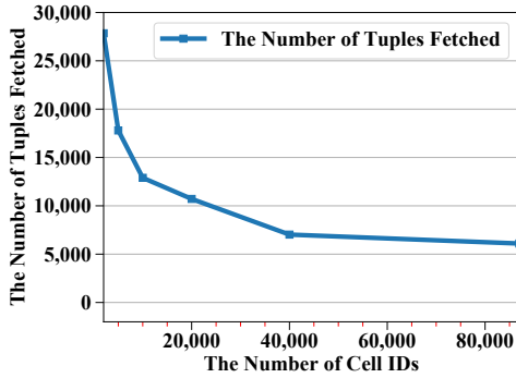
Figure 7: Exp 7: Impact of # cells-ids.
