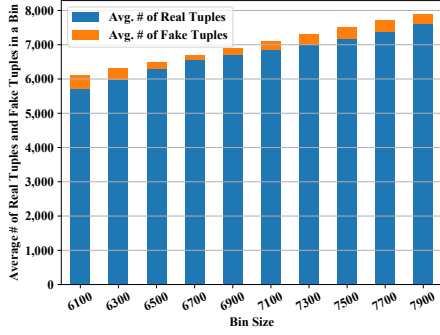
Figure 6: Exp 6: Impact of bin-size.
