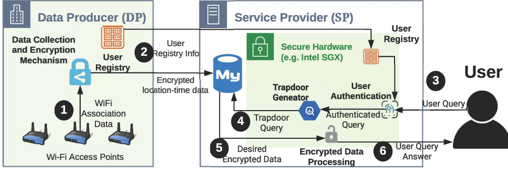
Figure 1: CONCEALER model.
