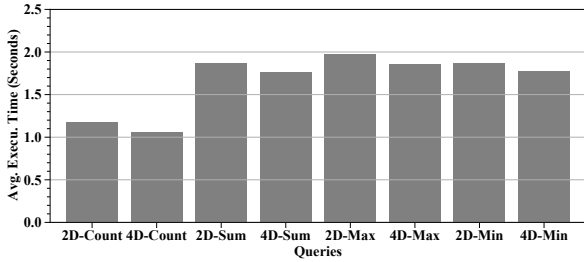
Figure 8: Exp 8: Query performance on TPC-H data.
