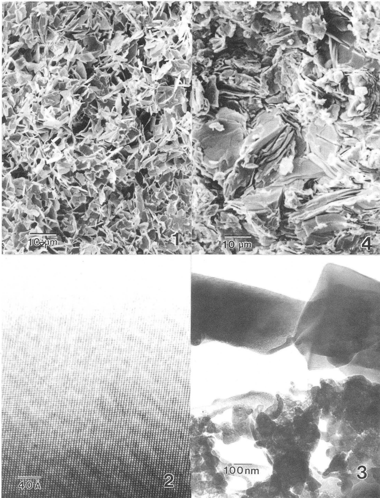
FIG. 1. -- Scanning electron image of porous microstructure in sintered pellet of BiCaSrCuO. FIG. 2. -- High Resolution TEM image from crushed specimen, showing (001) cleavage. FIG. 3. -- TEM image of ion milling damage in porous material. FIG. 4. -- Scanning electron image of sintered BiCaSrCuO pellet with additional processing.
