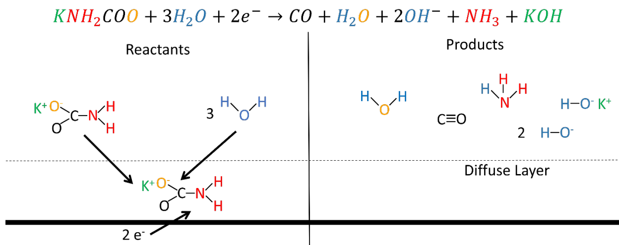
Figure 4: A worked example of the overall carbamate reduction using a water proton source. Color coding is provided to aid the reader in determining how the atoms rearrange. The capture agent RH (NH 3 ) is shown in red, the proton source XH (H 2 O) is shown in blue and the resultant salt KX (KOH) is shown in green. The O of the carbamate are coded orange and black to shown that the
