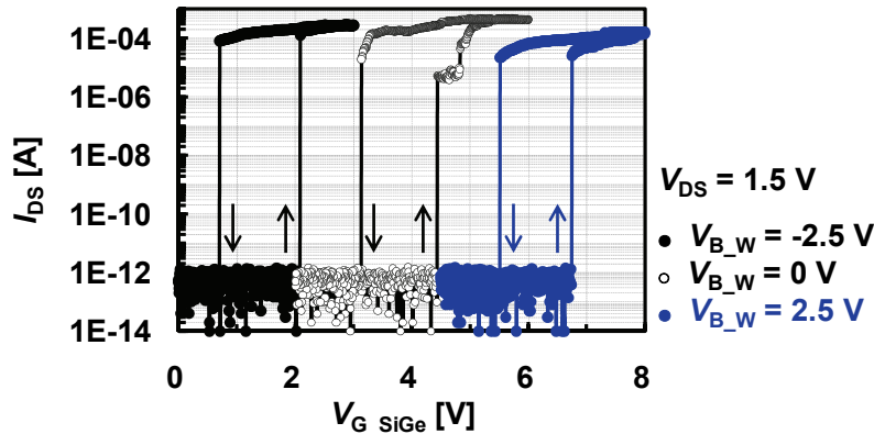
Figure 2.5: Measured I_{DS} - V_G characteristics of a fabricated 4-T relay at room temperature under N 2 purge at atmospheric pressure, for various body biases. Zero off -state leakage and abrupt switching behavior (less than 1 mV/decade) are observed. The on -state resistance ( R_{ON} ) values are 5.5 k \Omega , 3.3 k \Omega , and 9.1 k \Omega at V_{G, SiGe} = 1.2 \cdot V_{PI} for V_{B, W} of -2.5 V, 0 V, and 2.5 V, respectively. The hysteretic switching behavior is due to pull-in mode operation (because T_{CONTACT} > T_{ACT} / 3 ) as well as surface adhesion forces which increase with decreasing R_{ON} . The variation in R_{ON} is partly attributed to oxidation of the channel and source/drain electrode surfaces over time. The measurements were made firstly for V_{B, W} = 0 V, then for V_{B, W} = -2.5 V, finally for V_{B, W} = 2.5 V.
