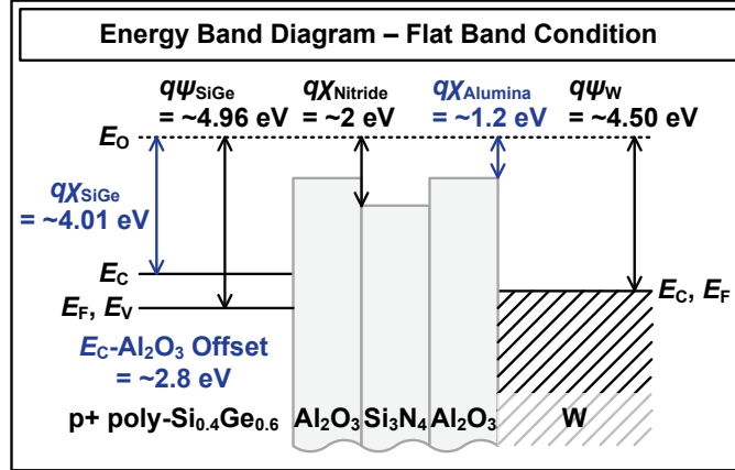
Figure 3.6: Energy band diagram for a SONOS-type memory 4-T relay under flat band condition. Si 3 N 4 is used as a charge trap layer (less than 10 nm), and Al 2 O 3 is used as tunneling (less than 5 nm, c.f. mean free path of electrons in the oxide = 3.2 nm [15]) and blocking (less than 15 nm) layers. Si 3 N 4 is a good trap material, since it provides deep-level traps in which a net positive or negative charge can be stored [16]. A programming voltage applied across the dielectric stack leads to a thinner electrical tunneling oxide thickness, i.e. higher tunneling probability.
