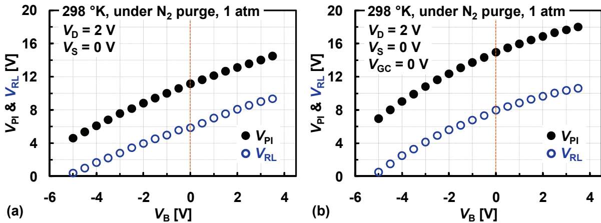
Figure 5.7: Measured V_{PI} and V_{RL} with changes in body-bias voltages. (a) Both gate electrodes were swept. (b) The gate electrode ( V_{GE} ) was swept.
