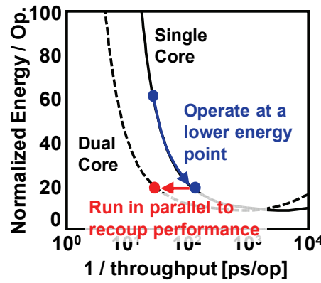
Figure 1.4: A single-core microprocessor that runs at a lower clock speed can be made to operate at lower energy per operation. Two single-core processors can be run in parallel to recoup the overall system performance.
