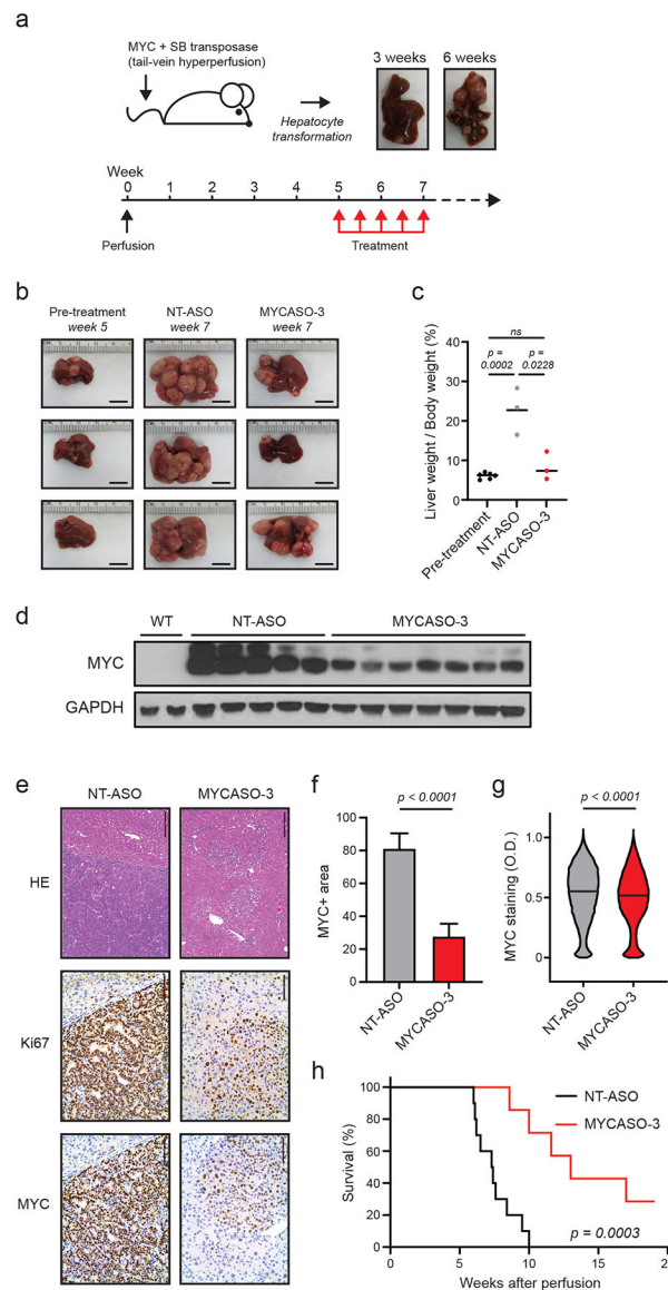
Figure 6: In vivo effects of MYCASO-3 in a MYC-induced model of hepatocellular carcinoma. (a) Schematic of HCC tumor model used to assess MYCASO-3 effects. A plasmid expressing human MYC is co-injected with a plasmid expressing the Sleeping Beauty transposase by hydrodynamic injection. Liver tumor formation is observed by three weeks following perfusion, with large tumor masses observable by 6 weeks. MYCASO-3 was dosed at 25 mg/kg in mice beginning 5 weeks after perfusion, and dosing was performed every 3 days for a period of 2 weeks (a total of 5 doses). (b) Example harvested livers from pre-treatment (5 weeks after perfusion; n=6), NT-ASO treated (7 weeks after perfusion; n=3), and MYCASO-3 treated mice (7 weeks after perfusion; n=3). (c) Ratios of liver weight to body weight in pre-treatment (n=5), NT-ASO treated (n=3), and MYCASO-3 treated mice (n = 3). Bars represent mean values. Statistical analysis performed by t test. (d) MYC immunoblotting on extracts from wild-type (WT) liver tissue, tumor tissue from NT-ASO treated mice, and tumor tissue from MYCASO-3 treated mice. (e) HE
