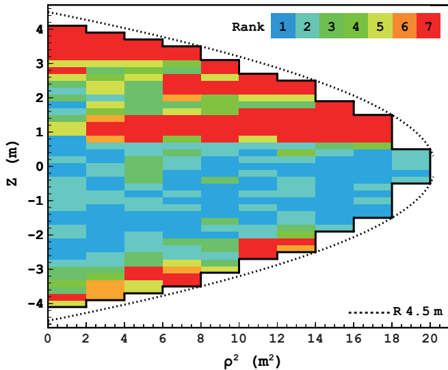
FIG. 2: Rank classification of partitions in the fiducial volume during a short data taking interval.
