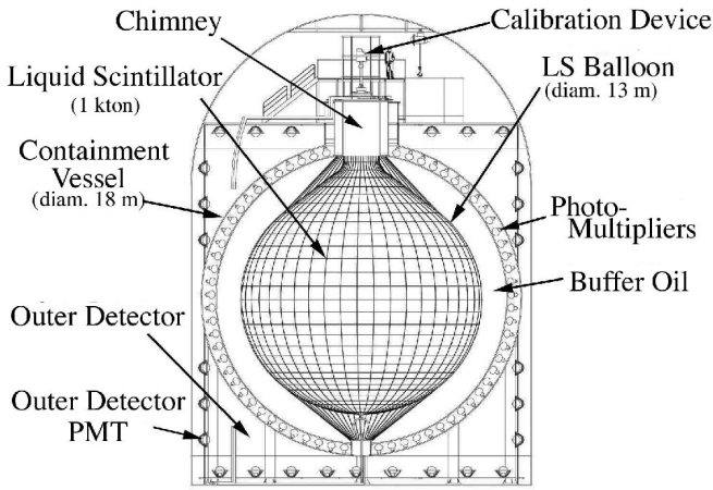
FIG. 1: Schematic diagram of the KamLAND detector.
