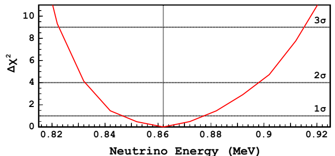
FIG. 5: \Delta\chi^2 -profile from the fit to the energy of mono-energetic neutrinos discussed in the text. The vertical line indicates the neutrino energy predicted from the {}^7\text{Be} electron-capture reaction at 862 \text{ keV} .
