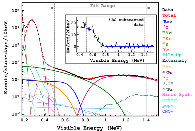
FIG. 4: Energy spectrum of selected {}^7\text{Be} solar neutrino candidates for the rank-1 data-set together with the best-fit curves from the simultaneous fit to all rank's spectra. The fit range is 0.5 \text{ MeV} < E < 1.4 \text{ MeV} . The background-subtracted spectrum is shown in the inset, where a Compton-like shoulder characteristic for the {}^7\text{Be} solar neutrino contribution is evident. The error bars are statistical only and do not include correlated systematic uncertainties in the background rate estimates.
