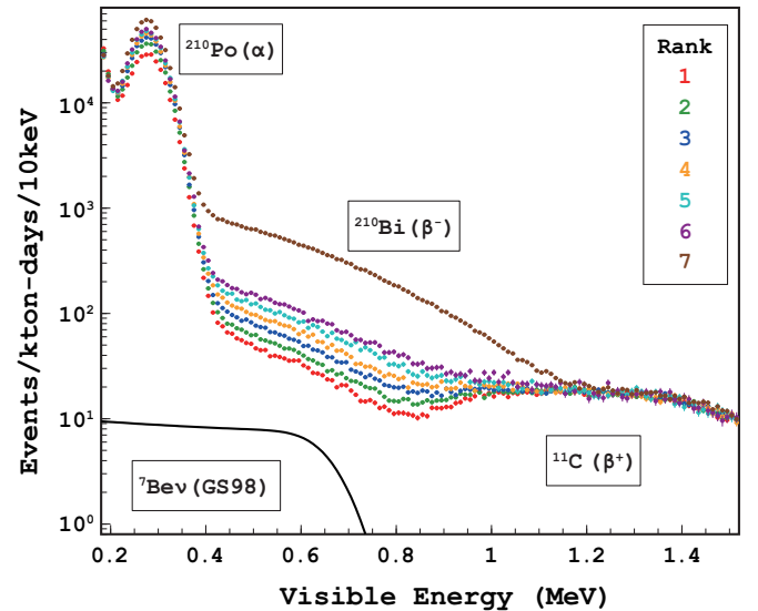
FIG. 3: Energy spectra of candidate events for each data-set rank, exhibiting different ^{210}\text{Bi} rates. All data sets are used for the simultaneous fit of the ^7\text{Be} solar neutrino spectrum, with a common rate normalization. The location of the major background sources are labeled and the theoretical electron recoil spectrum of 862 keV ^7\text{Be} solar neutrinos, whose rate is based on the standard solar model by Serenelli et al. [15] is shown for comparison.
