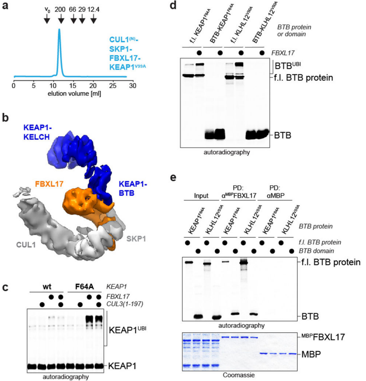
Extended Data Figure 3: SCF FBXL17 binds the BTB domain, but its active site is next to the Kelch repeats of KEAP1.
