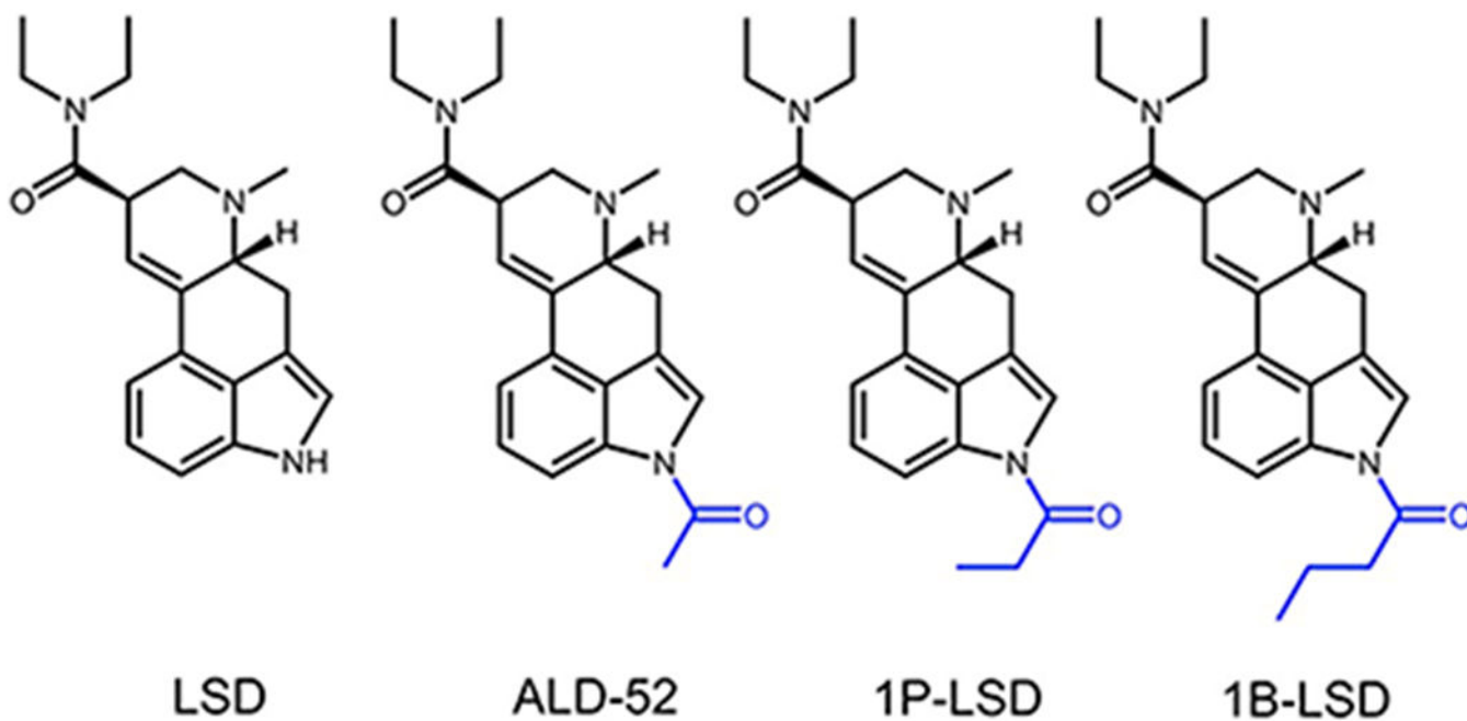
Fig. 1. Chemical structures of LSD and N^1 -substituted derivatives. Structural changes in comparison to LSD are indicated in blue.
