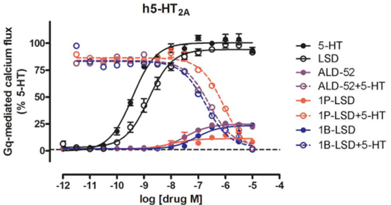
Fig. 2. Agonist and antagonist potencies of N 1 -substituted LSD derivatives at the human 5-HT 2A (h5-HT 2A ) receptor. Receptor activation was assessed using Ca 2+ mobilization. Concentration-response curves are shown for 5-HT, LSD, ALD-52, 1P-LSD, and 1B-LSD. Antagonist assays were performed in the presence of 3 nM 5-HT. Values are the mean ± SEM of between three and five independent experiments performed in triplicate.
