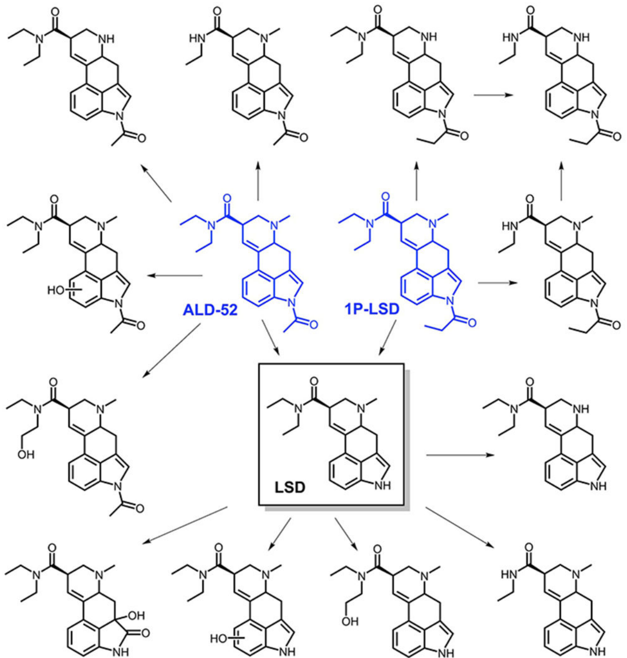
Fig. 4. Postulated metabolic pathways for ALD-52 and 1P-LSD after subcutaneous administration to Sprague-Dawley rats. As indicated in the diagram, both ALD-52 and 1P-LSD are metabolized to LSD.
