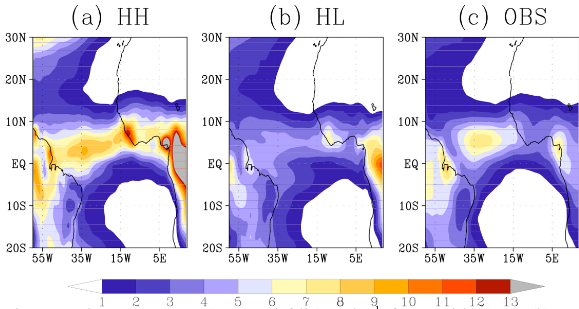
Figure 5.9 Six-year (1999-2004) mean rainfall ( \text{mm day}^{-1} ) from model; (a) HH, (b) HL, and (c) the observations from the Global Precipitation Climatology Project (GPCP). The model precipitation in (a) and (b) is re-gridded to the GPCP grids at 2.5^\circ \times 2.5^\circ . Precipitation greater than 13 \text{ mm day}^{-1} is shaded in gray.
