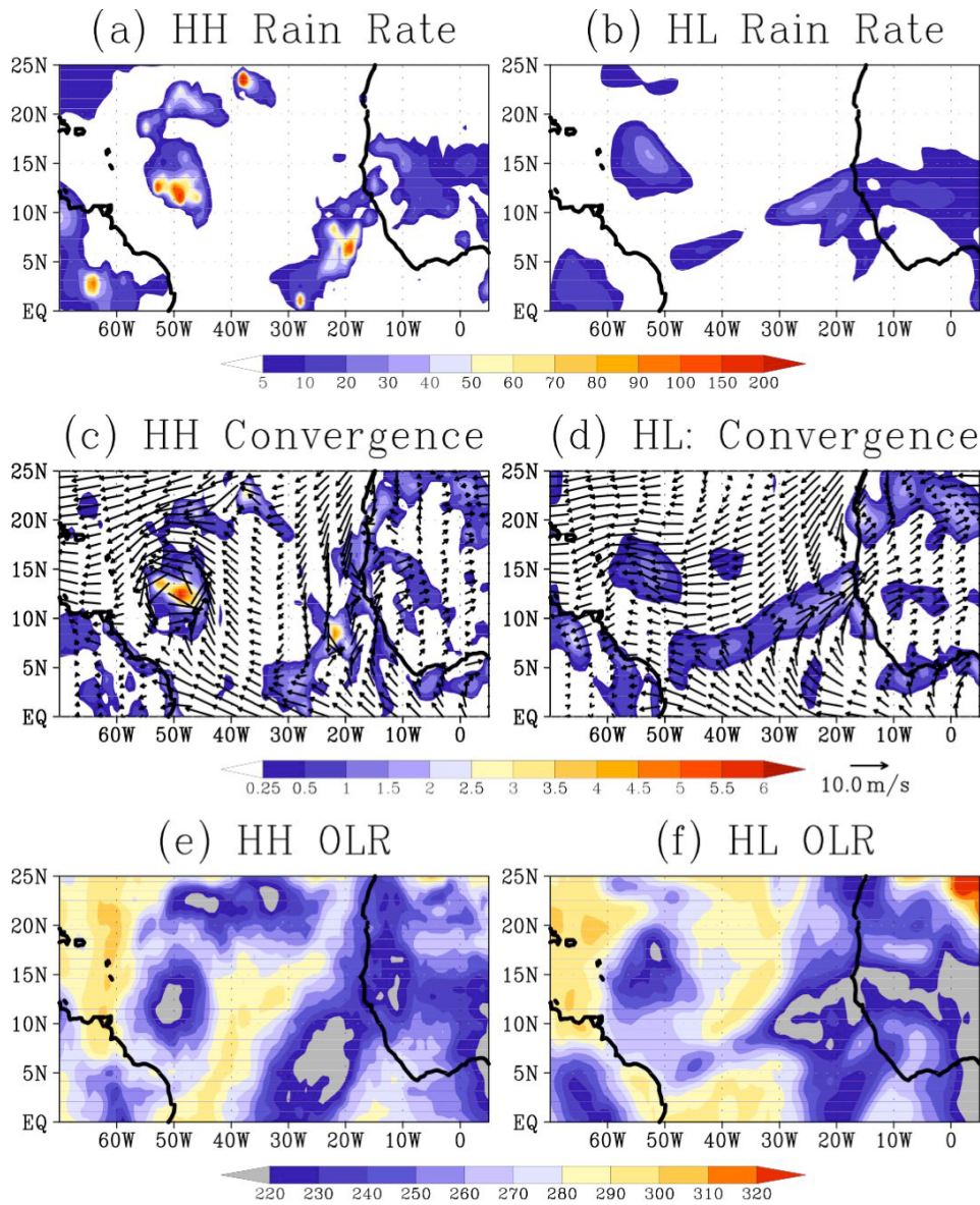
Figure 5.5 Two-day averages (August 31 – September 1, 2003) of (top) rainfall (mm day -1 ), (middle) near-surface convergence (10 -5 s -1 ) of 10 m winds and the wind vectors (m s -1 ), and (bottom) outgoing longwave radiation (OLR, W m -2 ) from (left) HH and (right) HL. Only convergence is plotted in (c) and (d) for clarity. OLR less than 220 W m -2 in (e) and (f) is plotted in gray and represents strong atmospheric convection.
