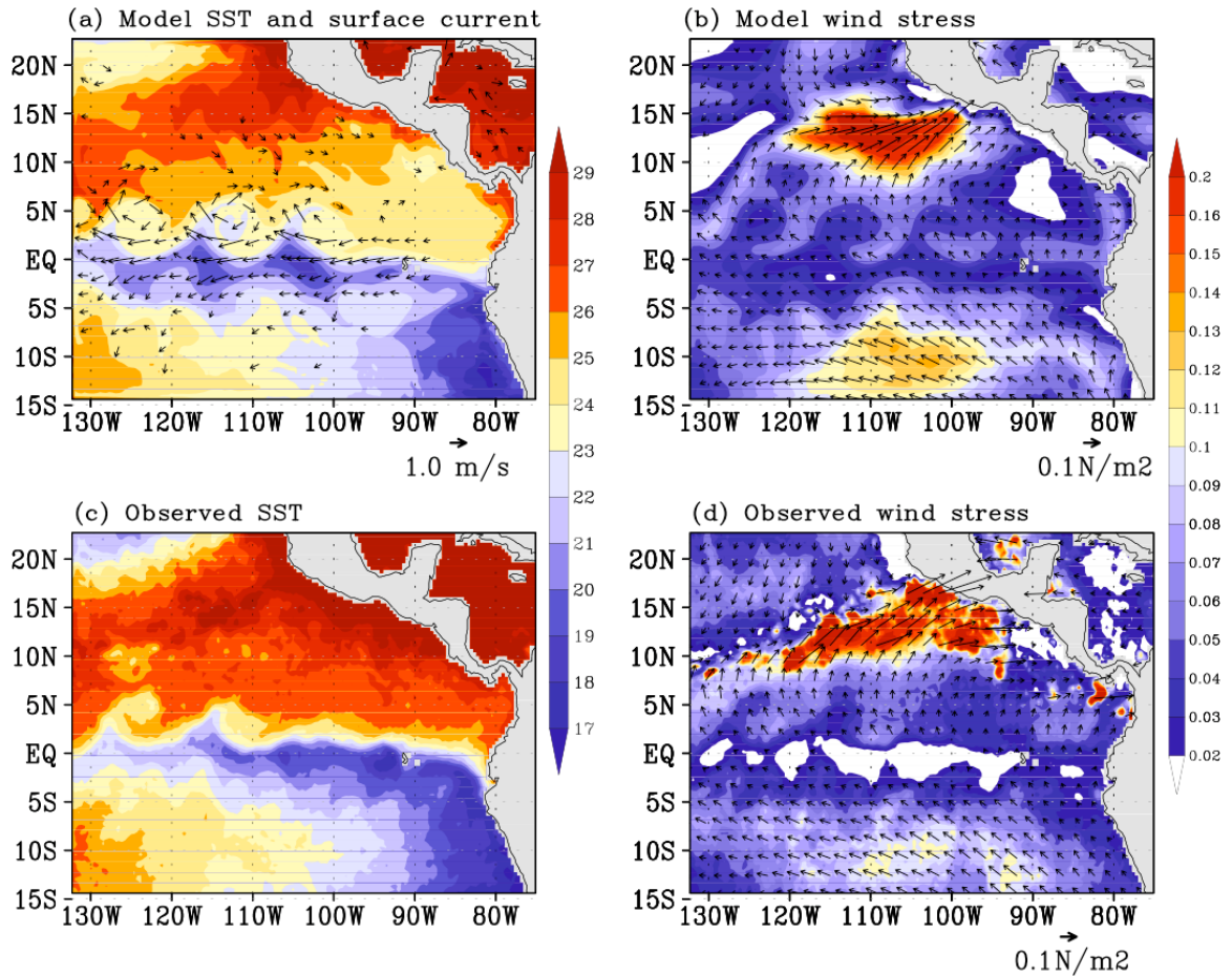
Figure 2.3 Three-day averaged oceanic and atmospheric states centered on September 3, 1999 from (upper panel) the model simulations, and (bottom panel) from the observations. (a) SST ( ^{\circ}C ) and ocean surface currents ( m\ s^{-1} ), (b) wind stress ( WS ) vector and magnitude ( N\ m^{-2} ). (c) SST ( ^{\circ}C ) from TMI, and (d) wind stress vectors and magnitude from the QuikSCAT. Surface current speed less than 0.4\ m\ s^{-1} is not plotted in (a). Wind stress magnitude less than 0.02\ N\ m^{-2} is not plotted in (b) and (d).
