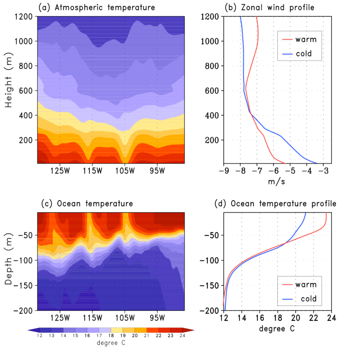
Figure 2.9 (left) Longitude-height (depth) cross-sections of (a) atmospheric temperature (°C) and (c) ocean temperature (°C) from 2-4 September 1999 averaged from 1°N-2°N. (right) The composite profiles of (b) zonal wind ( \text{m s}^{-1} ) and (d) vertical ocean temperature (°C). Red (blue) lines are mean profiles when zonal deviation of SST is warmer (colder) than 1 standard deviation. There were 17 (15) warm (cold) phases from 2-4 September 1999.
