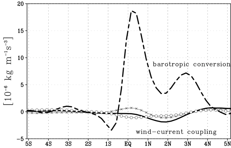
Figure 3.7 Zonal average ( 30^{\circ}\text{W} - 10^{\circ}\text{W} ) of 6-year model mean (dashed line) barotropic conversion rate of the zonal flow, -\rho_o(u'v'U_y) averaged over 150 m, i.e., \frac{1}{d} \int_d^{sfc} (-\rho_o u'v'U_y) dz , where d is the depth of the center of EUC (150 m). (Solid line) Time and zonal mean \bar{u}'_{sfc} \cdot \bar{\tau}'_z averaged over 150 m, i.e., \frac{1}{d} \int_d^{sfc} (\bar{u}'_{sfc} \cdot \bar{\tau}'_z) dz . Zonal (meridional) component of \frac{1}{d} \int_d^{sfc} (\bar{u}'_{sfc} \cdot \bar{\tau}'_z) dz is shown by the light solid line with x (o).
