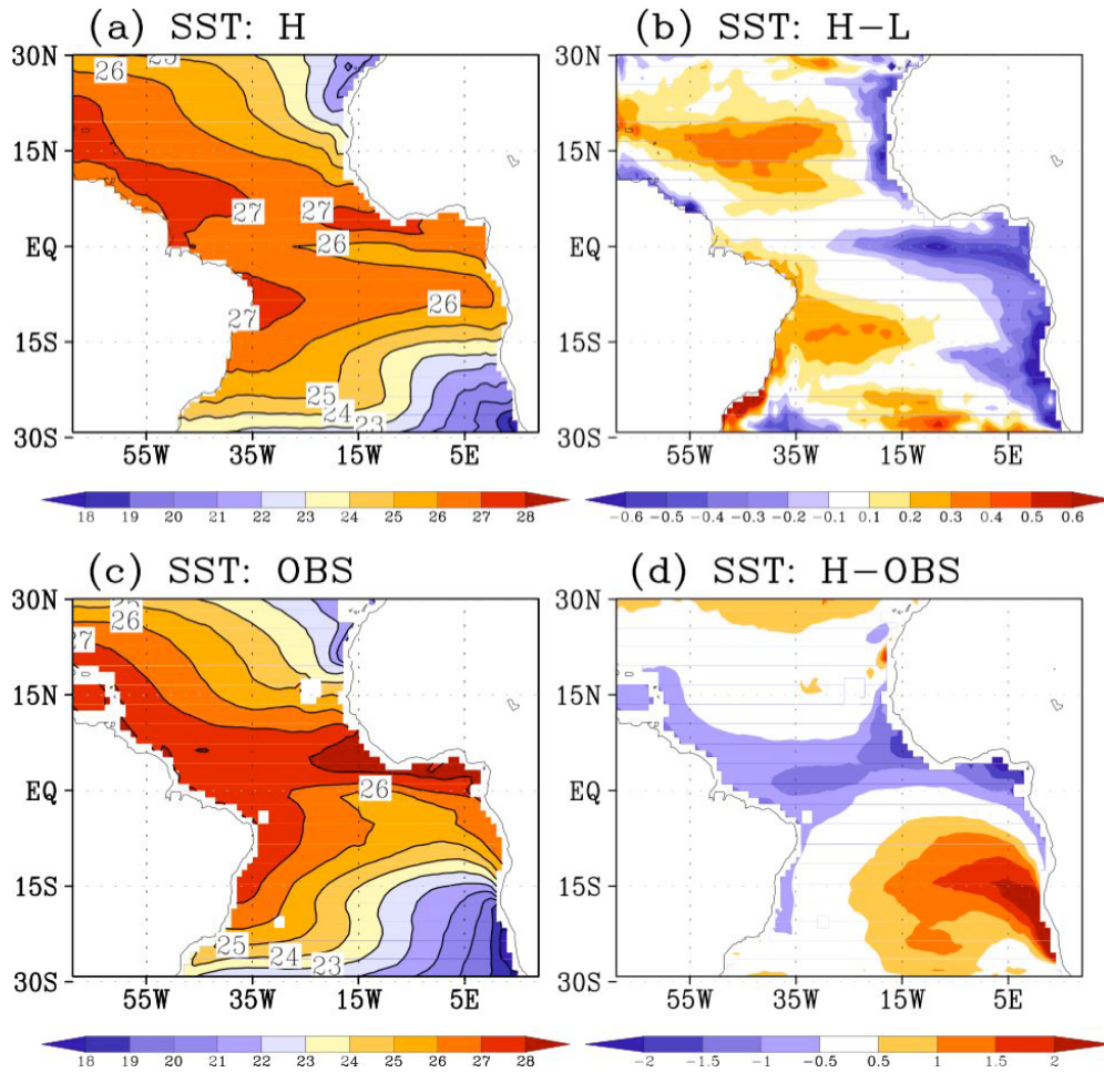
Figure 4.1. Mean SST (°C) from 1999 to 2004, (a) H, (b) H-L, and (c) observed SST from Tropical Rainfall Measuring Mission Microwave Image (TMI) (OBS), and (d) H-OBS. H SST is colder by up to 0.6°C in the equatorial cold tongue and African coastal upwelling region, while warmer in the extratropics.
