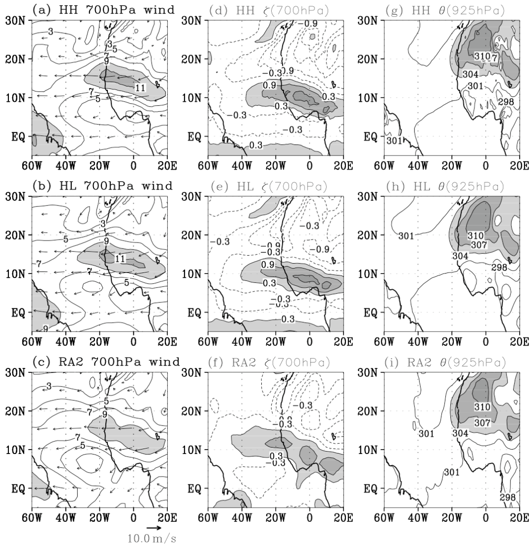
Figure 5.1 Six-year summertime (July-August-September) mean (a-c) wind speeds and vectors at 700 hPa (shaded when greater than 9 m s -1 ), (d-f) 700 hPa relative vorticity (shaded when greater than 0.3 s -1 ), and (g-i) 925 hPa potential temperature (shaded when greater than 304K). (top) HH, (middle) HL, and (bottom) NCEP/DOE Reanalysis II (RA2). HH in the top panel and RA2 in the bottom panel are interpolated to the grids on HL.
