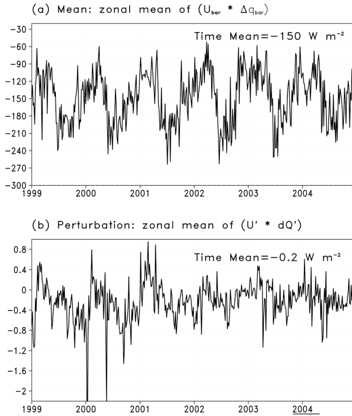
Figure 3.11 Six-year time series of (a) \rho LC_H \overline{U \Delta q} and (b) \rho LC_H \overline{U' \Delta q'} at 2^\circ\text{N} averaged over 30^\circ\text{W} - 10^\circ\text{W} in the model. Similar results are found for different areas.
