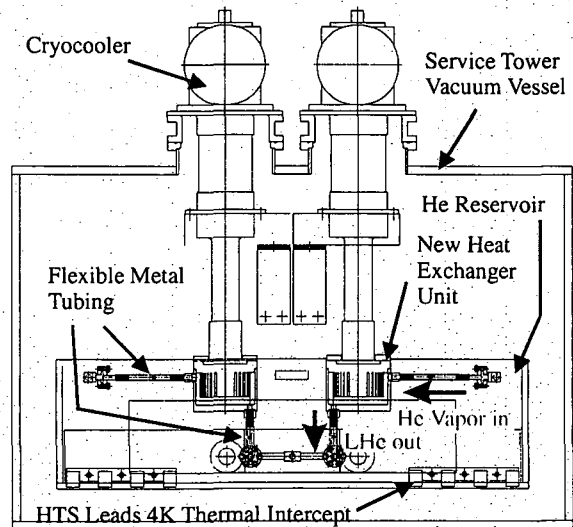
Figure 5 Side and front view of the new heat exchanger concept for the VENUS cryostat. In this design, the helium vapour transports the heat directly to the cryocoolers.
