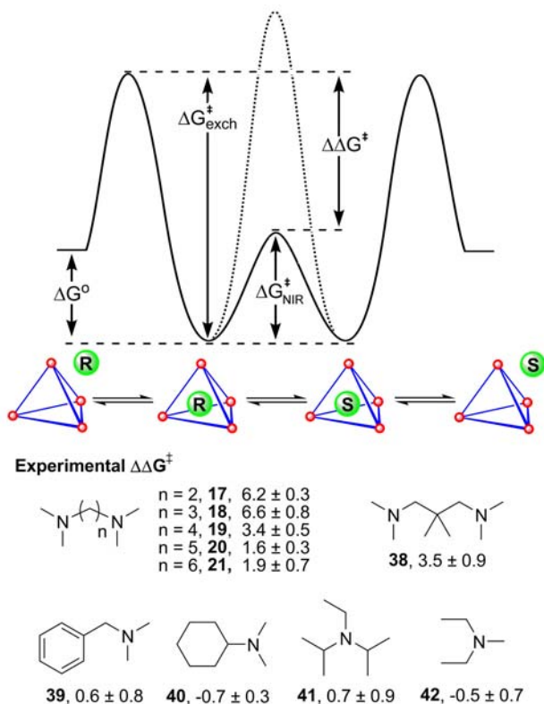
Figure 4. Top: Energy diagram for amine exchange and inversion in 1 . Solid line: \Delta G_{\text{NIR}}^\ddagger < \Delta G_{\text{exch}}^\ddagger , Dotted line: \Delta G_{\text{exch}}^\ddagger < \Delta G_{\text{NIR}}^\ddagger . Bottom: \Delta\Delta G^\ddagger values (kcal/mol) of the investigated amines. 28
