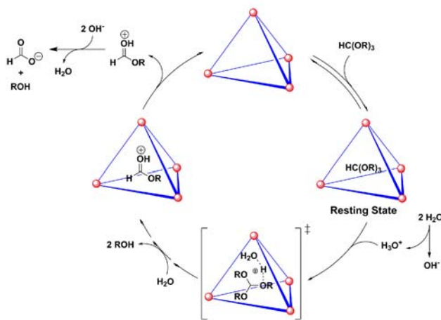
Figure 8. Proposed mechanism for catalytic hydrolysis of orthoformates in 1 . 42
