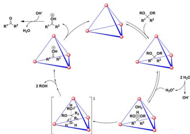
Figure 12. Proposed mechanism for acetal hydrolysis in 1 . 46
