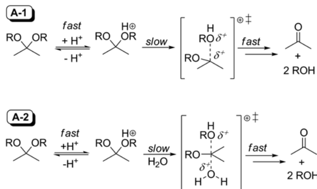
Figure 11. Comparison of A-1 and A-2 mechanisms for acetal hydrolysis. Hydrolysis of 56 proceeds through an A-1 mechanism in free solution but an A-2 mechanism in 1 .
