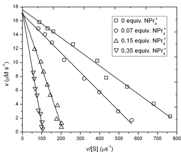
Figure 9. Eadie-Hofstee plot showing competitive inhibition by \text{NPr}_4^+ for the hydrolysis of 53 in 1 . 41
