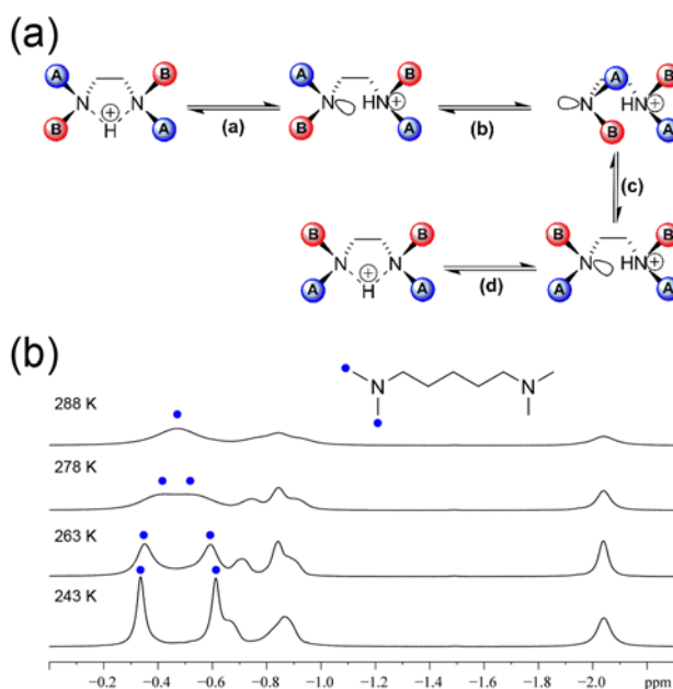
Figure 3. Top: Schematic for the NIR process resulting in the interchange of the geminal N -methyl groups. Bottom: Variable temperature ^1\text{H} NMR showing coalescence of the geminal N -methyl groups. 28
