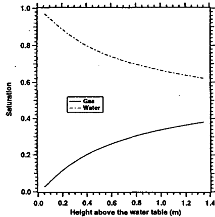
Fig. 1. Water and gas saturation in the two-phase layer in Zone #1.
