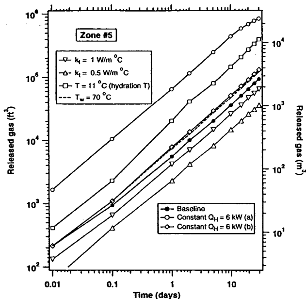
Fig. 12. Sensitivity of gas production to thermal conductivity k_f , hydrate temperature T , method of heat addition, and well boundary conditions.
