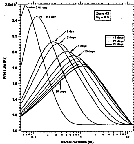
Fig. 7. Formation pressure during thermal dissociation of hydrates in Zone #3.
