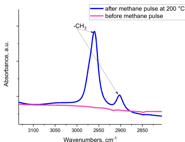
Figure 6. FTIR spectra showing the C-H stretching region of dehydroxylated gamma alumina before and after methane exposure (~0.5 Torr total pressure of methane) at 200 °C. The bands that developed correspond to two IR active vibrations of a methyl group.
