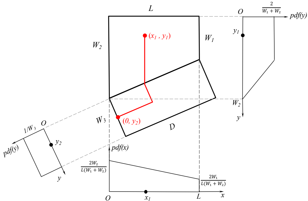
Figure 5.2 The Manhattan distance between two random dots in region S_1 and on edge W_3
