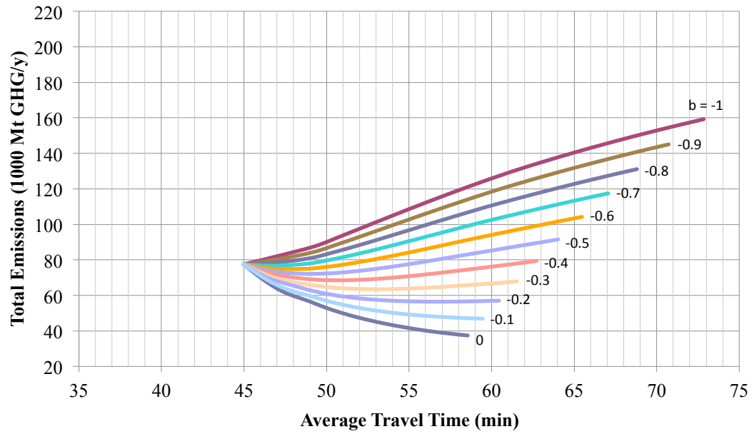
Figure 4.6 Change in total emissions with travel time as LOS is reduced for bus (scenario 2)
