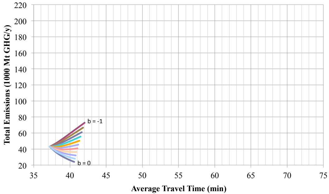
Figure 4.5 Change in total emissions with travel time as LOS is reduced for bus with no feeder access (scenario 2)
