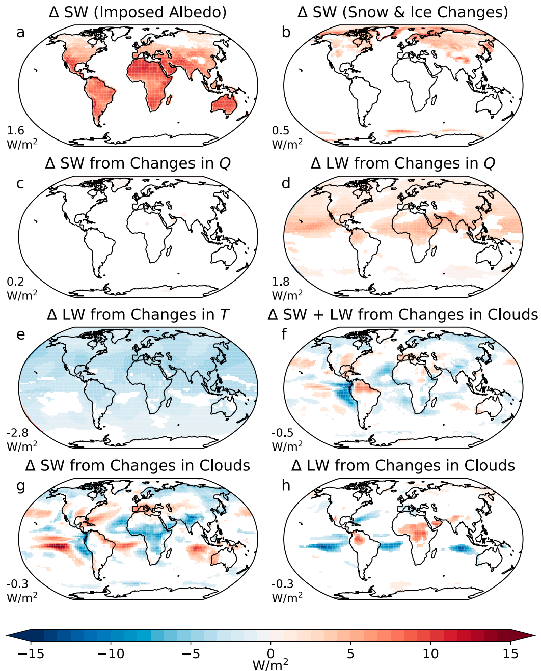
FIG. 4. Change in annual mean net top of atmosphere energy fluxes ( \text{W m}^{-2} ) as a result of decreasing land surface albedo. All fluxes (SW and LW) are shown positive down such that red colors indicate more energy absorbed by the Earth system, while blue colors indicate more energy lost by the Earth system. (a) Change in TOA net SW radiation from the imposed change in albedo. (b) Change in TOA net SW radiation from albedo changes due to changes in snow and ice. (c),(d) Changes in TOA SW and LW radiation, respectively, from changes in column water vapor. (e) Change in TOA LW from combined changes in the surface radiative temperature and changes in air temperature. (f) Total change in TOA SW + LW from changes in cloud cover. (g),(h) The effect of cloud cover separated into its impact on TOA SW and TOA LW, respectively. The area-weighted global mean value for each term is shown to the lower left of each map. Only values that differ with p < 0.05 in a Student's t test are shown.
